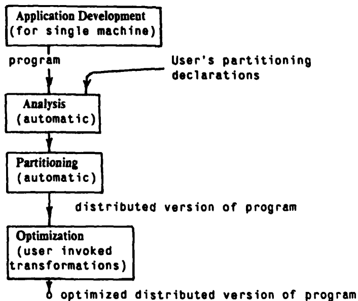
Figure 11-1: Development activities
