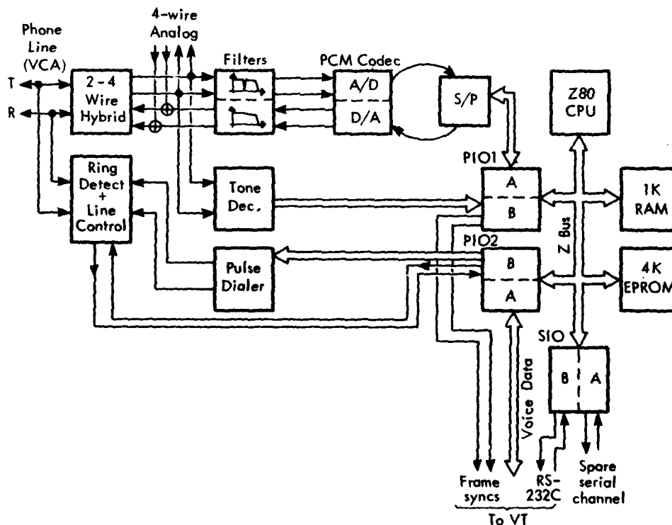
Figure 8-1: ISI STN interface
