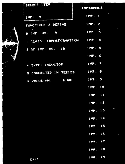
Plate 31 Function 2 DEFINE. Impedance definition menu for fully defined impedance of class transformation, type inductor
