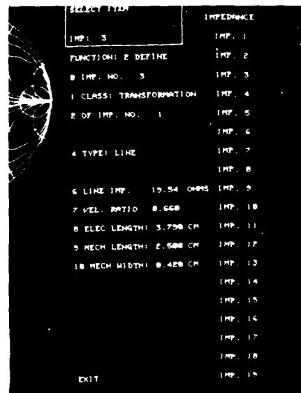
Plate 32 Function 2 DEFINE. Impedance definition menu for fully defined impedance of class transformation, type line
