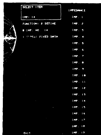
Plate 34 Function 2 DEFINE. Impedance definition menu for fully defined impedance of class fixed data
