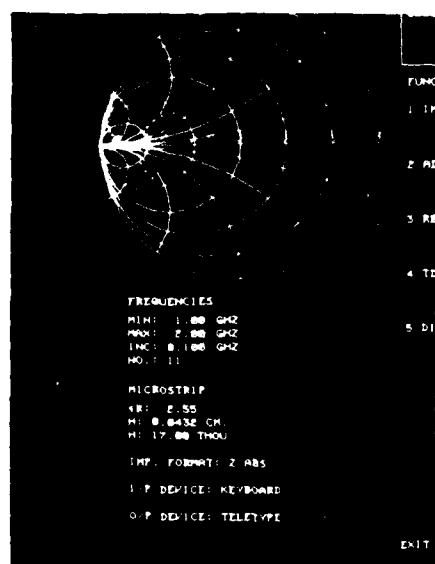
Plate 46 Admittance chart in display field
