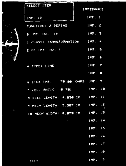
Plate 29 Function 2 DEFINE. Impedance definition menu after entering line electrical length
