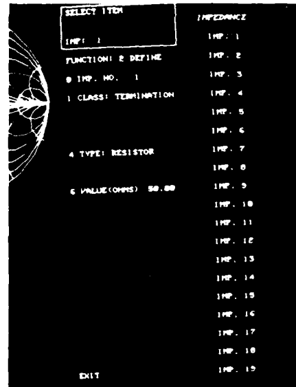
Plate 30 Function 2 DEFINE. Impedance definition menu for fully defined impedance of class termination
