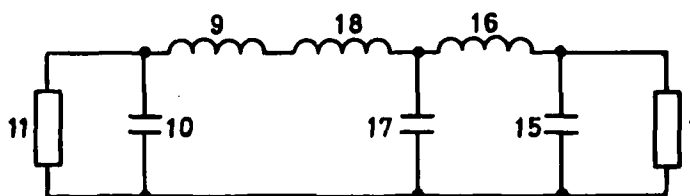
Fig 6 Lumped component matching network
