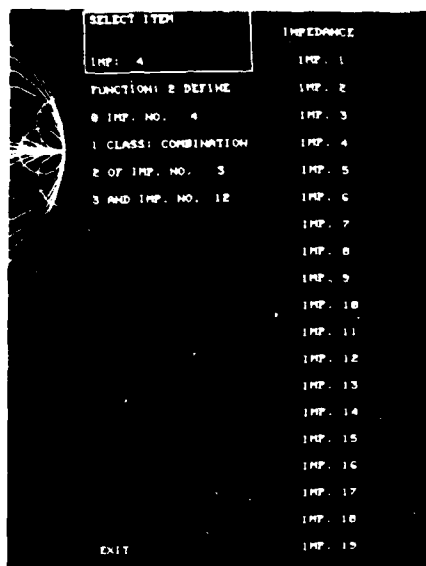
Plate 33 Function 2 DEFINE. Impedance definition menu for fully defined impedance of class combination
