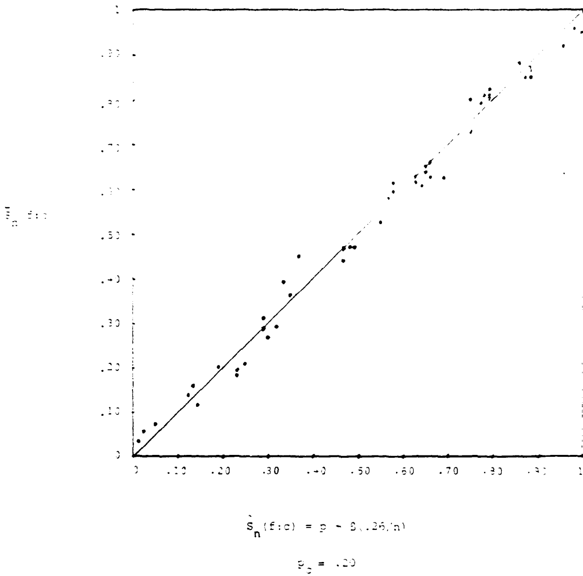
Figure 3: Actual vs. Predicted Net Strength for Aggregate Data
