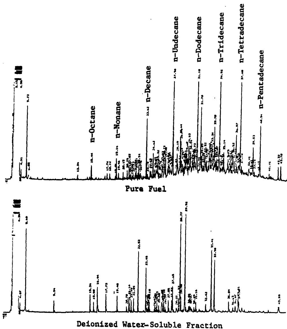
Figure 13. GC Traces of JP-8 in CS 2
