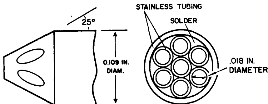
Figure 10. Probe Geometry
