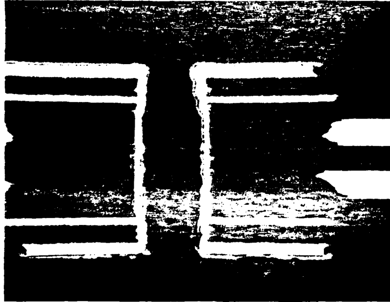
Figure 19. Plated-Through Hole Photomicrograph -- Visual Inspection
