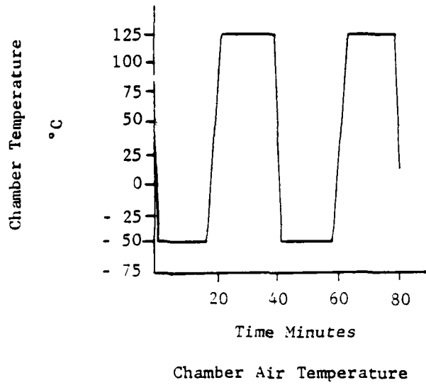
Figure A-7. Chamber Air Temperature
