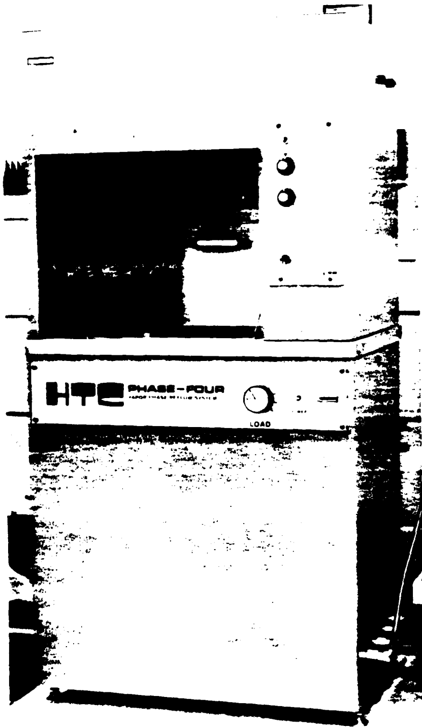
Figure 29. HTC Model 912 Vapor Phase Reflow Machine
