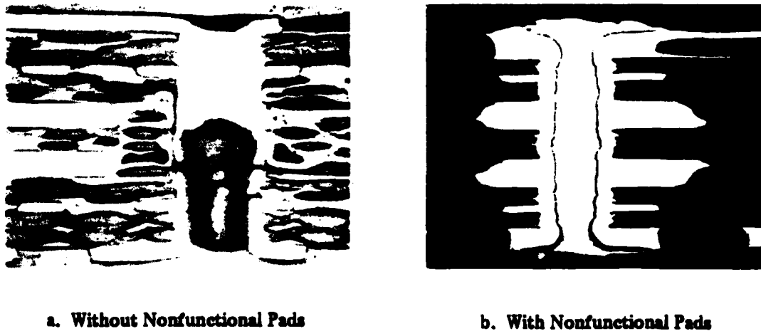
Figure 7. Failed Plated-Through Hole Microsection
