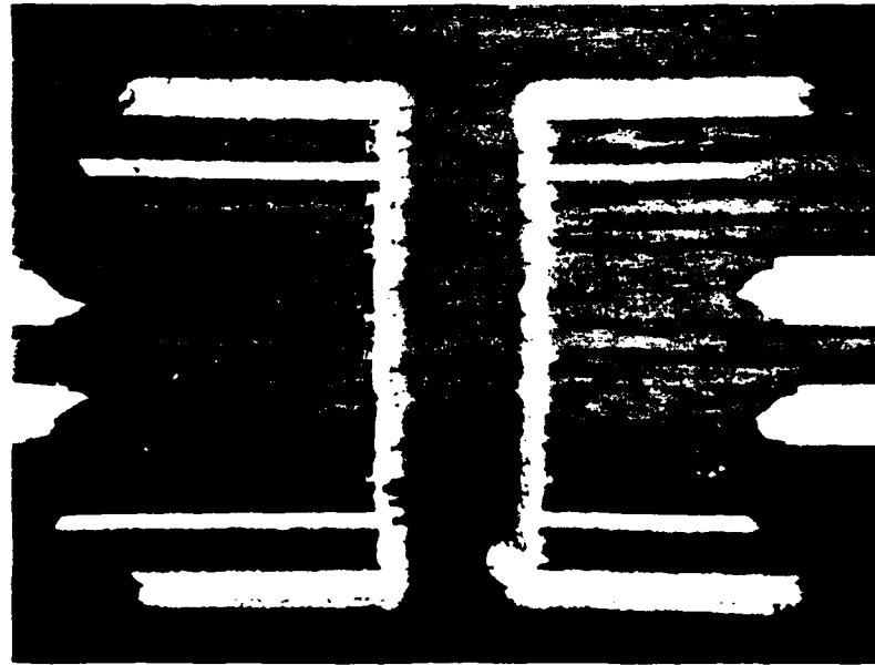
Figure 20. Plated-Through Hole Photomicrograph -- Dimensional Inspection
