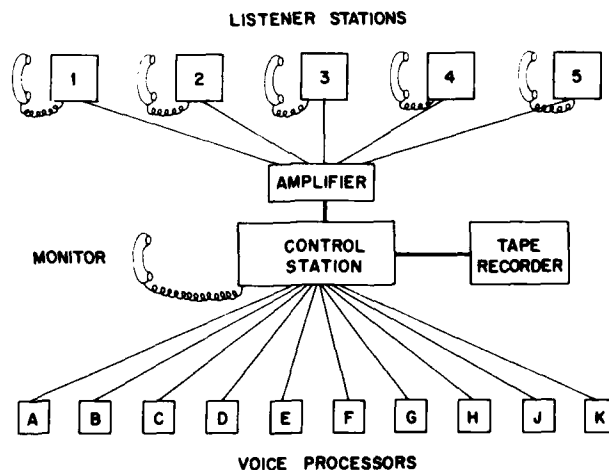
Fig. 1 — The NRL conversational test facility
