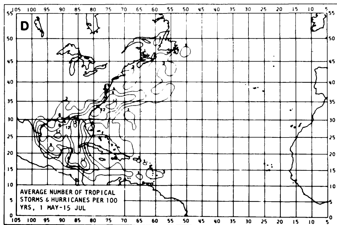
Figure 1-7 C,D. Early season storm frequency, 1 May-15 July. Note the small proportion of tropical cyclones reaching hurricane intensity.
