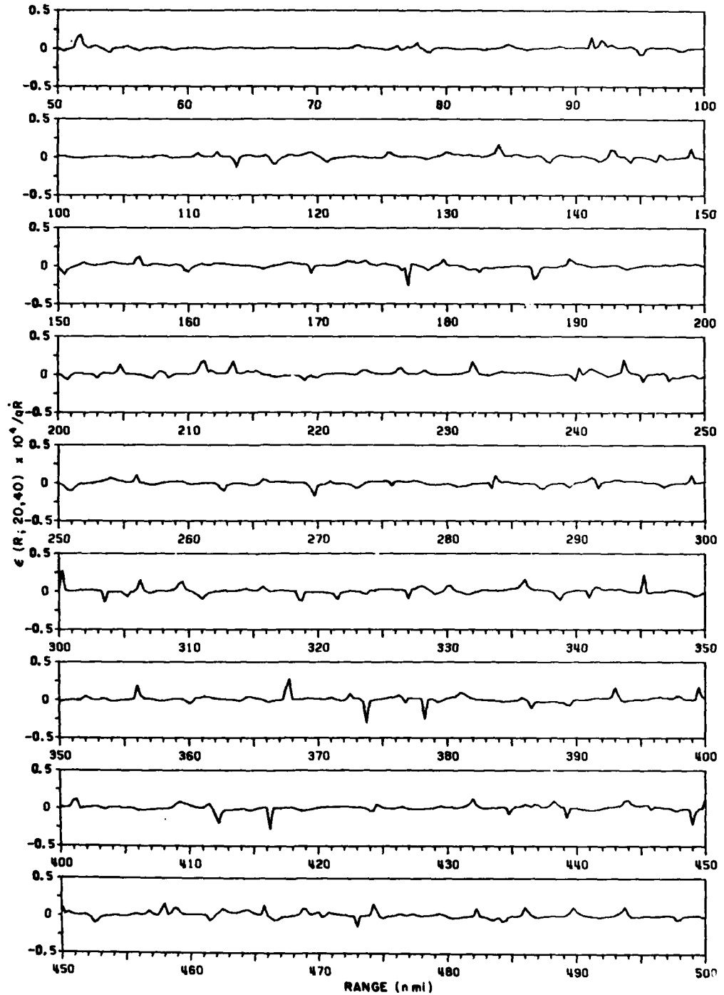
Fig. 36 — Dispersion measure \epsilon \times 10^4 / qR , over the range 50 to 500 nmi, between sinusoidal signals of 20 and 40 Hz. The measure of dispersion is the difference between the observed (or virtual) frequency ratio q' and the true frequency ratio q . R is the range rate in knots.
