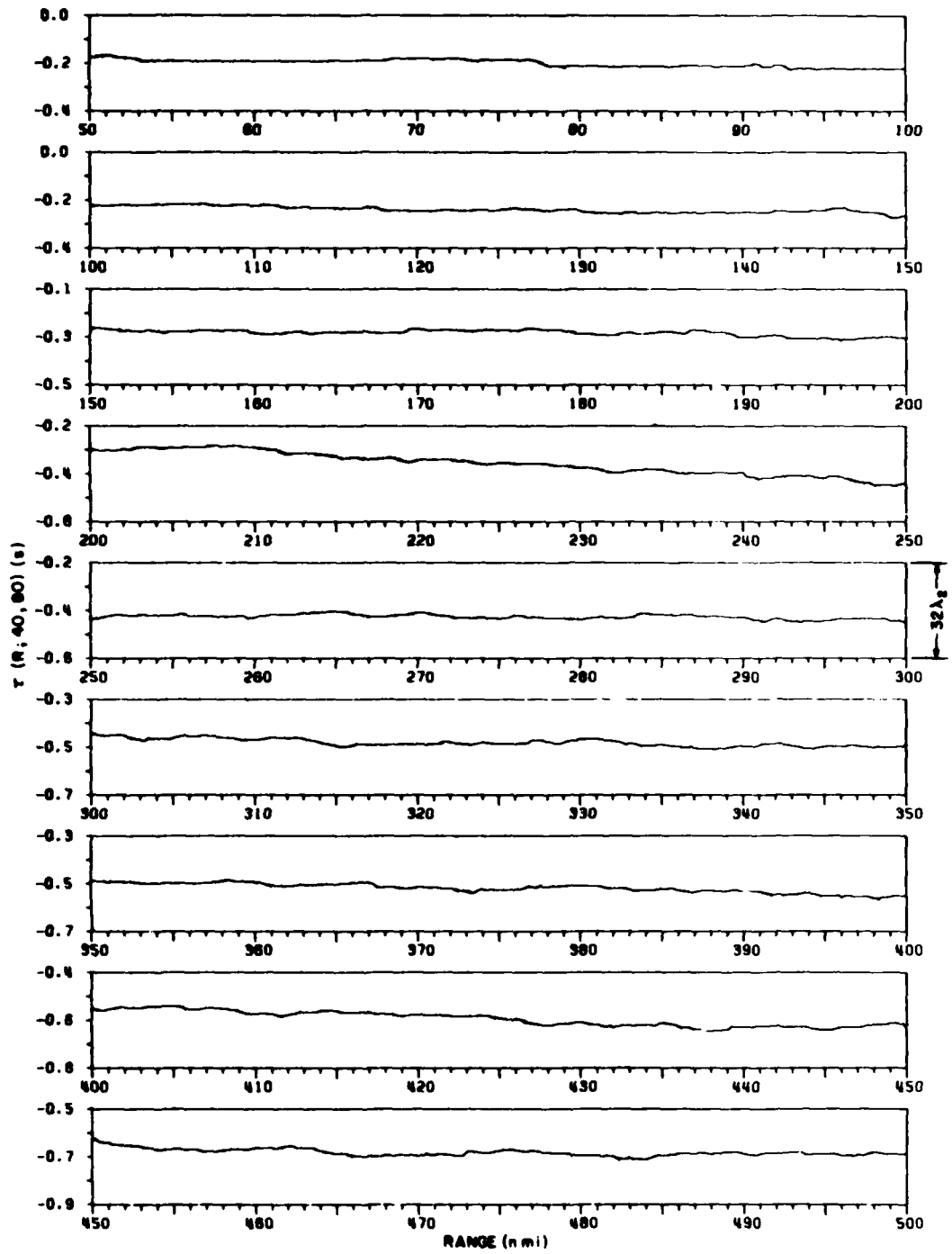
Fig. 25 — Difference in virtual propagation time, over the range 50 to 500 nmi, between sinusoidal signals of 40 and 80 Hz. The time scale, in wave periods of the upper frequency, is shown at the right of the center graph.
