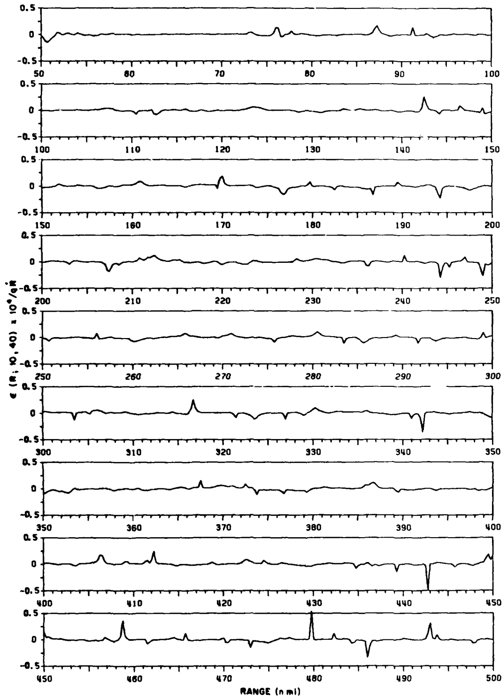
Fig. 31 — Dispersion measure \epsilon \times 10^4 / qR , over the range 50 to 500 nmi, between sinusoidal signals of 10 and 40 Hz. The measure of dispersion is the difference between the observed (or virtual) frequency ratio q' and the true frequency ratio q . R is the range rate in knots.
