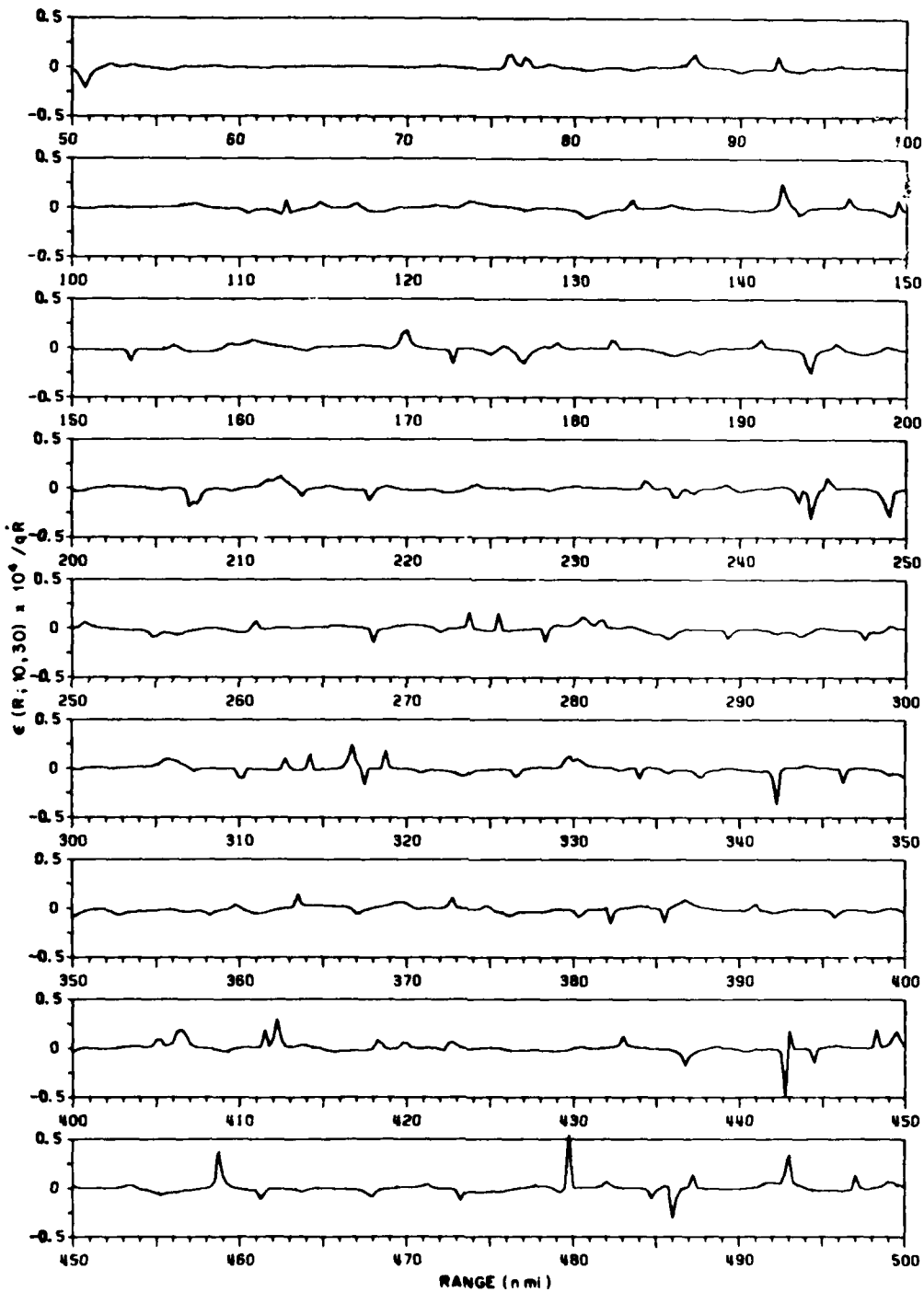
Fig. 29 — Dispersion measure \epsilon \times 10^4 / qR , over the range 50 to 500 nmi, between sinusoidal signals of 10 and 30 Hz. The measure of dispersion is the difference between the observed (or virtual) frequency ratio q' and the true frequency ratio q . R is the range rate in knots.
