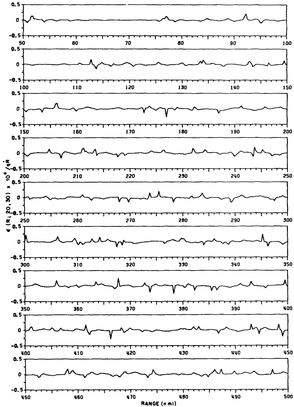
Fig. 33 — Dispersion measure \epsilon \times 10^4 / qR , over the range 50 to 500 nmi, between sinusoidal signals of 20 and 30 Hz. The measure of dispersion is the difference between the observed (or virtual) frequency ratio q' and the true frequency ratio q . R is the range rate in knots.
