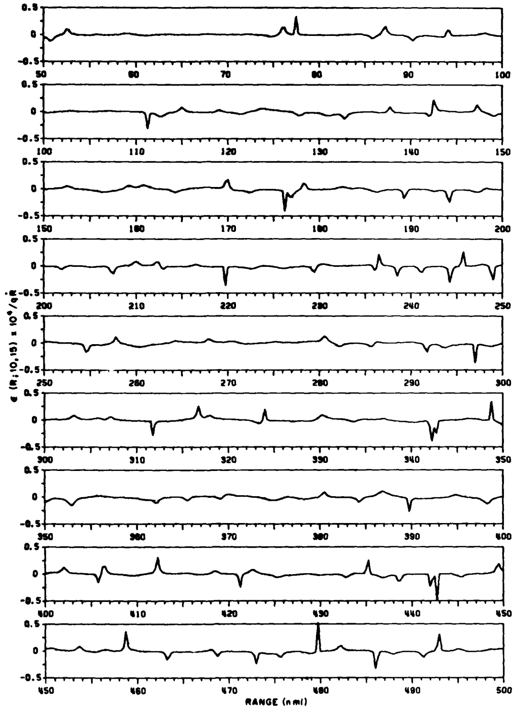
Fig. 26 — Dispersion measure \epsilon \times 10^6 / qR , over the range 50 to 500 nmi, between sinusoidal signals of 10 and 15 Hz. The measure of dispersion is the difference between the observed (or virtual) frequency ratio q' and the true frequency ratio q . R is the range rate in knots.
