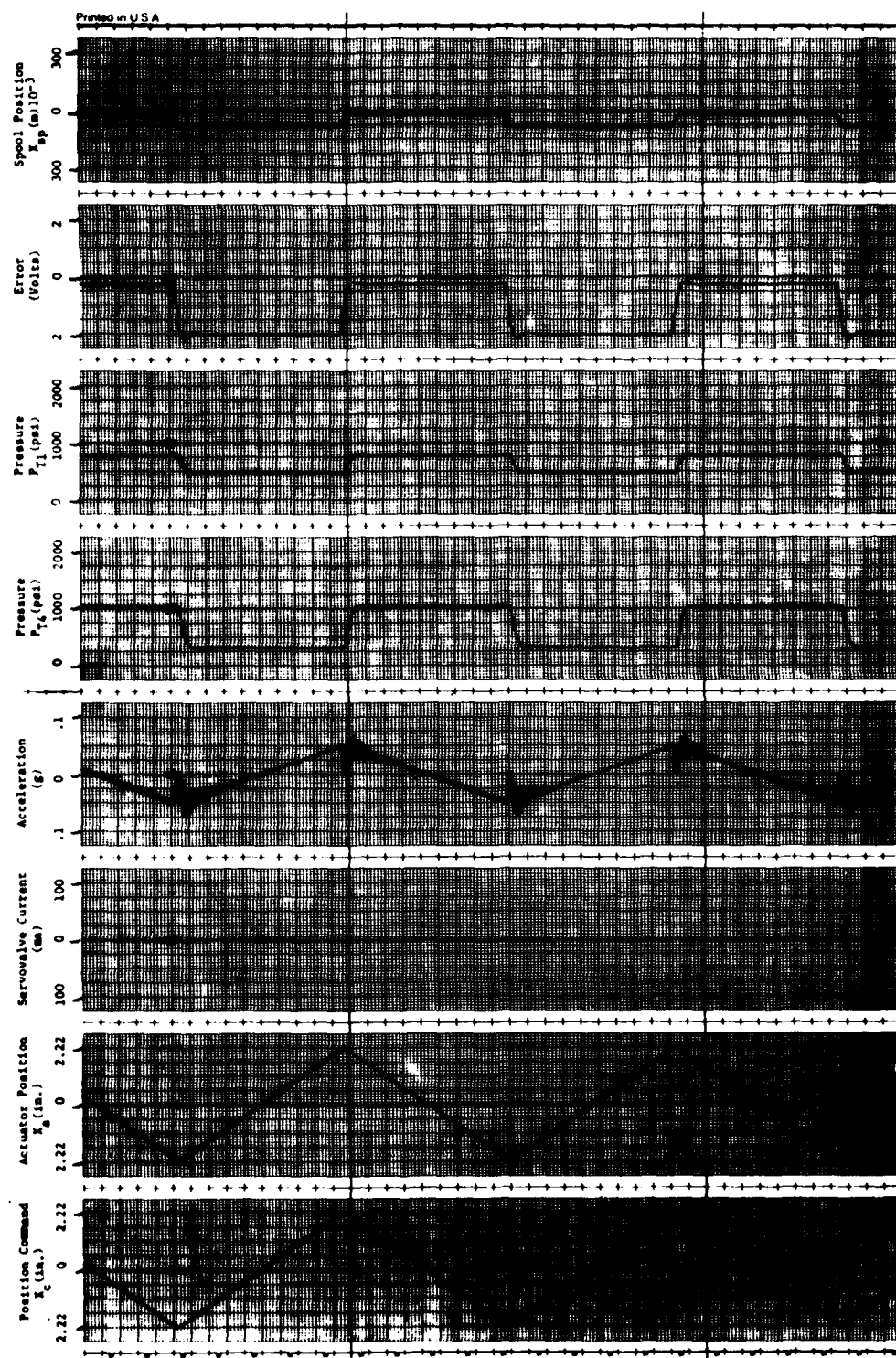
FIGURE: F-8 FREQUENCY: 0.10 WAVEFORM: TRIANGULAR
