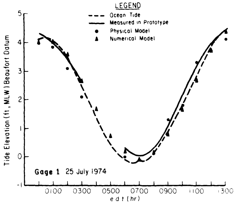
Figure A-1. Observed and predicted tides at gage 1.
