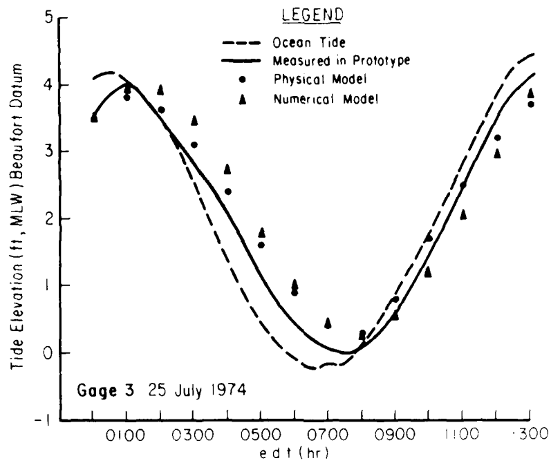
Figure A-3. Observed and predicted tides at gage 3.
