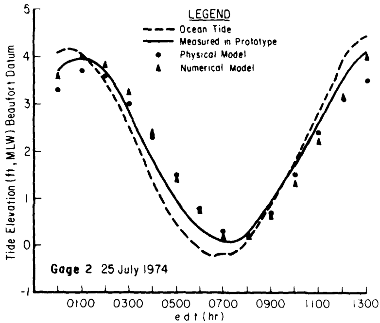
Figure A-2. Observed and predicted tides at gage 2.
