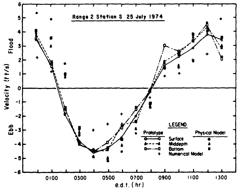
Figure A-12. Observed and predicted velocities at range 2, station S.
