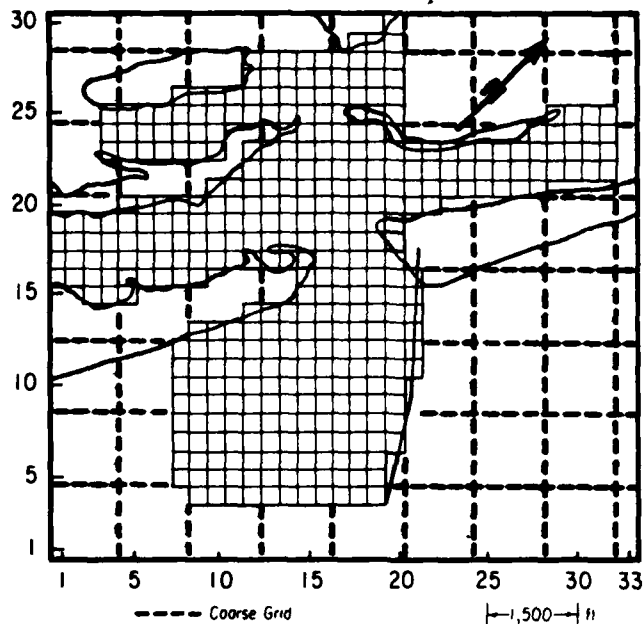
Figure 11. Fine grid configuration used to describe September 1969 conditions (Masch, Brandes, and Reagan, 1977).
