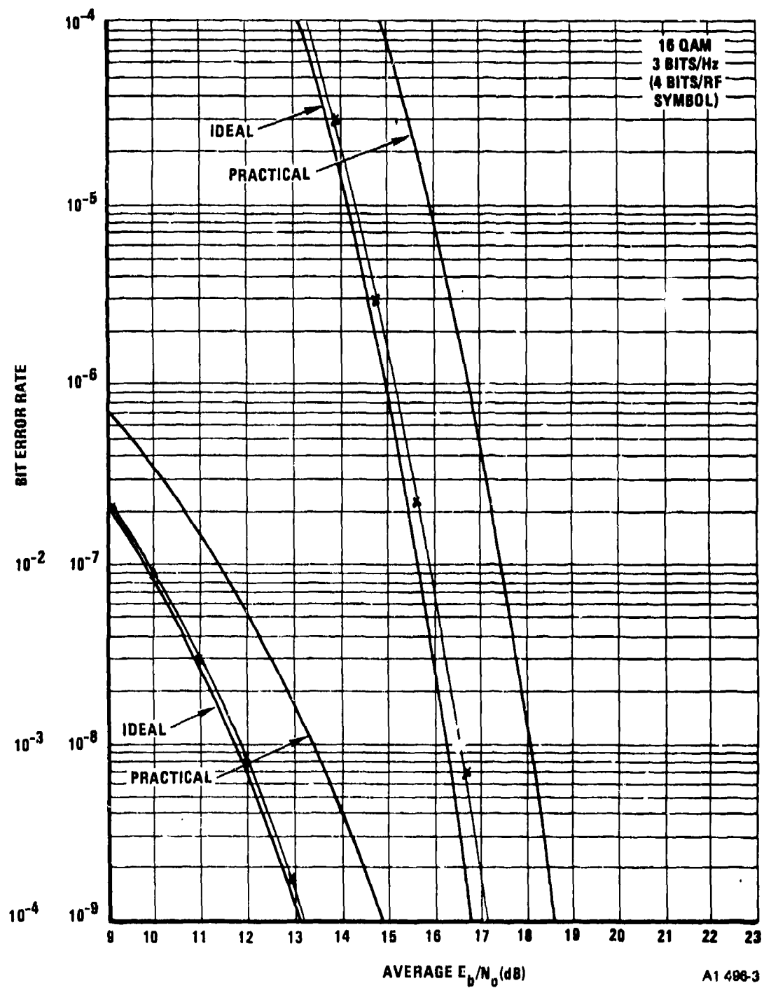
Figure 4.1.3.1-3. 16-QAM Back-to-Back Performance, No Filters
