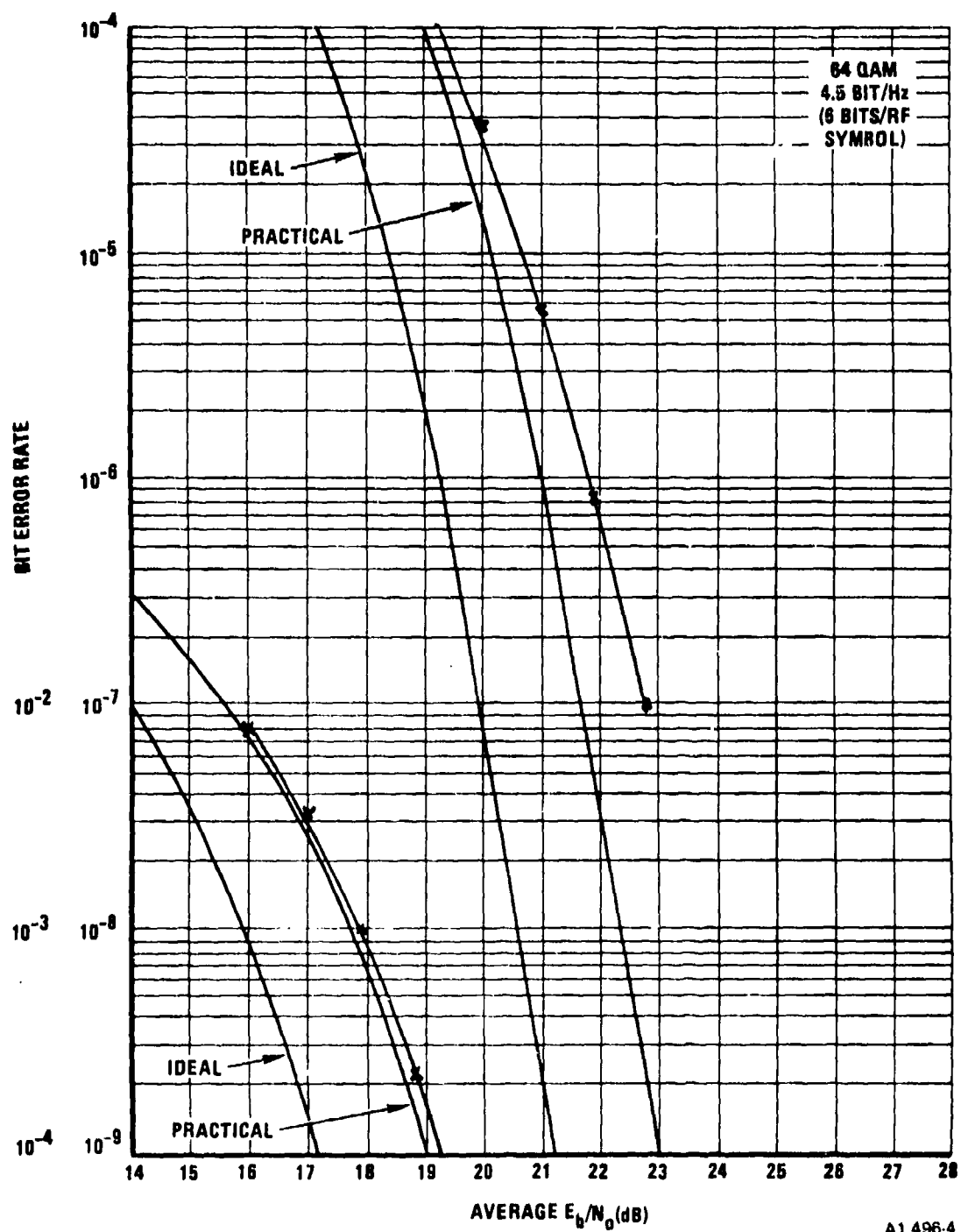
Figure 4.1.3.2-26. 64-QAM Back-to-Back Performance With Predistortion Enabled
