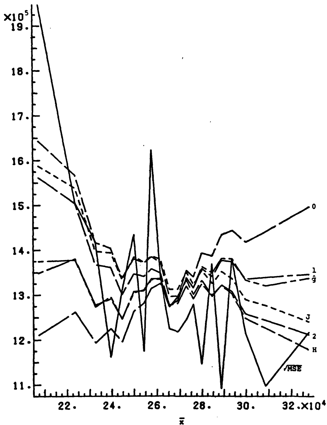
Figure 5. Curves \sqrt{MSE} , \sqrt{v_0} , \sqrt{v_1} , \sqrt{v_2} , \sqrt{v_g} , \sqrt{v_J} , \sqrt{v_H} for population (2).
