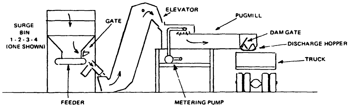
Figure 5. Continuous-mix plant—schematic operation.
