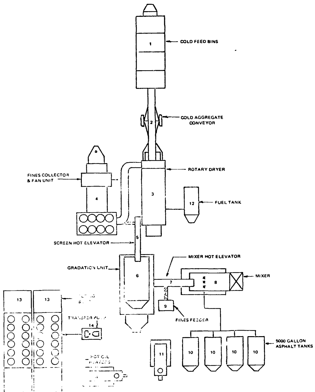
Figure 4. 150-ton/h asphalt mixing plant.
