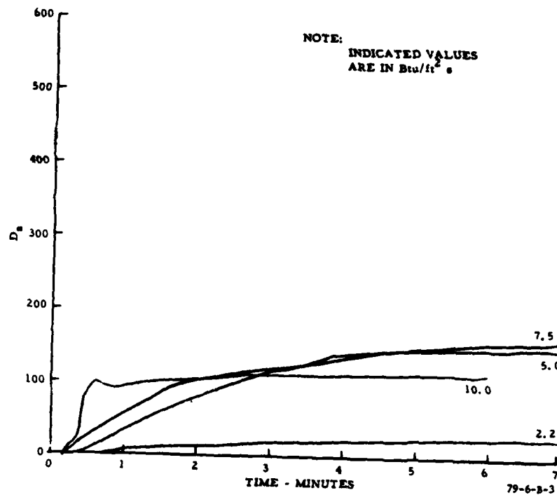
FIGURE B-3. FR TREATED NYLON (No. 209), NONPILOTED
