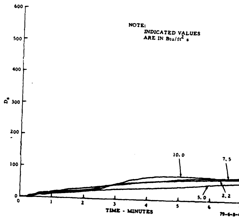
FIGURE B-4. FR TREATED NYLON (No. 209), PILOTED
