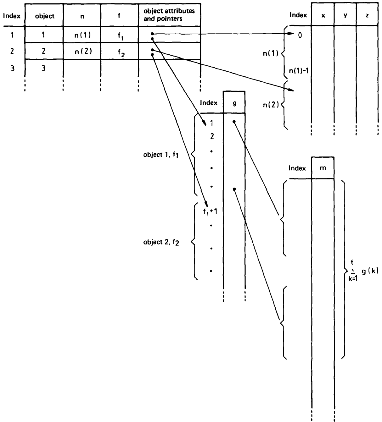
FIG. 2.4 SCENE DESCRIPTION DATA STRUCTURE
