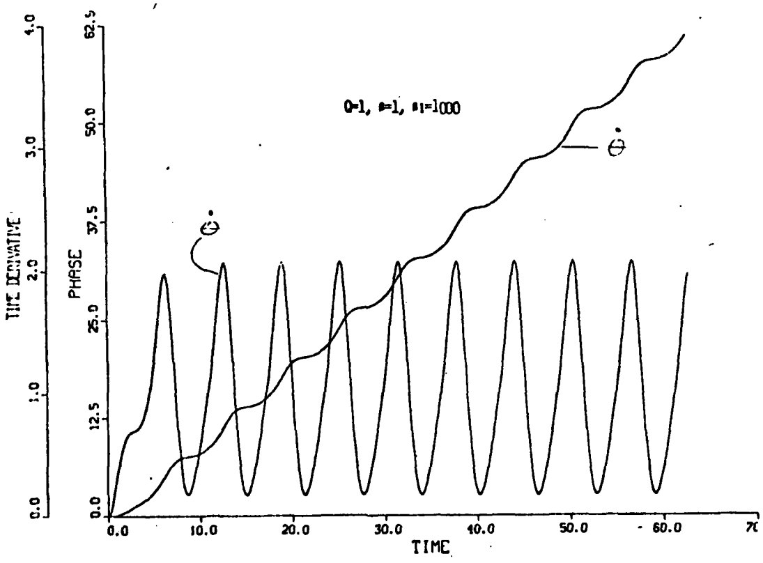
FIGURE 3. Computed time dependence of \theta and \dot{\theta} of the resistive SQUID for Q=1 , \beta=1 and \beta_1=50, 1000 corresponding to \omega_J/\omega_0=0.05 and 1 , respectively. Time is measured in \omega_0^{-1} .
