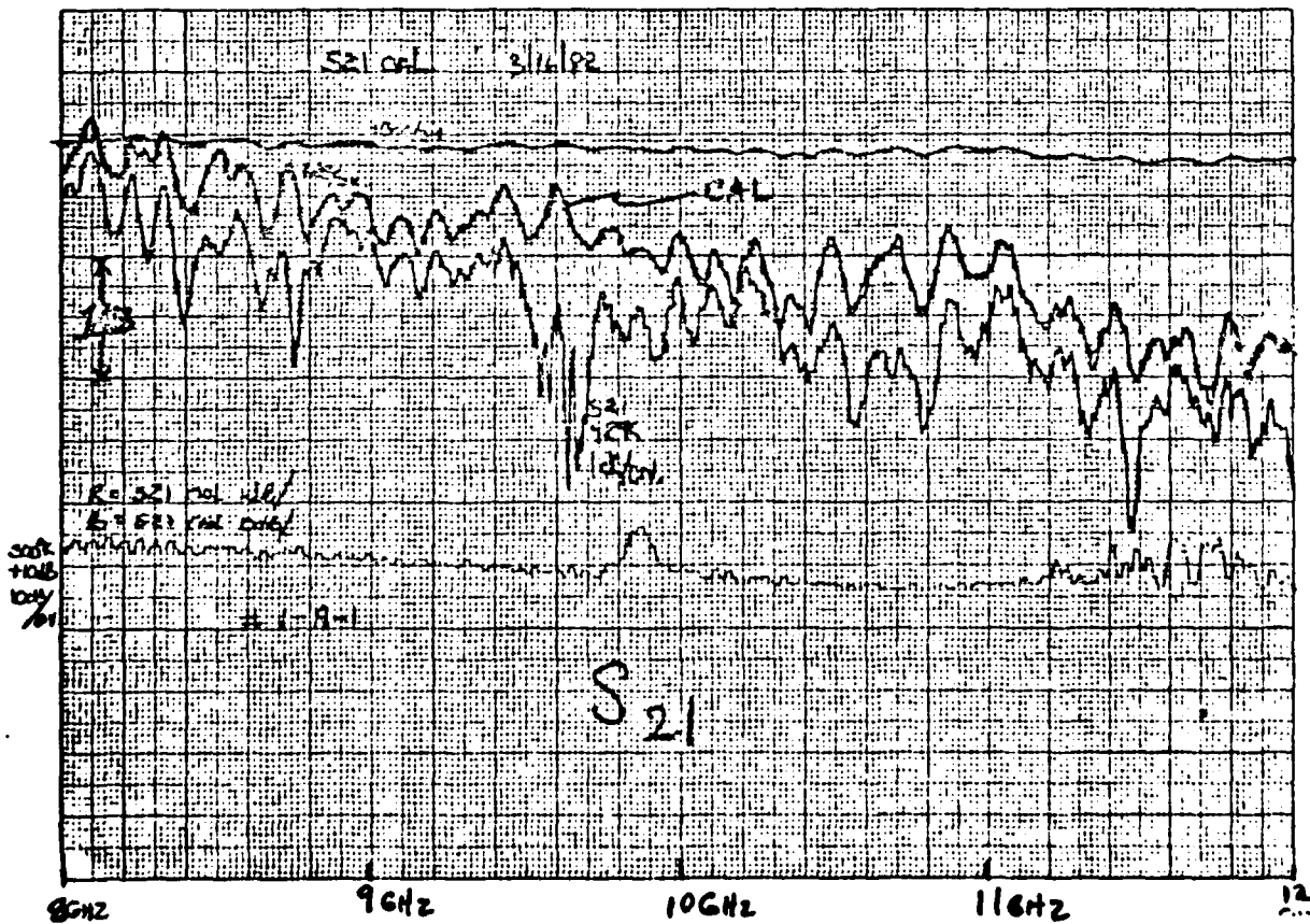
Figure 13. Response of 50Ω tapered coaxial lines on silicon substrate measured at 4K. The upper graph shows S 11 (and S 22 ) at 4K; the faint curve is S 11 at 300K. The lower graph is S 21 at 4K.
