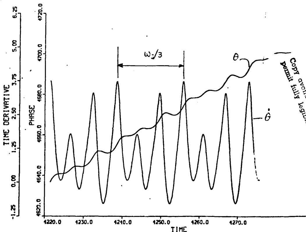
FIGURE 8. Computed time dependence of \theta and \dot{\theta} for the resistive SQUID (lower graph) and power spectrum (upper graph) for Q=5 , \beta=1 and \beta_1=1100 , corresponding to \omega_j=1.1\omega_0 . Time is measured in \omega_0^{-1} and frequency in \omega_0 .
