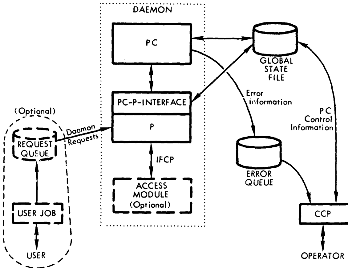
Figure 4-3: Daemon configuration
