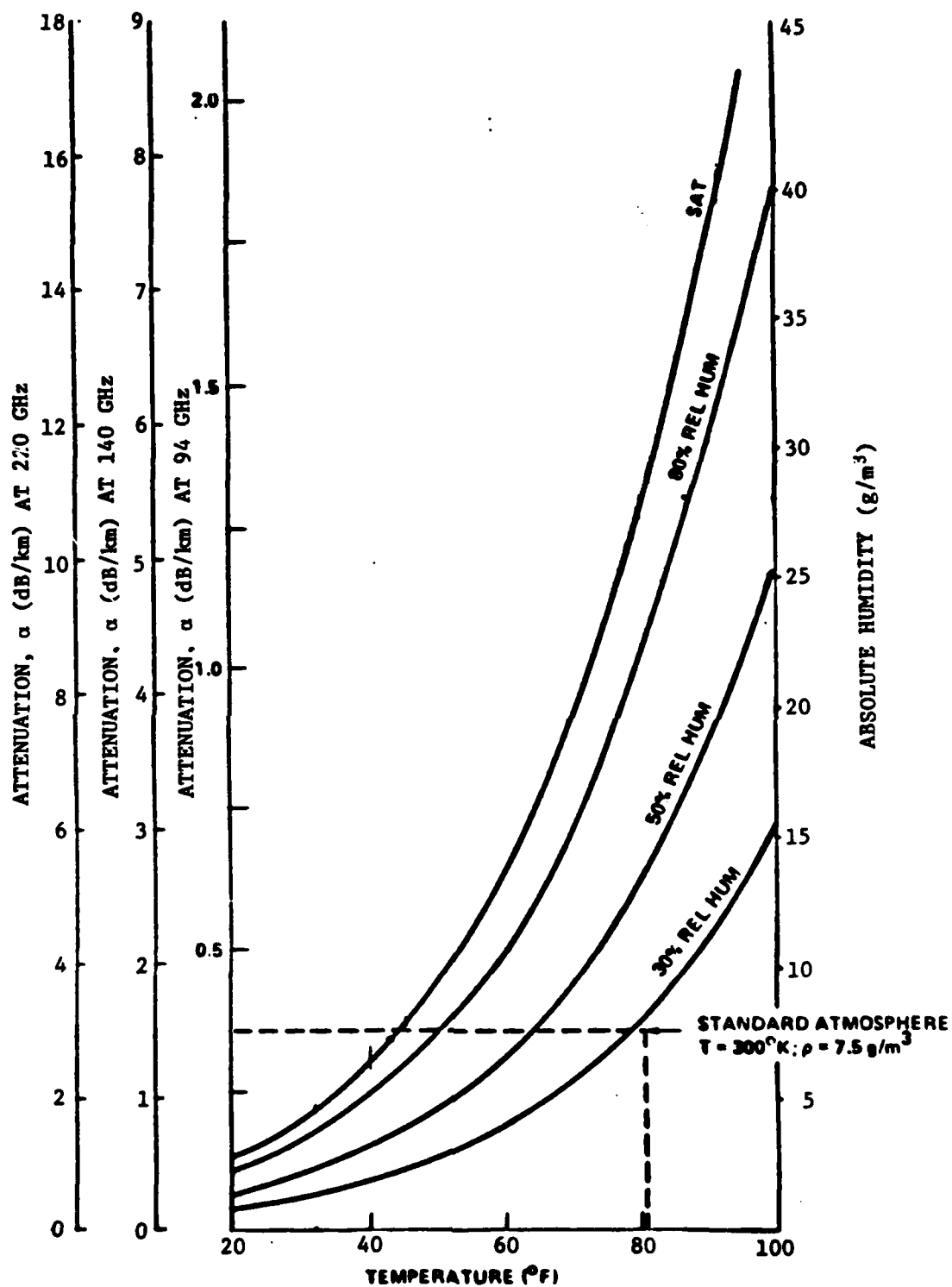
Figure 27. Atmospheric Absorption by Water Vapor.
