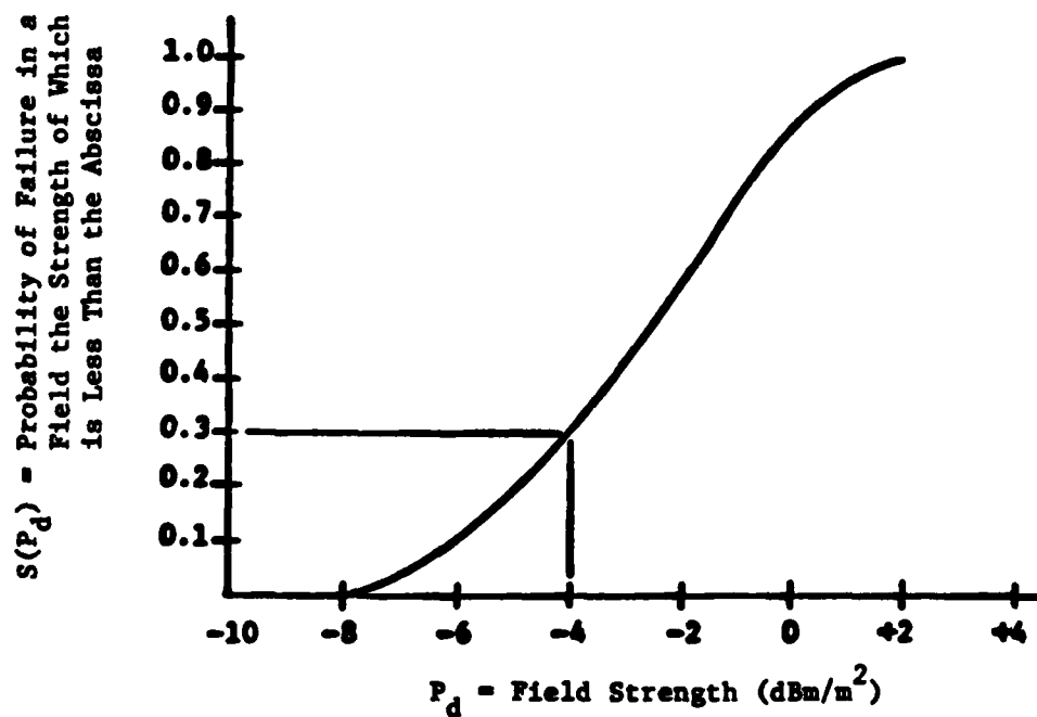
Figure 25. Sample Statistical Description of Case Emissions and Case Susceptibility.
