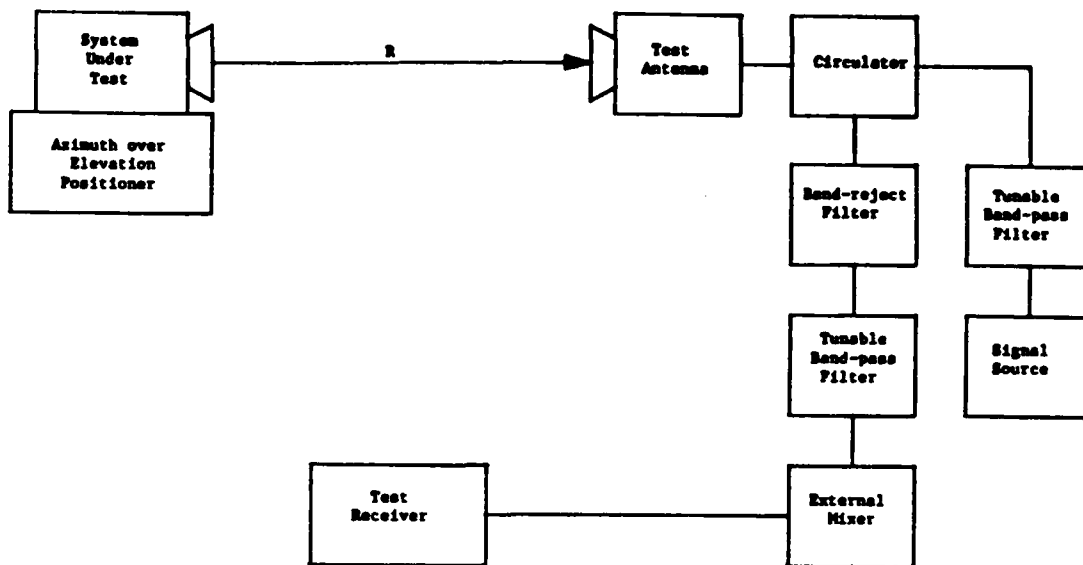
(a) One Test Antenna Method
