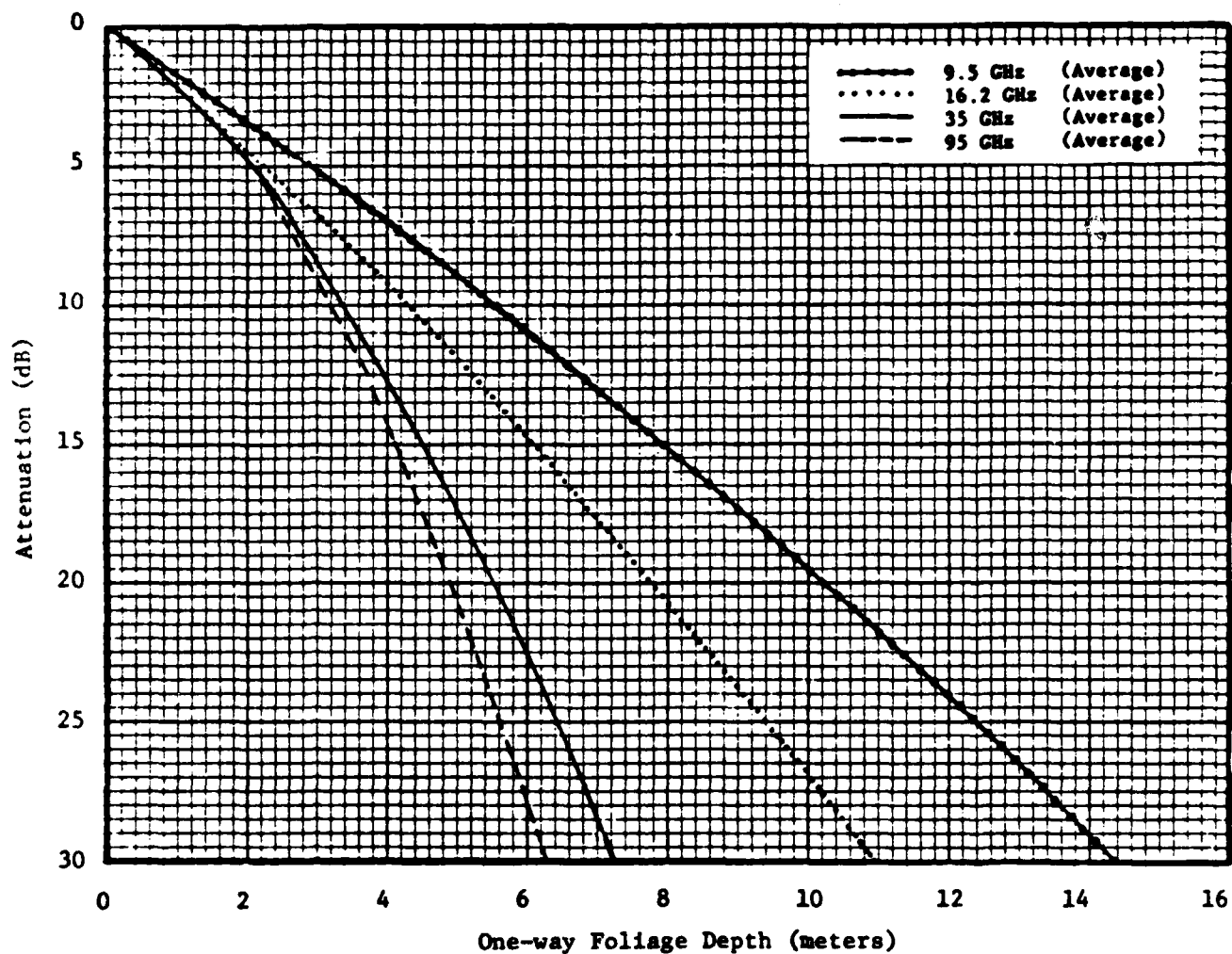
Figure 8. Total Attenuation as a Function of one-way Foliage Depth as Determined by the two-way Experiment [11].
