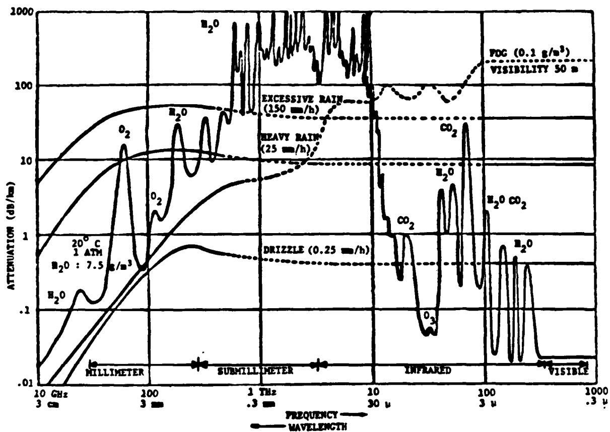
Figure 28. Attenuation by Atmospheric Gases, Rain and Fog.
