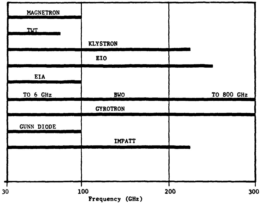
Figure 1. MMW Source Frequency Coverage, State-of-the-Art.
