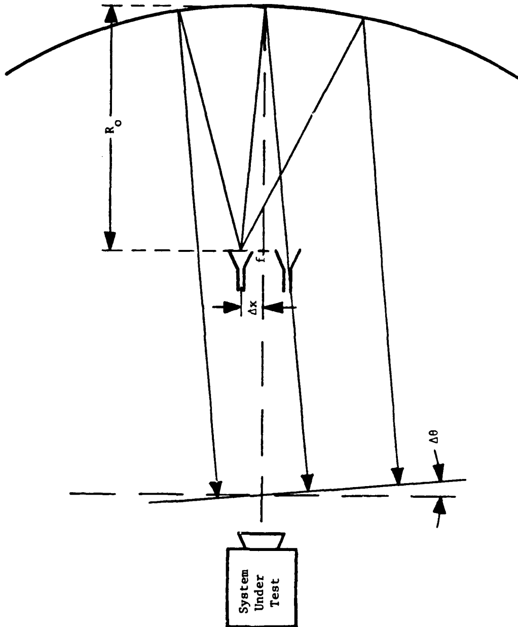
Figure 17. Geometry of Compact Range Test Setup for Two Antenna Intermodulation Test.
