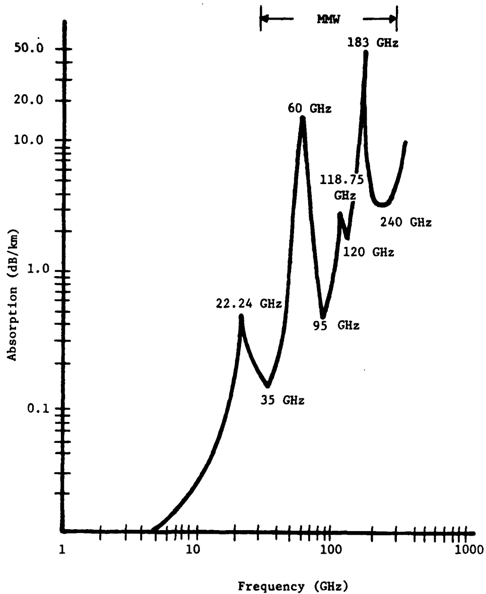
Figure 6. Total Sea Level Atmospheric Absorption. [15].
