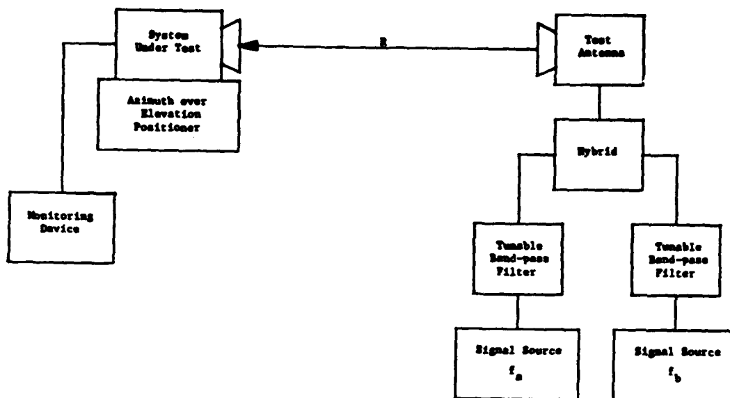
(a) One Test Antenna Method
