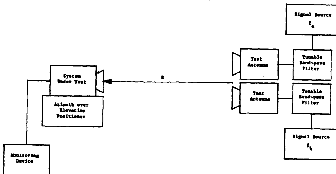
(b) Two Test Antenna Method
