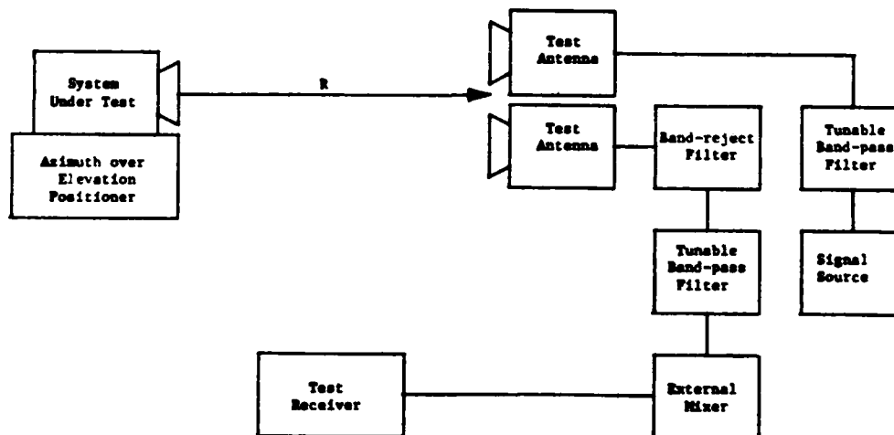
(b) Two Test Antenna Method
