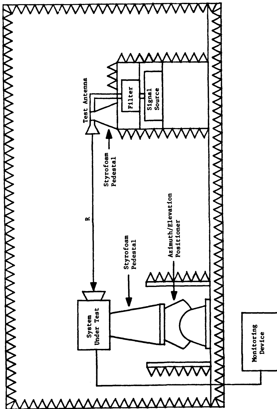
Figure 12. Test Setup for Radiated Susceptibility Measurements Performed in an Anechoic Chamber.
