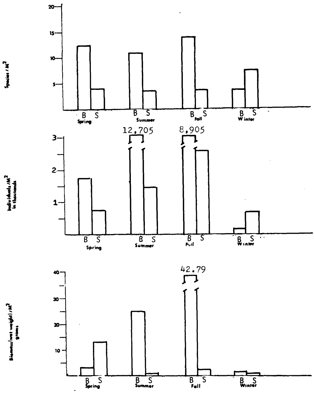
Figure 15. Mean number of species, individuals, and biomass at the bottom (B) and side (S) stations of the navigation channel, at Cow Point, Grays Harbor, Washington, 1980-81.
