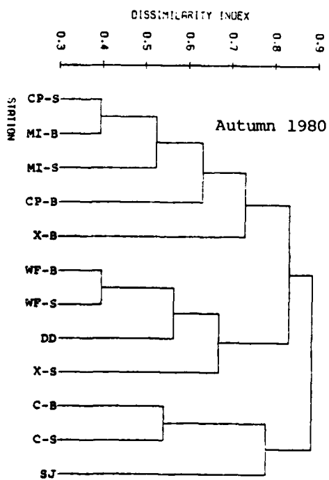
Figure 59. Cluster analysis dendograms for subtidal stations, by season, Grays Harbor, Washington, 1980-1981.
