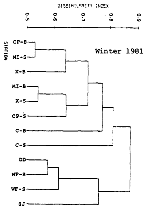
Figure 59. Cluster analysis dendograms for subtidal stations, by season, Grays Harbor, Washington, 1980-1981.
