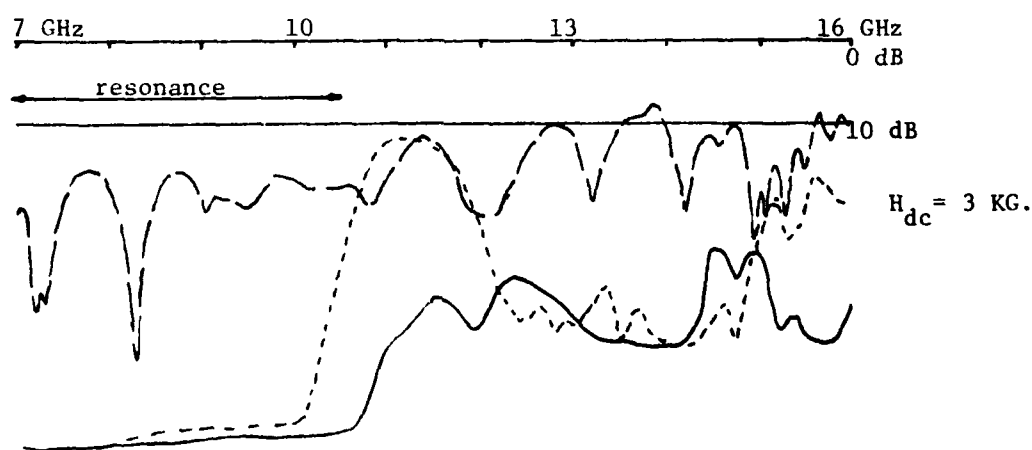
Fig. (5.7b) Guide suspended 1.4 mm above ground plane by means of dielectric
