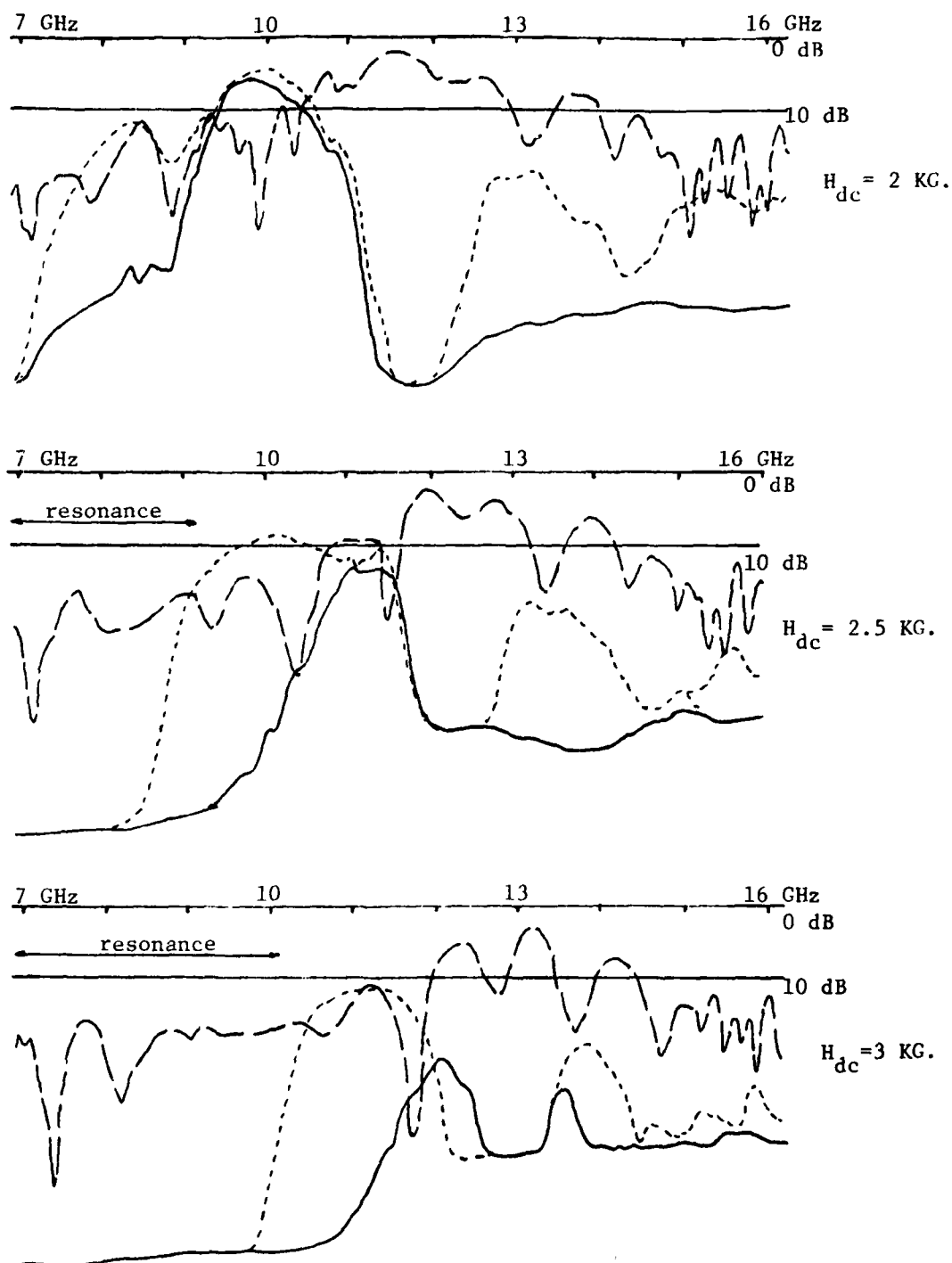
Fig. (5.6b) Guide suspended 0.7 mm above ground plane by means of dielectric
