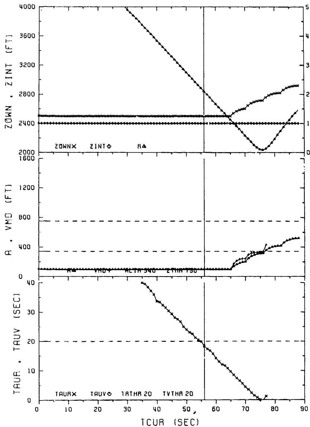
FIGURE 8-21 SEPARATION, TAU PLOTS FOR SCENARIO J IN PERFORMANCE LEVEL 3 (A SUCCESSFUL RESOLUTION)
