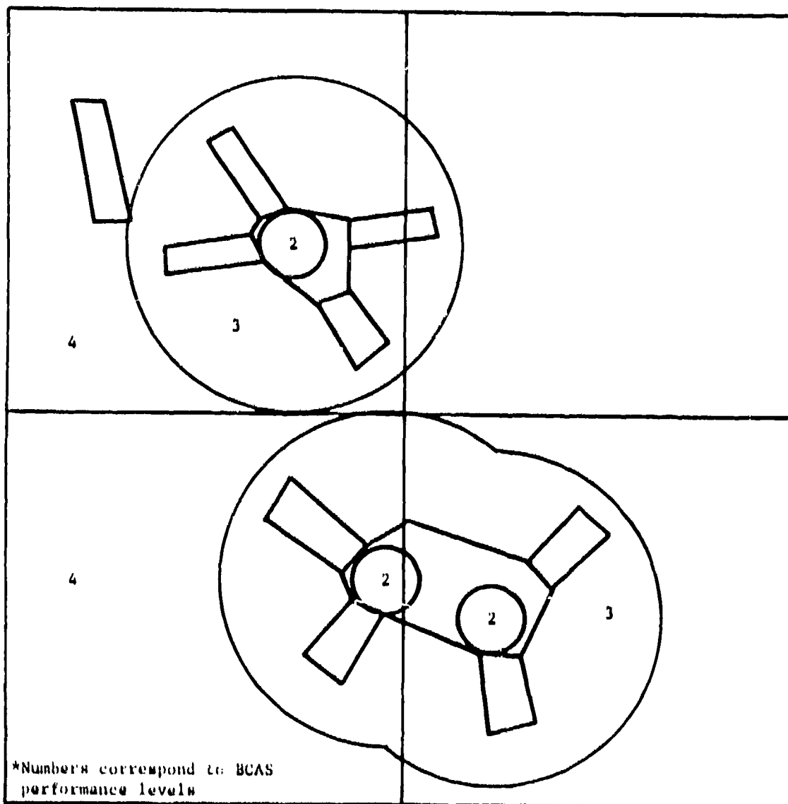
FIGURE 7-3 OVERLAID BCAS AND CONFLICT ALERT MAPS
