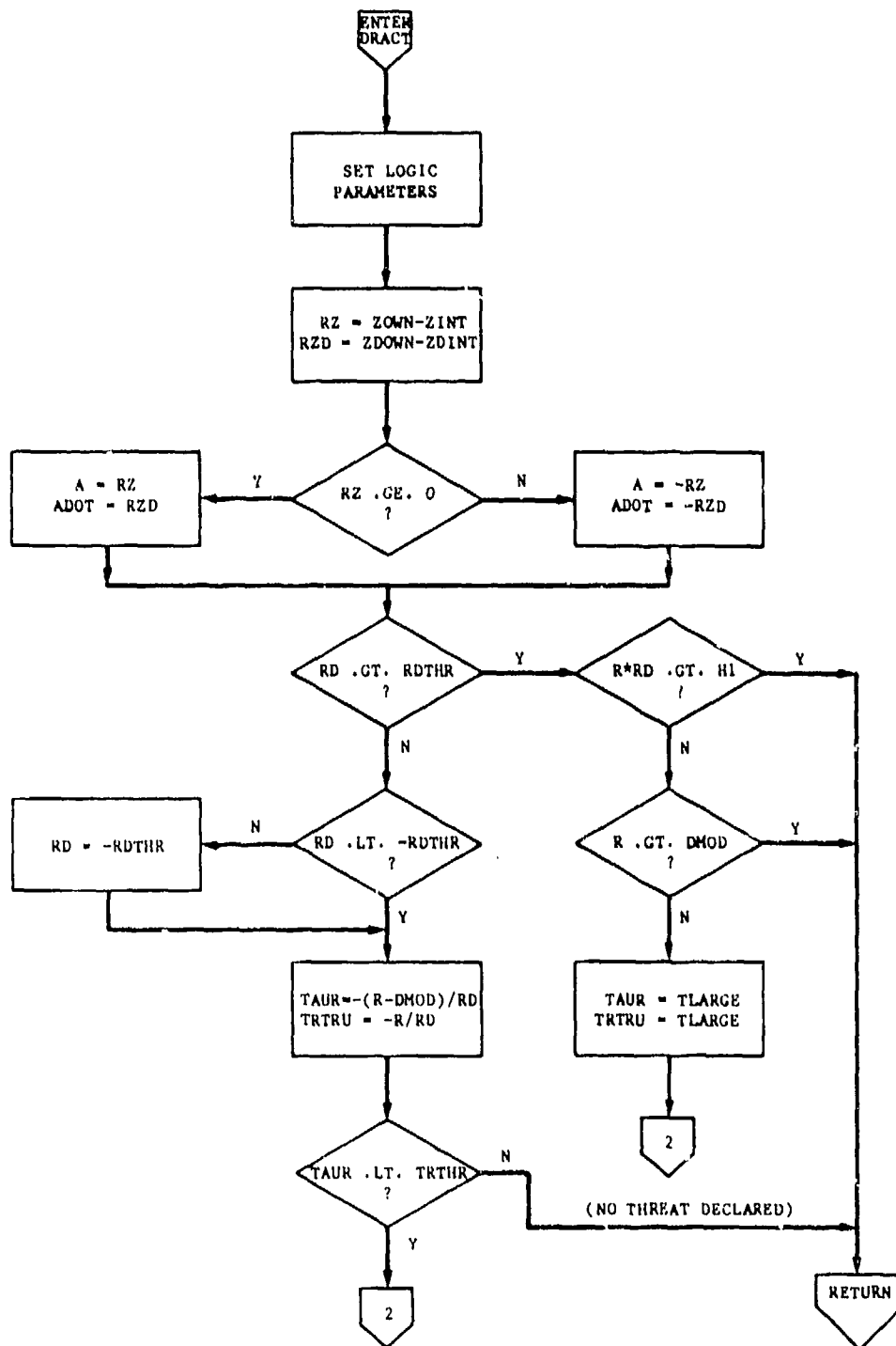
FIGURE 2-3(a) DETECTION AND RESOLUTION (DRACT) FLOWCHART
