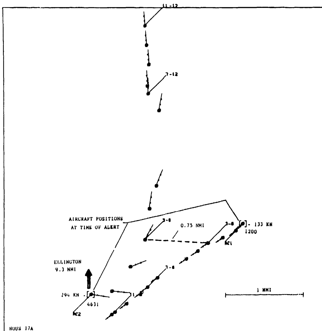
FIGURE 4-7 AN EXAMPLE SHOWING WHY ECAS SHOULD NOT BE INHIBITED BELOW 1000 FEET
