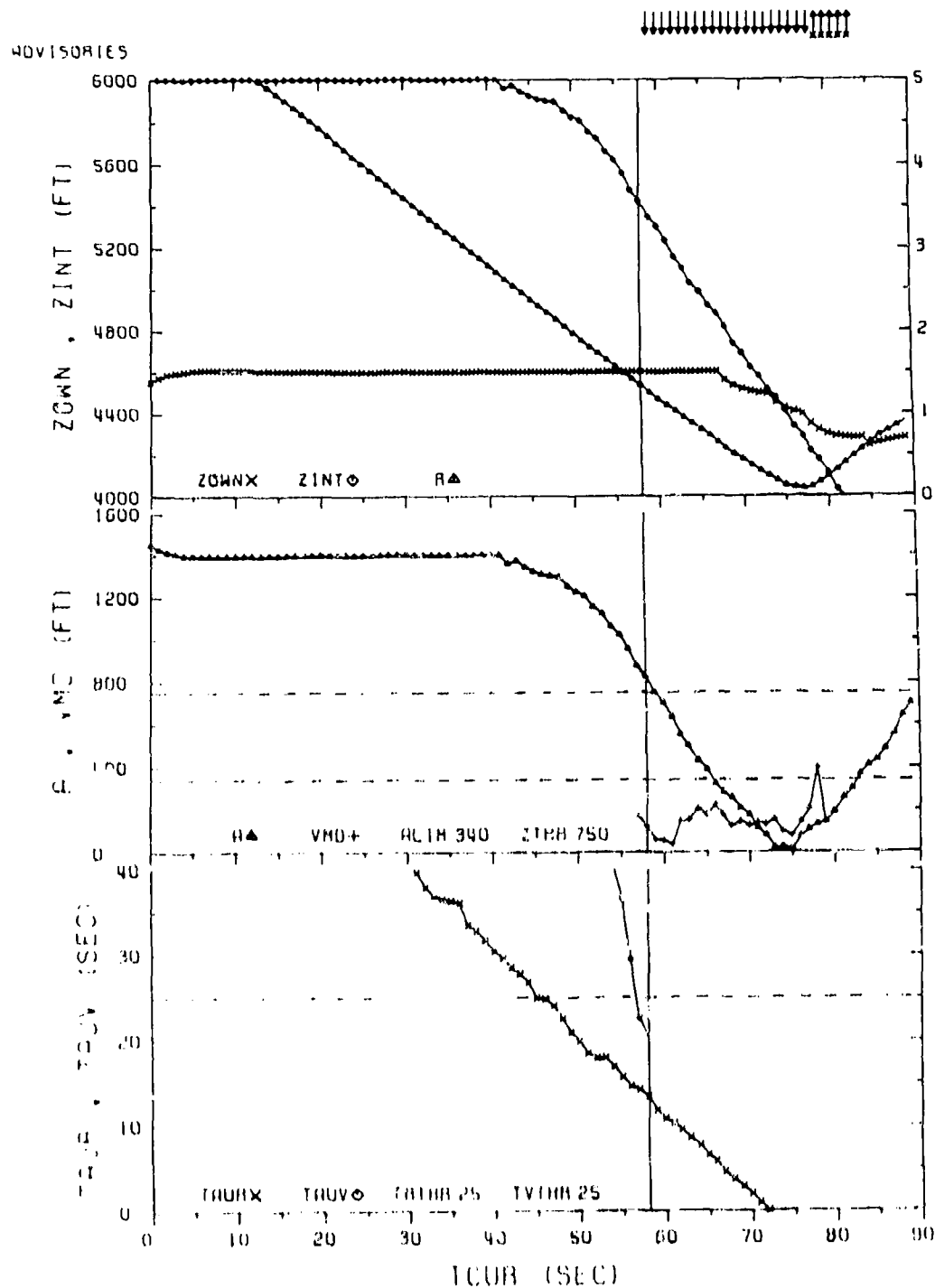
FIGURE 8-28 SEPARATION, TAU PLOTS FOR SCENARIO G IN PERFORMANCE LEVEL 4 (AN UNSUCCESSFUL RESOLUTION)
