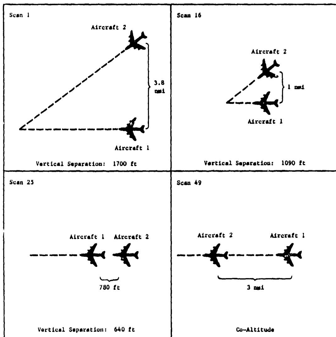
FIGURE 7-6 ENCOUNTER WHICH PRODUCED A BCAS ALERT WITHOUT A CONFLICT ALERT SYSTEM ALERT
