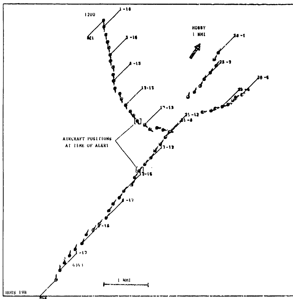
FIGURE 4-5 A JUSTIFIED POSITIVE ALERT IN PERFORMANCE LEVEL 3 REGION
