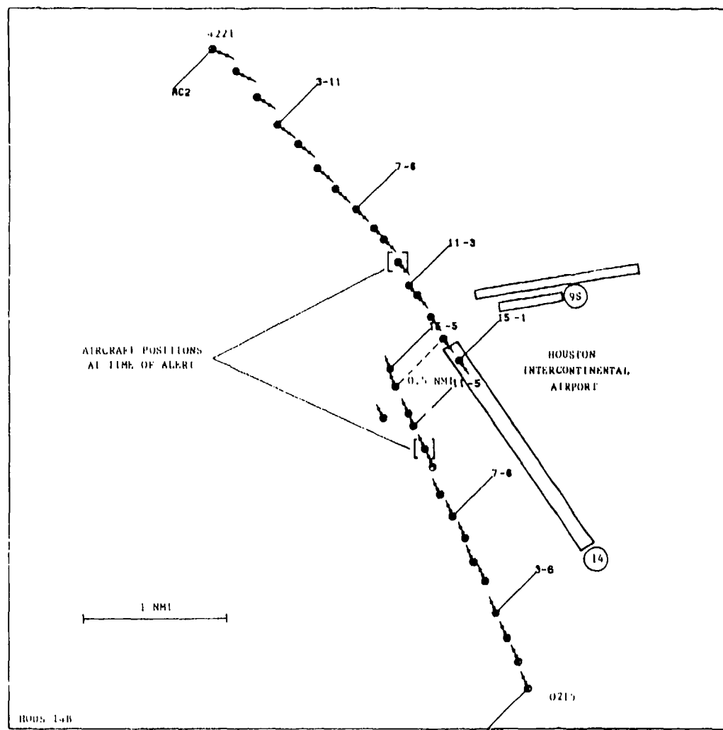
FIGURE 3-10 AN UNNECESSARY POSITIVE ALERT ELIMINATED BY THE 900 FOOT ALTITUDE BOUNDARY
