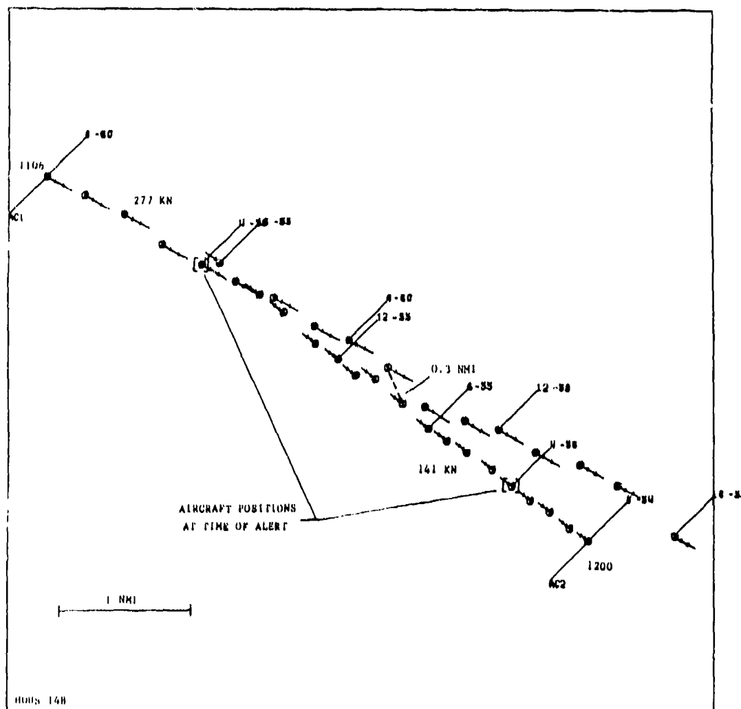
FIGURE 4-8 AN EXAMPLE OF HOW DESENSITIZED ALIM ALLOWS THE 500 FOOT RULE TO WORK INSIDE THE TCA
