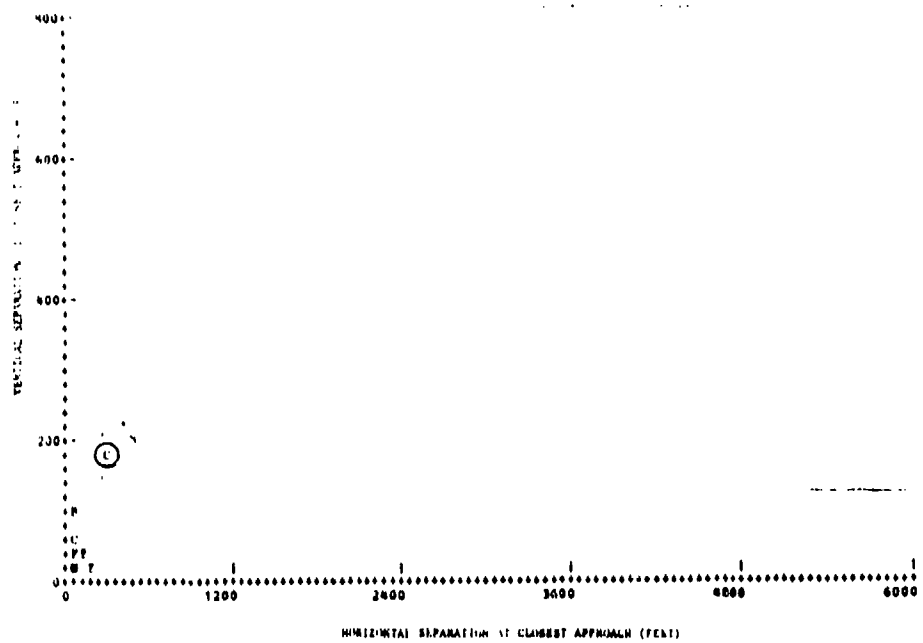
FIGURE 8-4 SEPARATION AT CLOSEST APPROACH WITHOUT BCAS RESOLUTION FOR ALL 15 MIDAIR SCENARIOS IN AN 'ERROR-FREE' ENVIRONMENT
