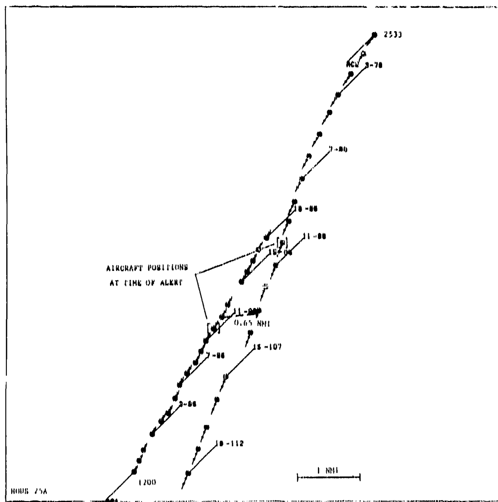
FIGURE 5-3 AN UNNECESSARY POSITIVE ALERT ELIMINATED BY VERTICAL DIVERGENCE LOGIC
