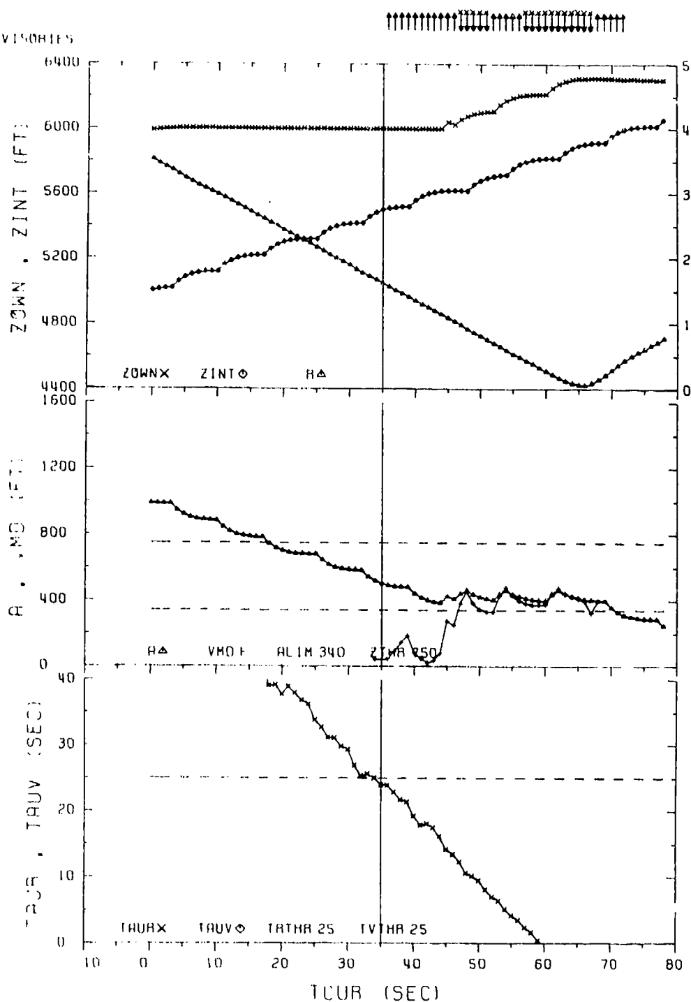
FIGURE 8-23 SEPARATION, TAU PLOTS FOR SCENARIO C IN PERFORMANCE LEVEL 4 (A SUCCESSFUL RESOLUTION)
