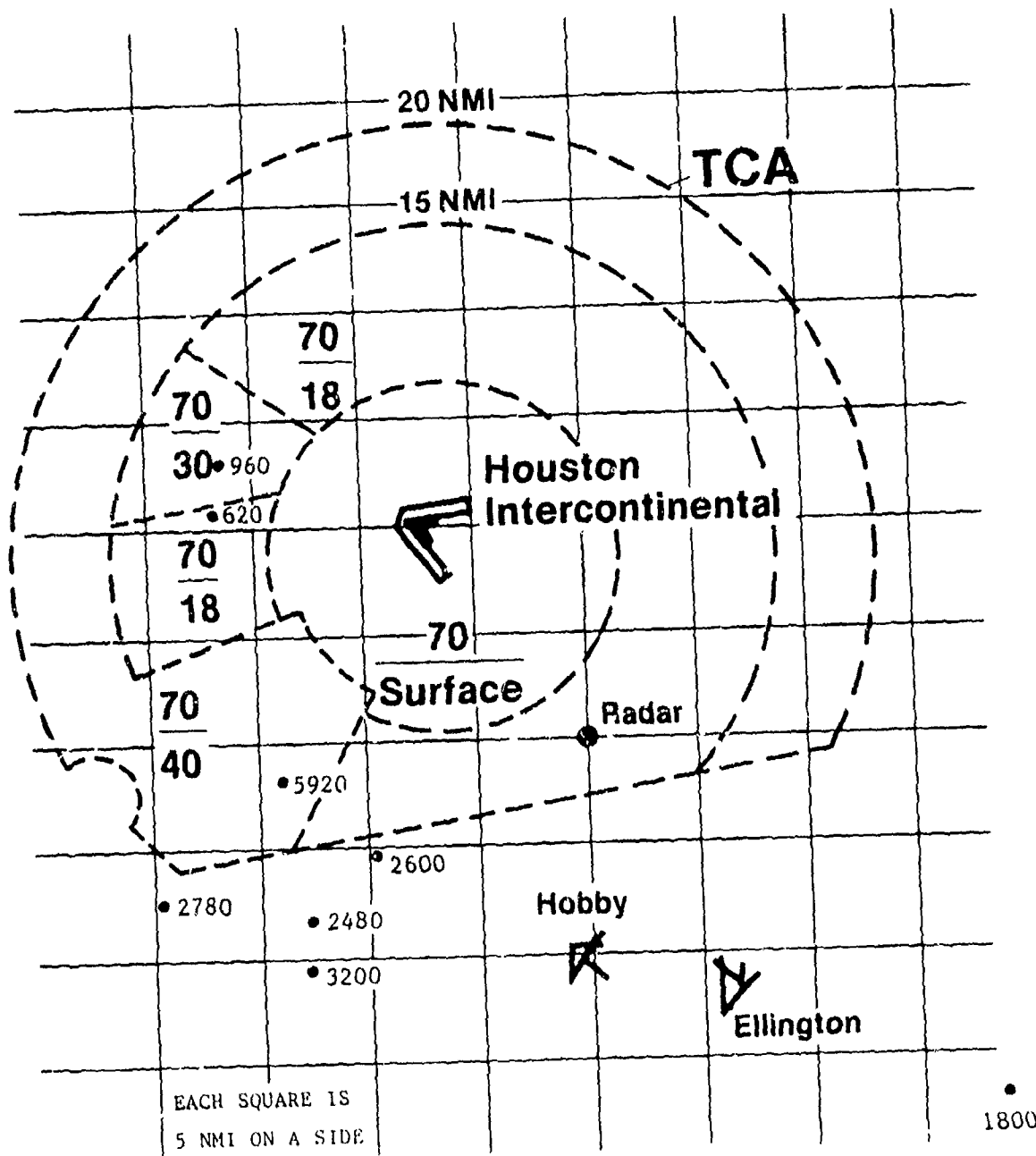
FIGURE D-2(b) LOCATION OF PERFORMANCE LEVEL 4 POSITIVE ALERTS BETWEEN ONE ATC AND ONE 1200-CODE AIRCRAFT
