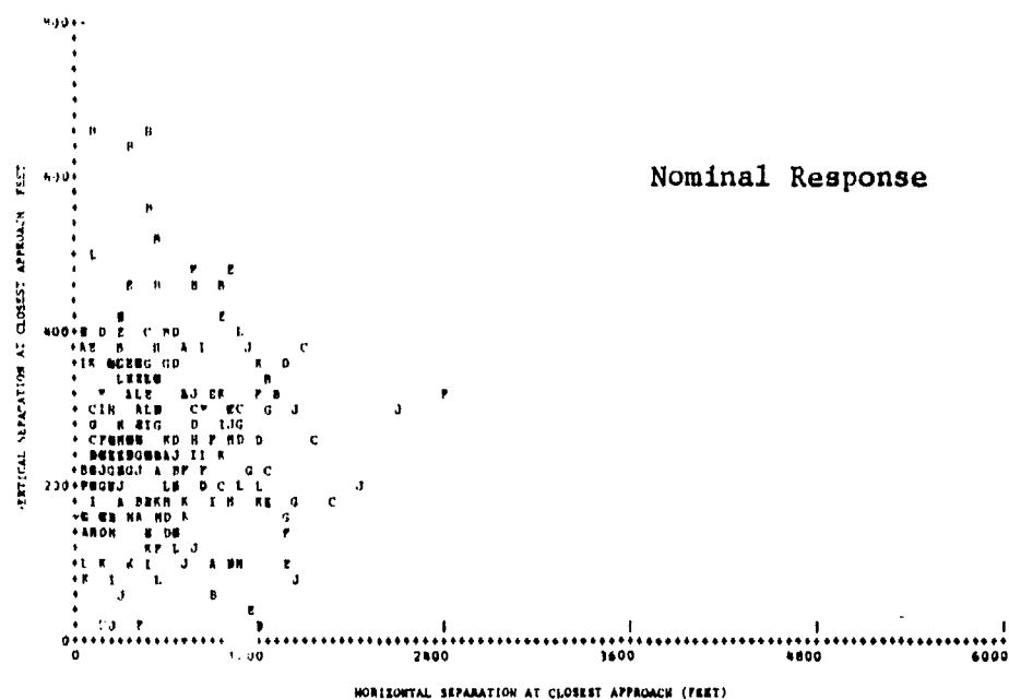
FIGURE 8-19 COMPARISON PLOTS OF NOMINAL RESPONSE VERSUS ZERO ALTIMETRY ERRORS (PERFORMANCE LEVEL 3 SCENARIOS— ONE UNEQUIPPED)
