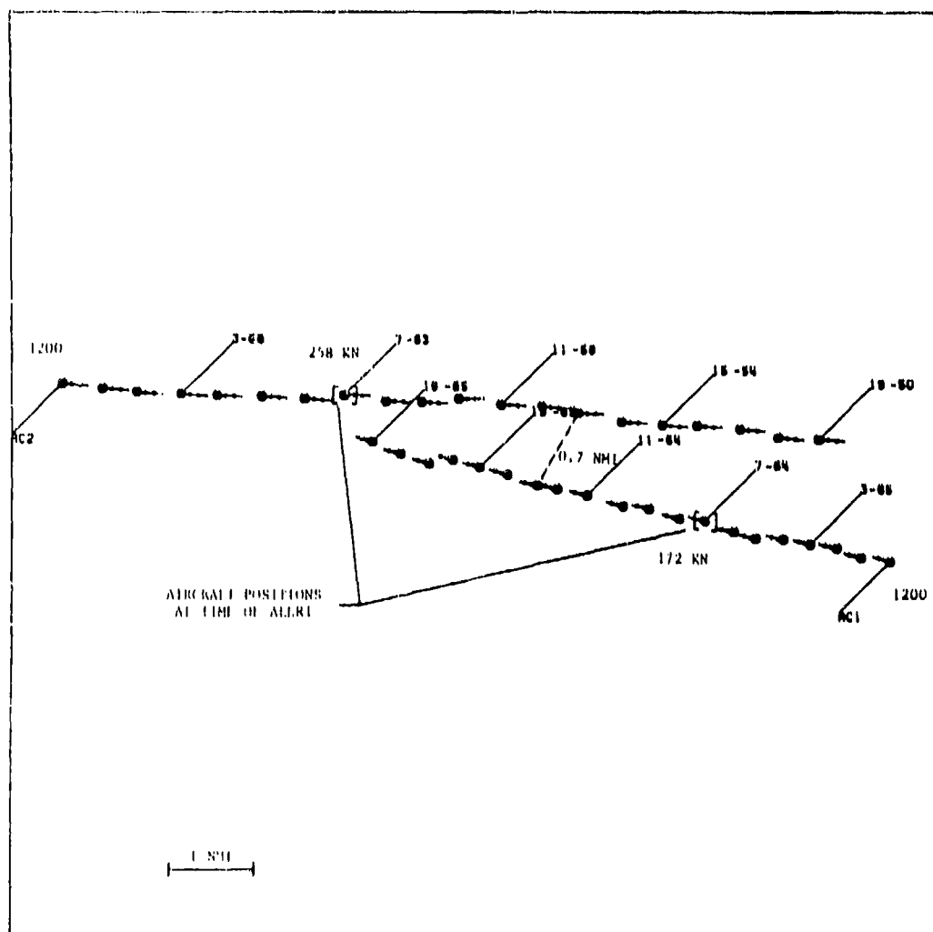
FIGURE 5-2 AN UNNECESSARY POSITIVE ALERT ELIMINATED BY VERTICAL DIVERGENCE LOGIC
