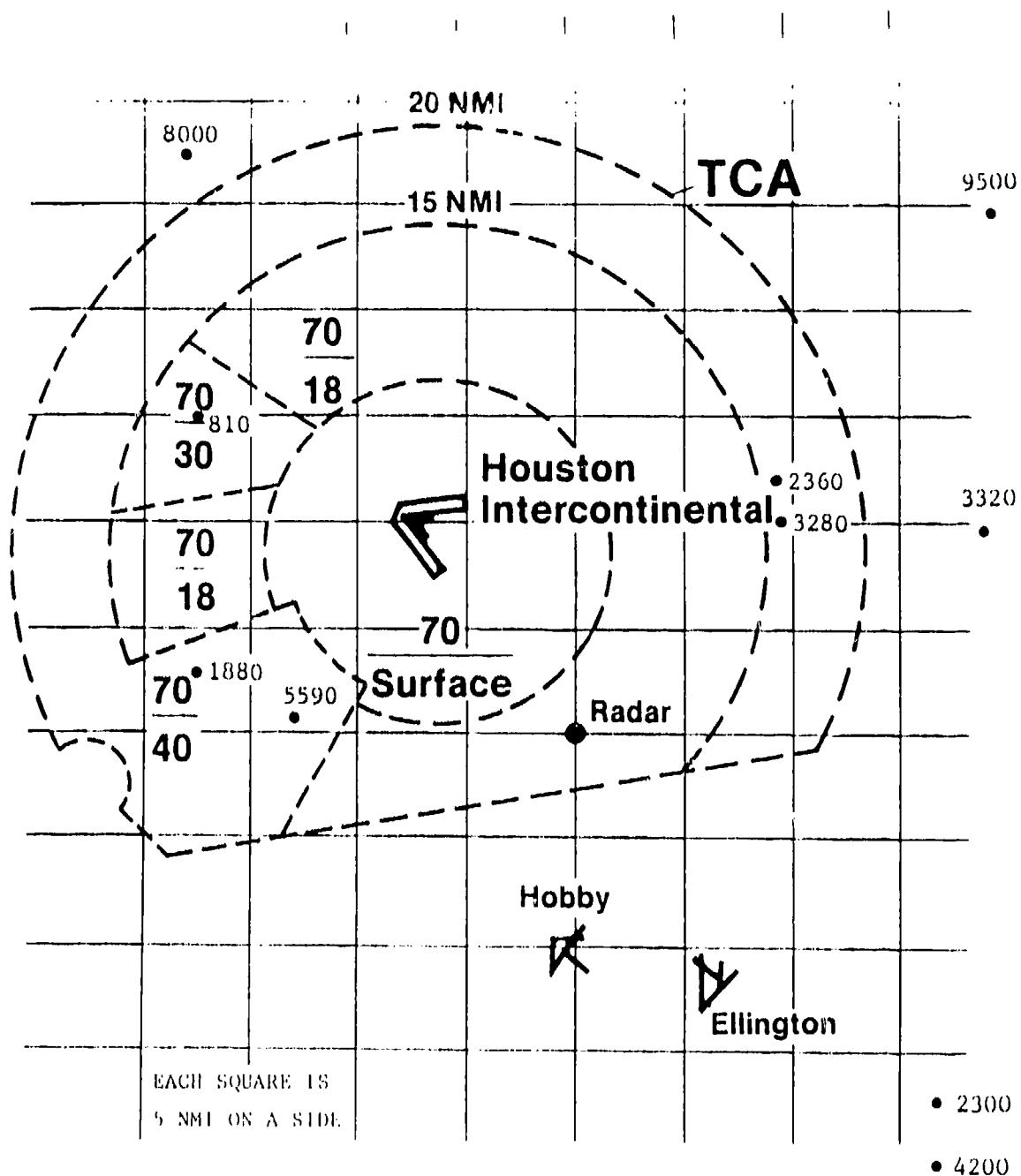
FIGURE D-1(b) LOCATION OF PERFORMANCE LEVEL 4 POSITIVE ALERTS BETWEEN TWO ATC-CODE AIRCRAFT
