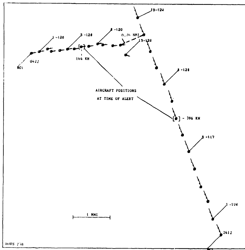
FIGURE 3-14 A JUSTIFIED POSITIVE ALERT IN PERFORMANCE LEVEL 5 REGION
