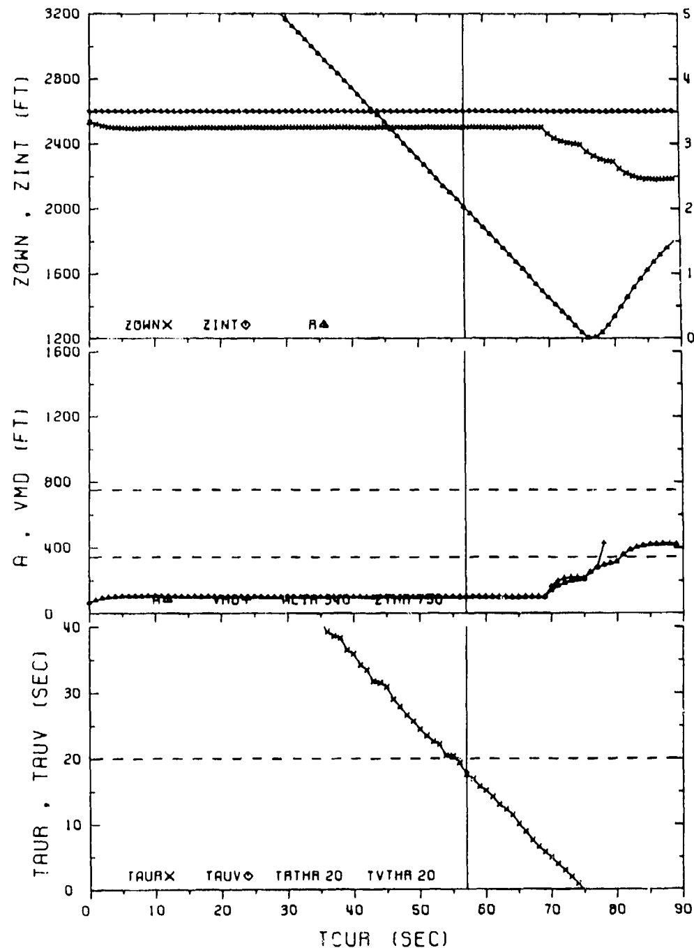
FIGURE 8-20 SEPARATION, TAU PLOTS FOR SCENARIO J IN PERFORMANCE LEVEL 3 (AN UNSUCCESSFUL RESOLUTION)
