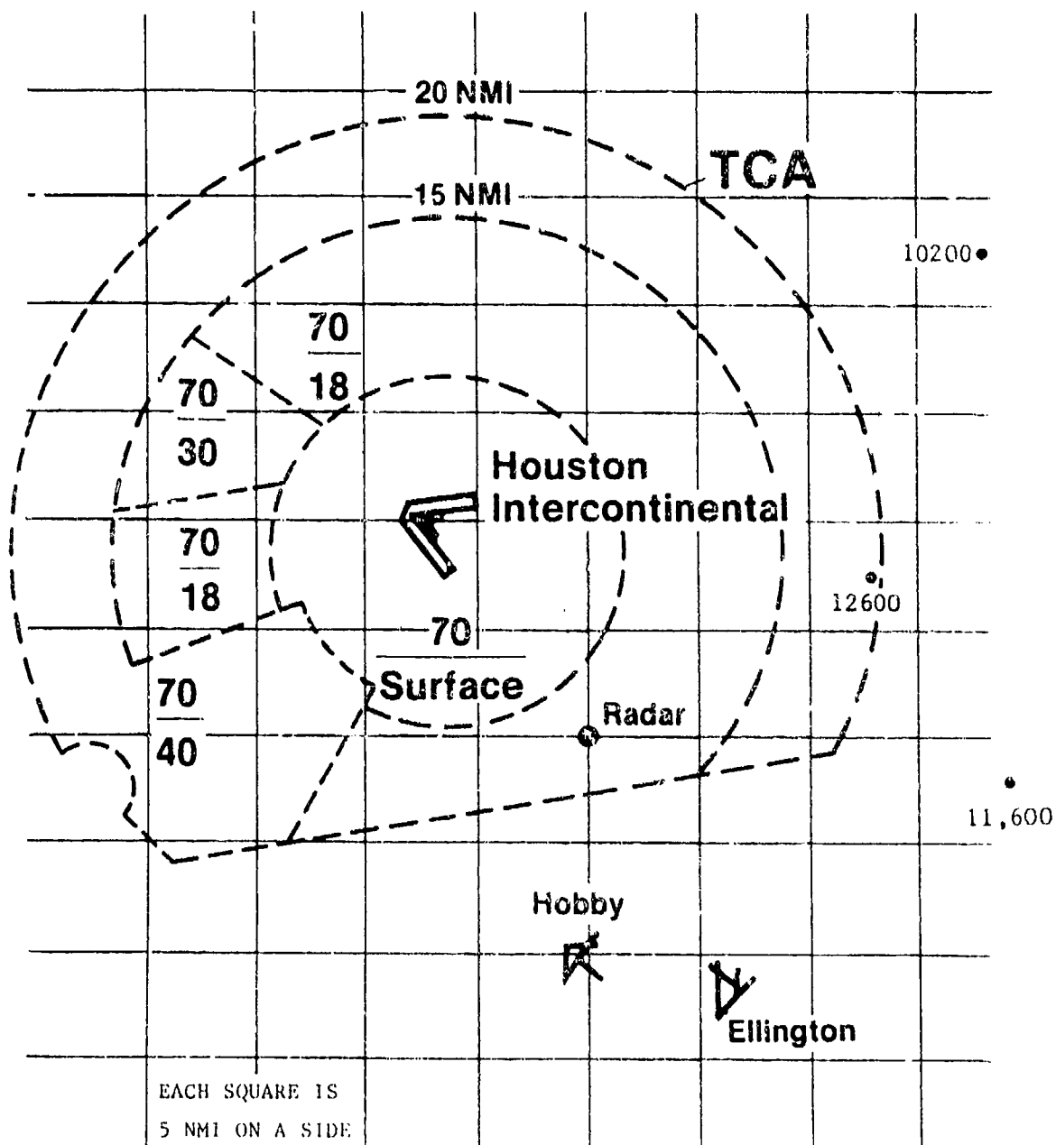
FIGURE D-2(c) LOCATION OF PERFORMANCE LEVEL 5 POSITIVE ALERTS BETWEEN ONE ATC AND ONE 1200-CODE AIRCRAFT
