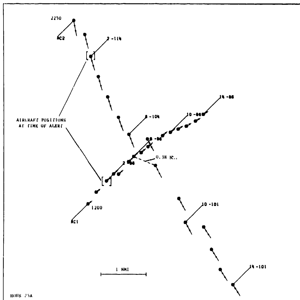
FIGURE 5-6 EXAMPLE OF A LEVEL-OFF SCENARIO
