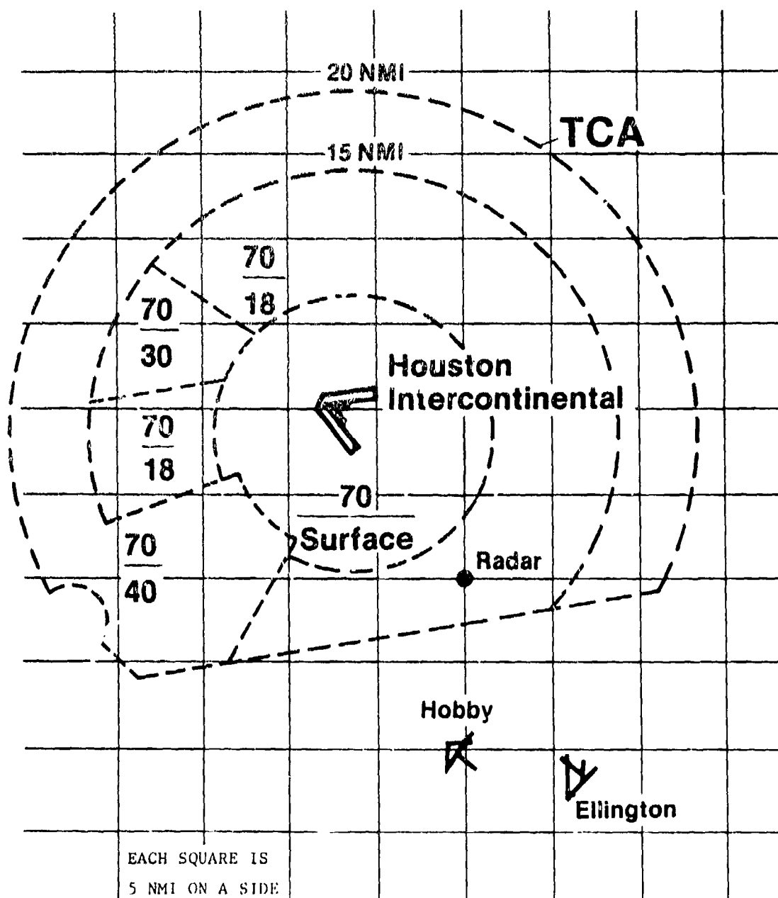
FIGURE D-3(c) LOCATION OF PERFORMANCE LEVEL 5 POSITIVE ALERTS BETWEEN TWO 1200-CODE AIRCRAFT
