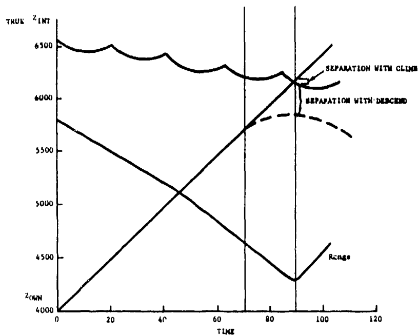
FIGURE 8-36 SEPARATION PLOT FOR SCENARIO E IN PERFORMANCE LEVEL 3 (AN UNSUCCESSFUL RESOLUTION DUE TO ALTIMETRY ERROR)
