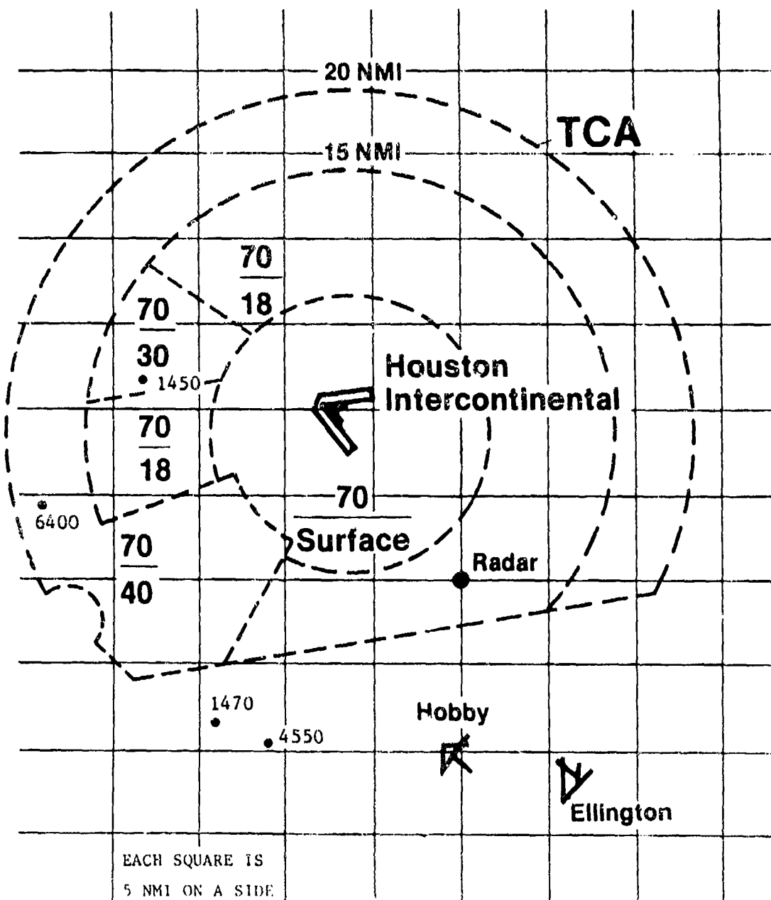
FIGURE D-3(b) LOCATION OF PERFORMANCE LEVEL 4 POSITIVE ALERTS BETWEEN TWO 1200-CODE AIRCRAFT
