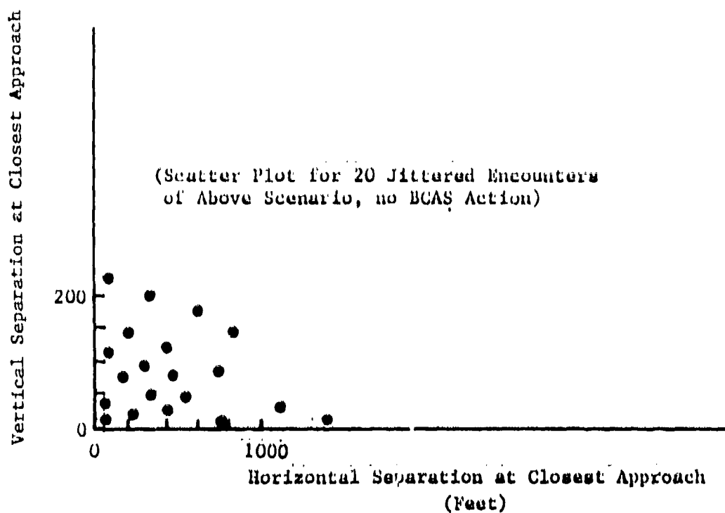
FIGURE 8-2 HORIZONTAL PLOT OF AN INPUT SCENARIO AND ITS RELATIONSHIP TO THE JITTERED ENCOUNTERS
