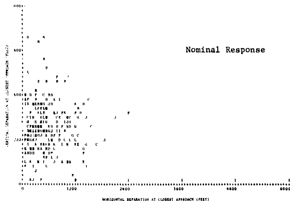
FIGURE 8-17 COMPARISON PLOTS OF NOMINAL RESPONSE VERSUS NO RESPONSE DEVIATION (PERFORMANCE LEVEL 3 SCENARIOS— ONE UNEQUIPPED)
