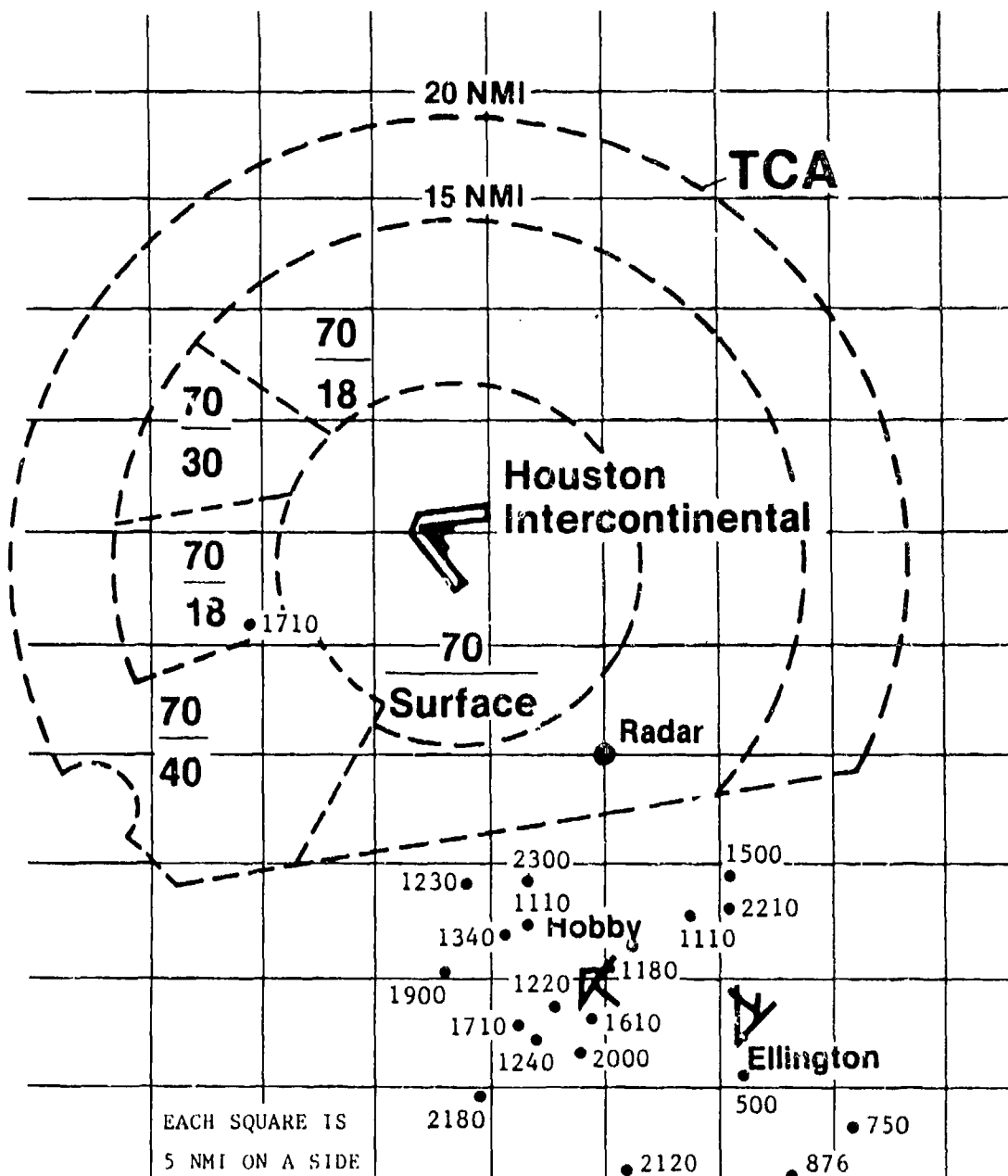
FIGURE D-2(a) LOCATION OF PERFORMANCE LEVEL 3 POSITIVE ALERTS BETWEEN ONE ATC AND ONE 1200-CODE AIRCRAFT
