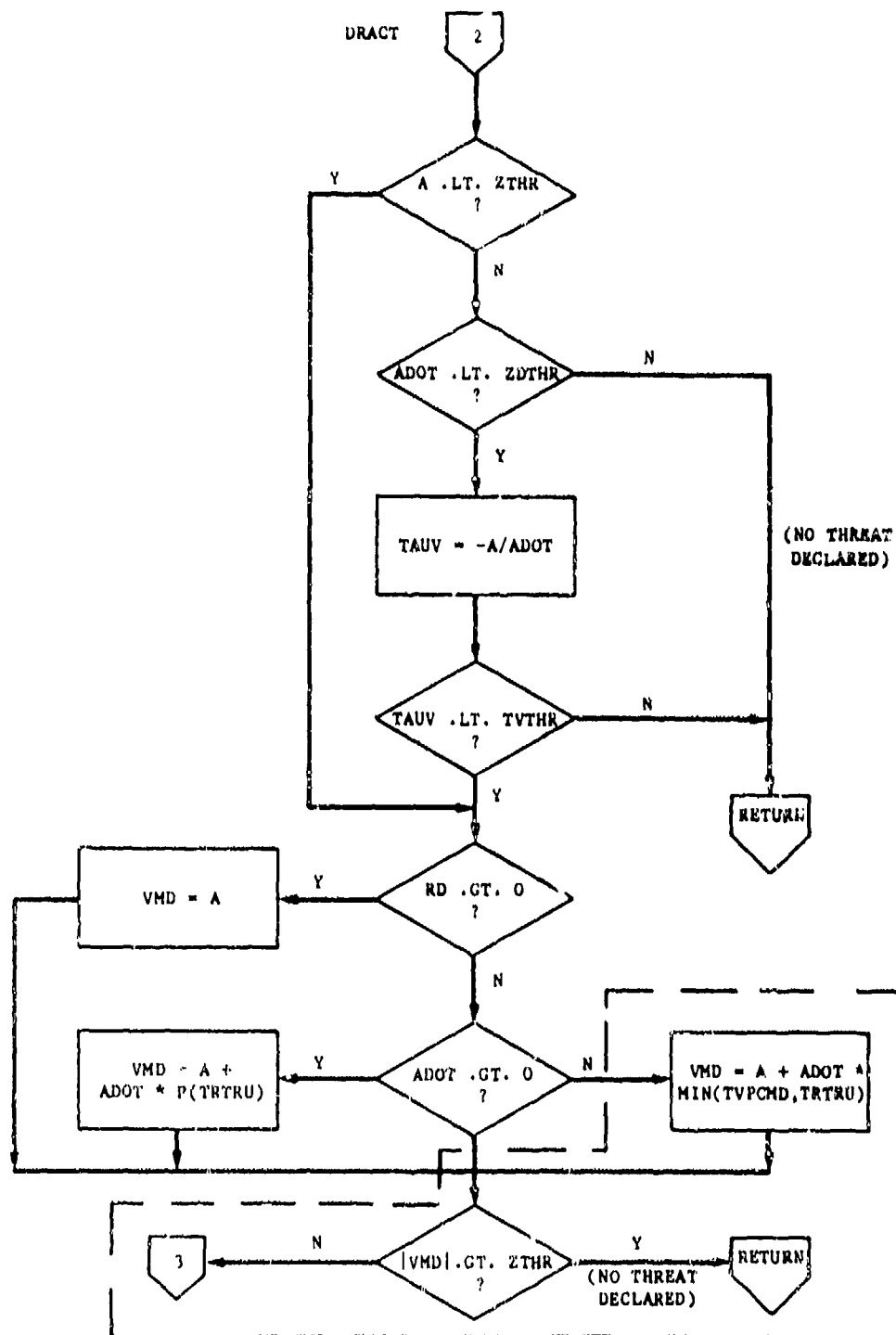
FIGURE 5-1 DETECTION AND RESOLUTION (DRACT) FLOWCHART (MODIFIED VERSION)
