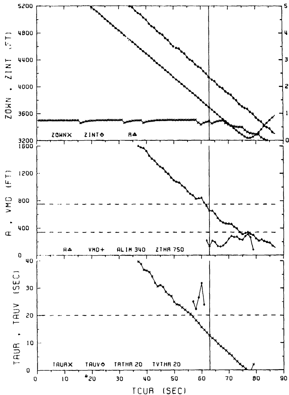
FIGURE 8-22 SEPARATION, TAU PLOTS FOR SCENARIO H IN PERFORMANCE LEVEL 3 (AN UNSUCCESSFUL RESOLUTION)
