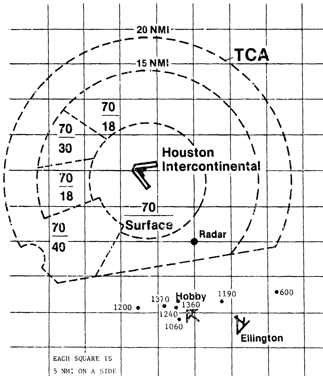
FIGURE D-3(a) LOCATION OF PERFORMANCE LEVEL 3 POSITIVE ALERTS BETWEEN TWO 1200-CODE AIRCRAFT
