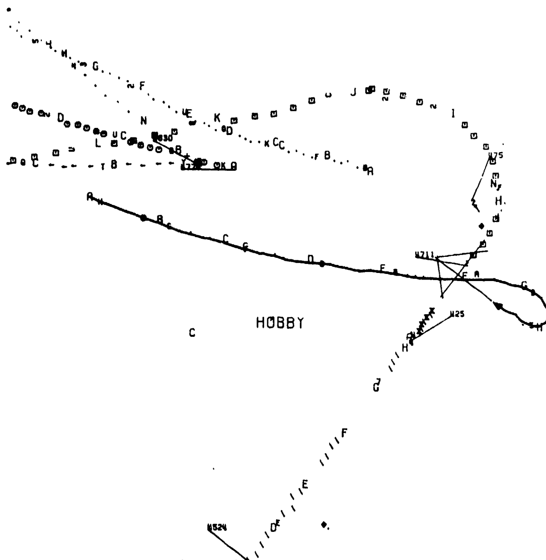
FIGURE 4-10 AIRCRAFT FLIES OVER HOBBY AIRFIELD BEFORE LANDING
