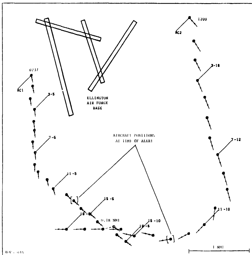
FIGURE 3-9 A LOW ALTITUDE JUSTIFIED POSITIVE ALERT BEYOND THE 2 NMI BOUNDARY
