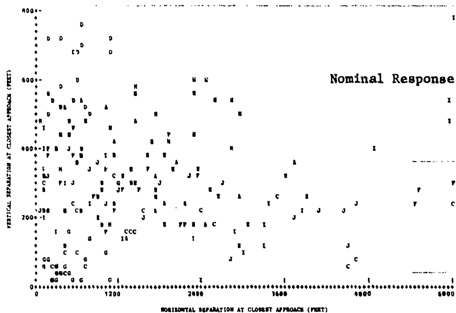
FIGURE 8-38 COMPARISON OF NOMINAL RESPONSE VERSUS SLOWER RESPONSE TIME (PERFORMANCE LEVEL 4 SCENARIOS—ONE UNEQUIPPED)
