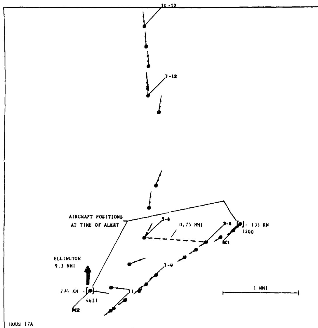
FIGURE 4-3 A LOW ALTITUDE POSITIVE ALERT NOT ELIMINATED BY DESENSITIZATION
