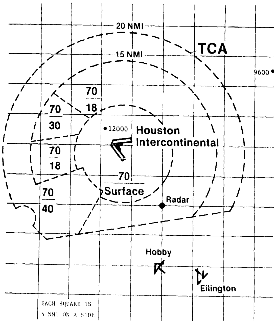
FIGURE D-1(c) LOCATION OF PERFORMANCE LEVEL 5 POSITIVE ALERTS BETWEEN TWO ATC-CODE AIRCRAFT
