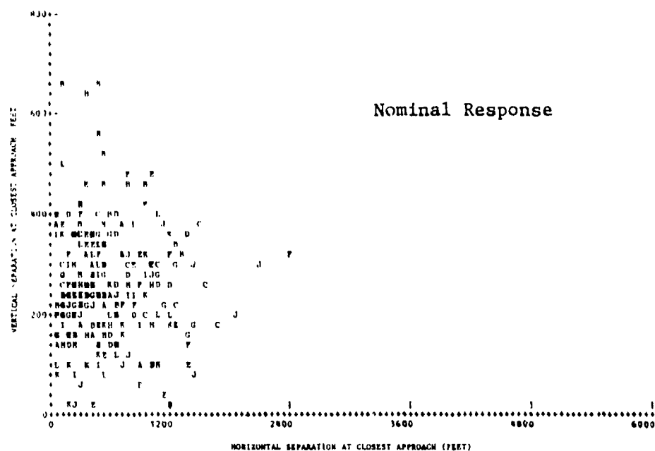
FIGURE 8-18 COMPARISON PLOTS OF NOMINAL RESPONSE VERSUS PERFECT ALTITUDE TRACKING (PERFORMANCE LEVEL 3 SCENARIOS—ONE UNEQUIPPED)
