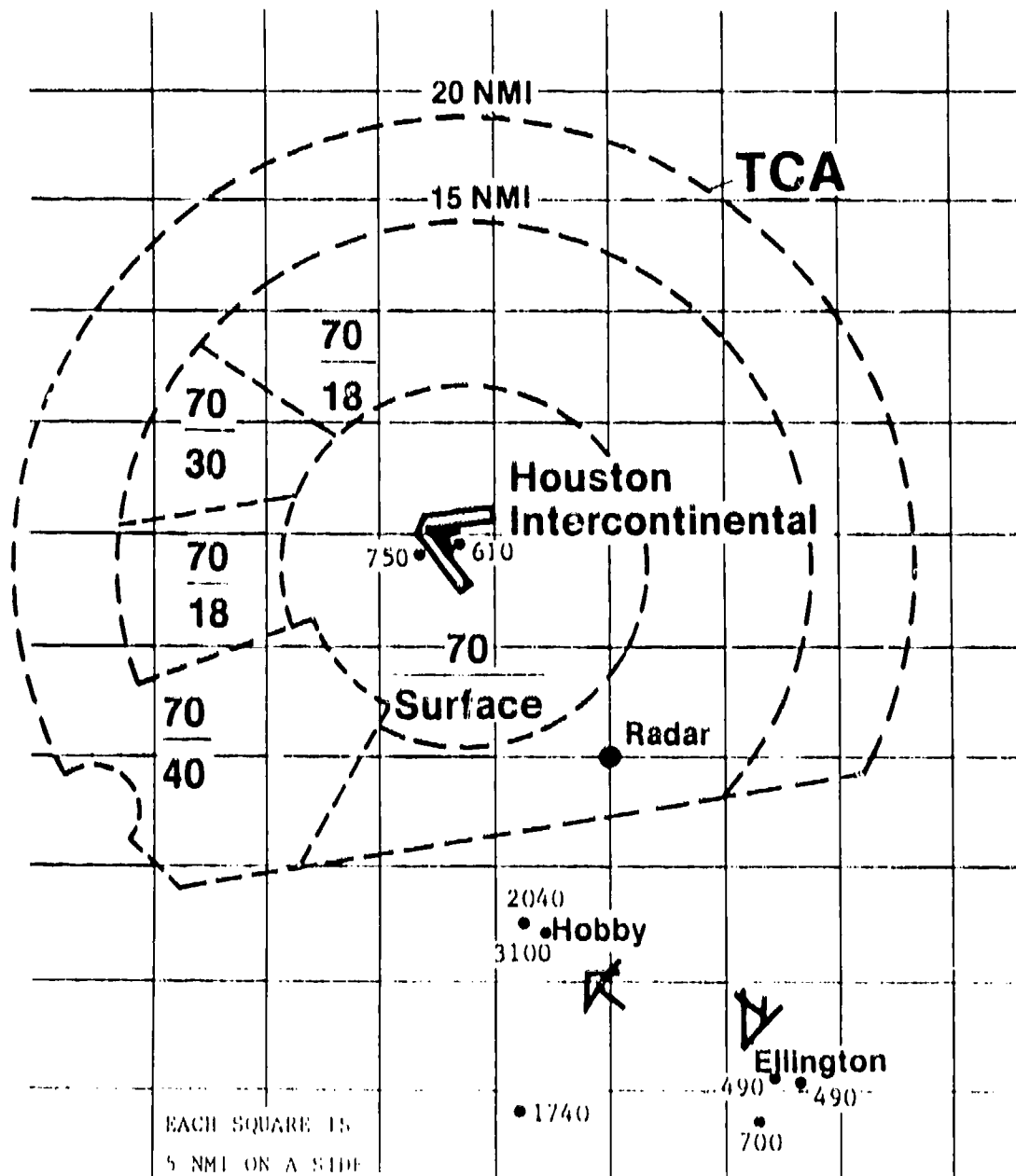
FIGURE D-1(a) LOCATION OF PERFORMANCE LEVEL 3 POSITIVE ALERTS BETWEEN TWO ATC-CODE AIRCRAFT
