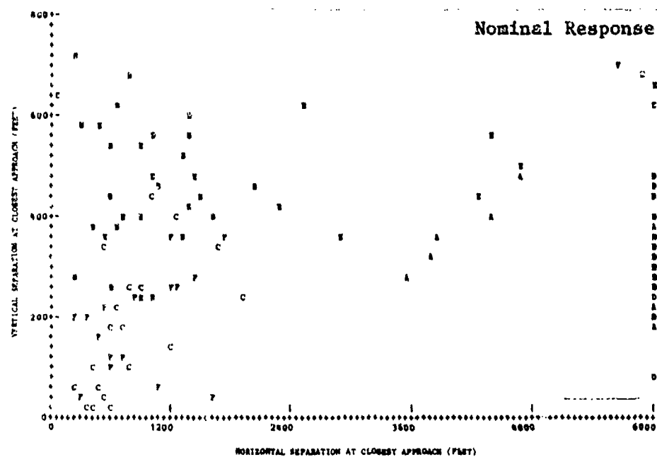
FIGURE 8-39 COMPARISON OF NOMINAL RESPONSE VERSUS SLOWER RESPONSE TIME (PERFORMANCE LEVEL 5 SCENARIOS—ONE UNEQUIPPED)
