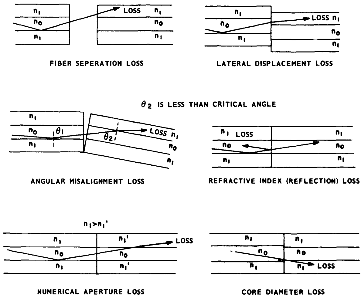
FIGURE A-4. CONNECTOR AND SPLICE LOSS MECHANISMS
