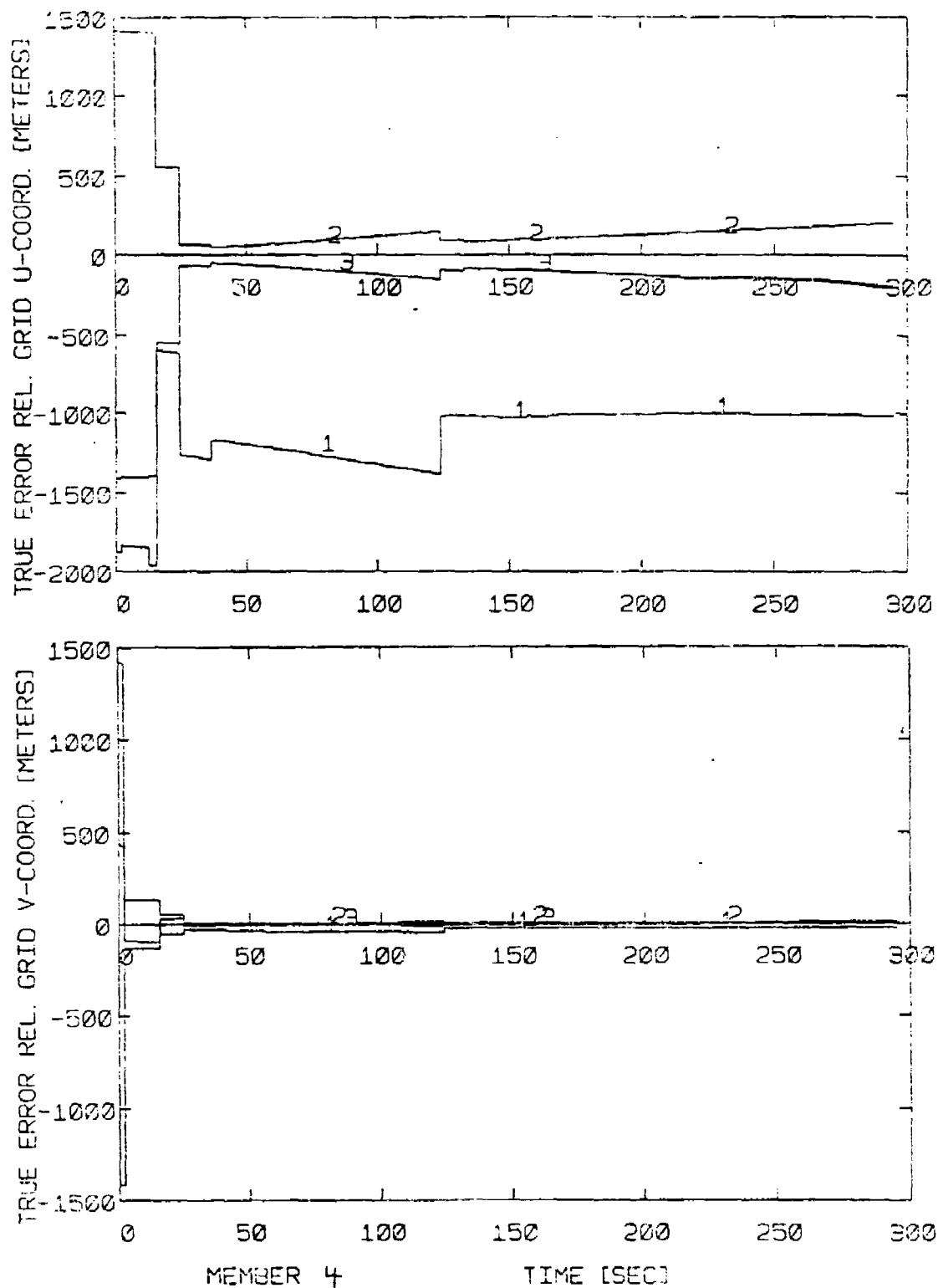
Fig. 7.30(a) Four Member ReInav Results, without Nonlinear Protection, and with More Accurate TOA Measurements (1m), Member 4
