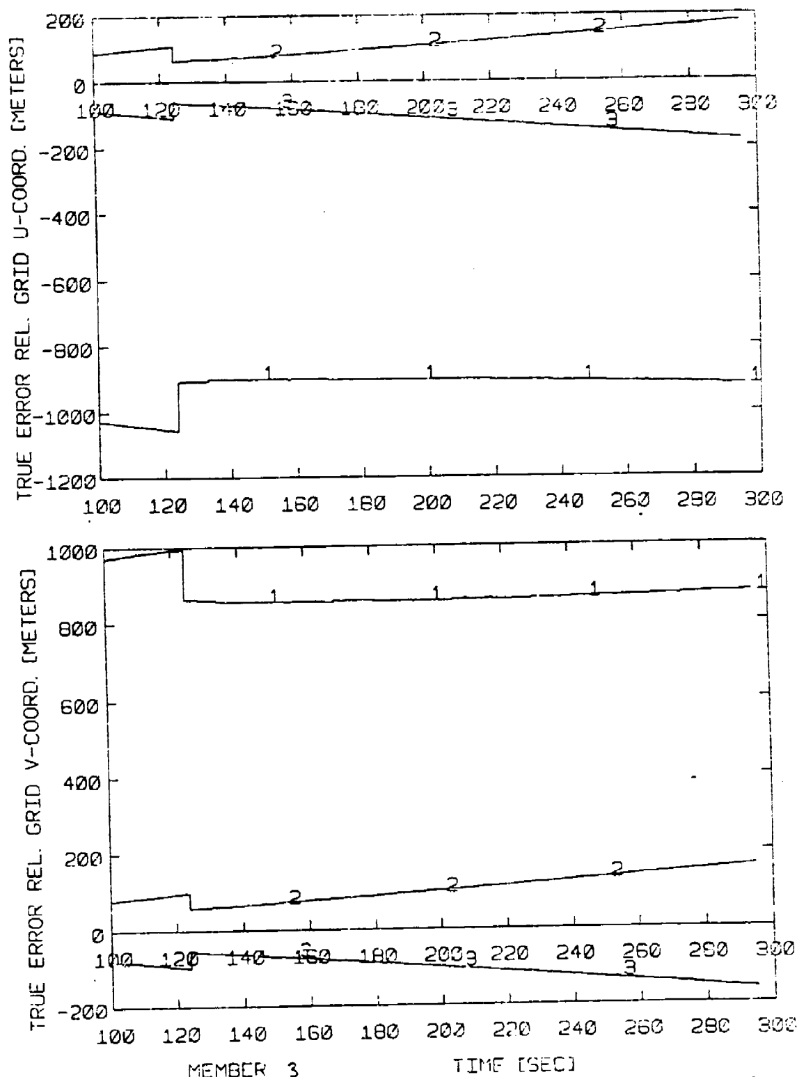
Fig. 7.29(b) Four Member Relnav Results, without Nonlinear Protection, and with More Accurate TOA Measurements (1m), Member 3, Expanded Scale
