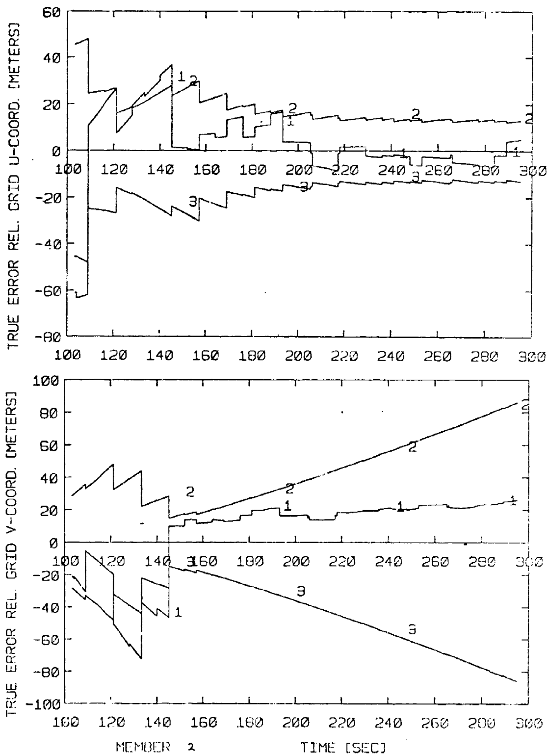
Fig. 7.6(b) Fly Around Trajectory, Relnav Results, Expanded Scale
