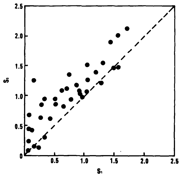
FIGURE 21. COMPARISON OF THE SENSITIVITIES OF THE SOOTING TENDENCY TO H/C RATIO FOR FUEL BLENDS CONTAINING POLYCYCLIC AROMATICS ( S_2 ) AND FUEL BLENDS CONTAINING MONOCYCLIC AROMATICS ( S_1 )
