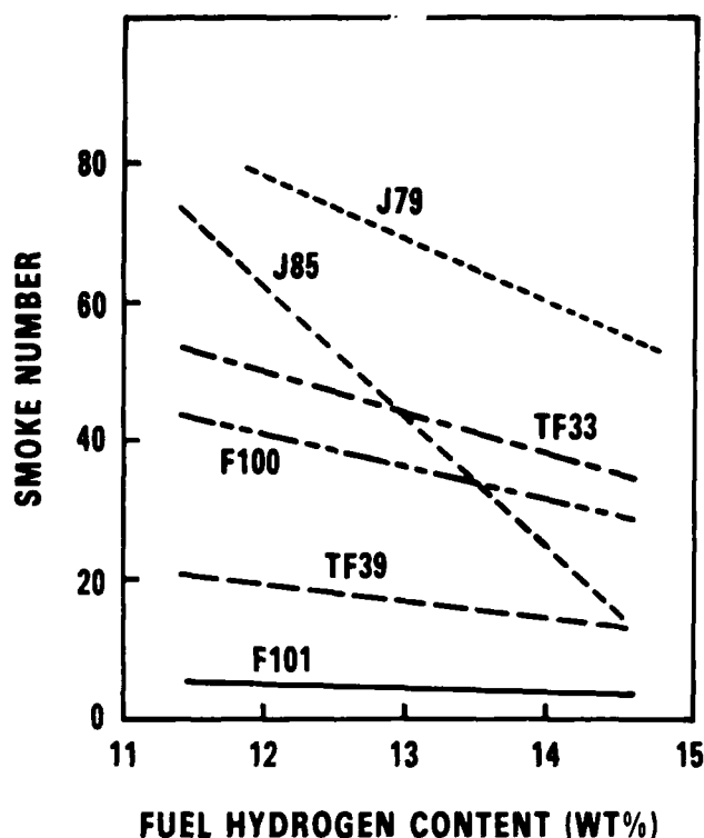
FIGURE 1. EFFECT OF FUEL HYDROGEN CONTENT ON EXHAUST SMOKE FROM ACTUAL ENGINES
