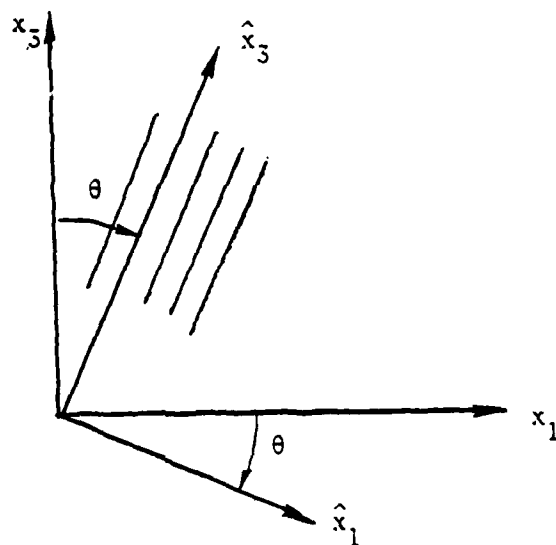
Fig. 3 Principal directions of an angle-ply laminate
