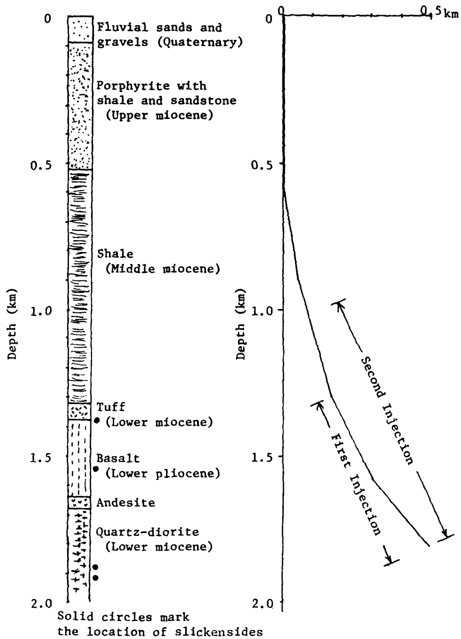
Figure 17. Log of injection borehole at Matsushiro (after Ohtake (1974))
