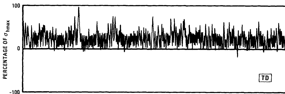
a. TENSION-DOMINATED SPECTRUM (WING ROOT)
