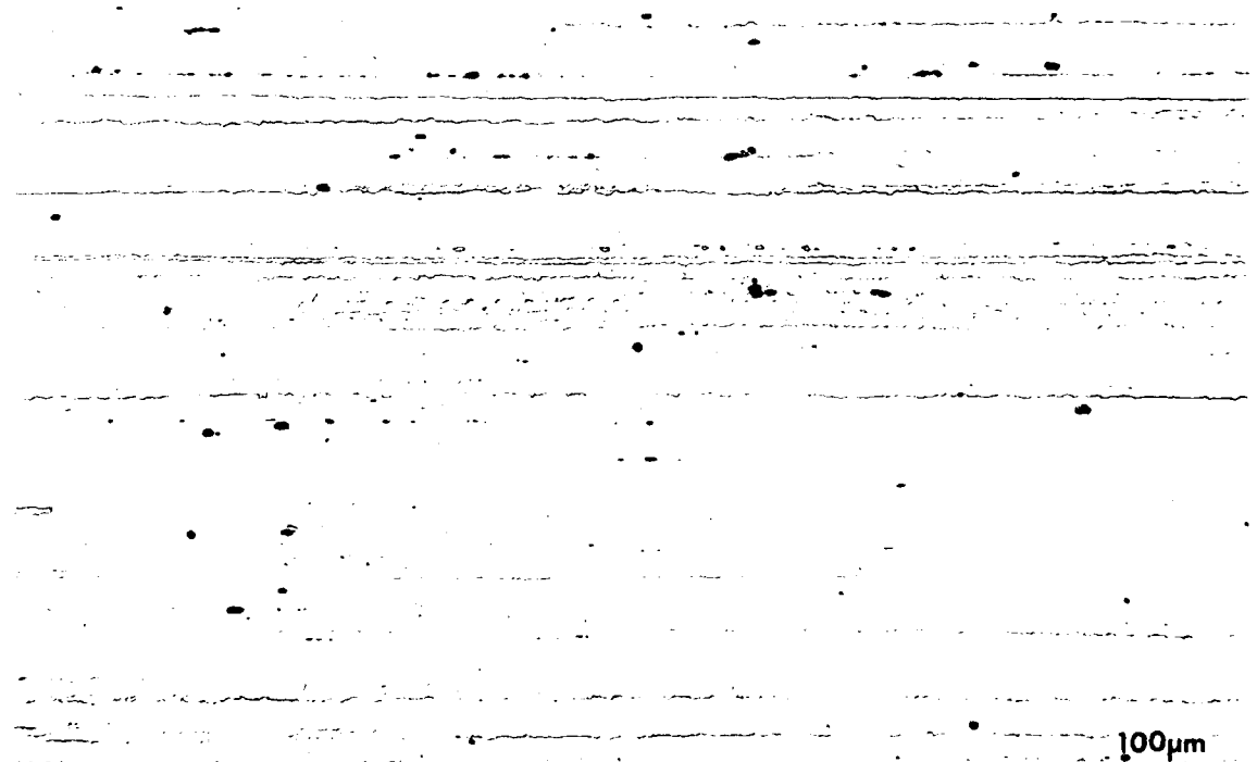
FIGURE 16. LONGITUDINAL MICROSTRUCTURE OF 7475-T651
