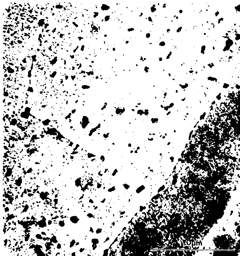
FIGURE 19. TEM MICROGRAPH OF 7075-T7351 PLATE SHOWING INCREASED PRECIPITATE SIZE OVER THE T6 TEMPER MATERIAL
