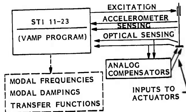
Fig. 3-32 Slim Beam Experiment Setup
