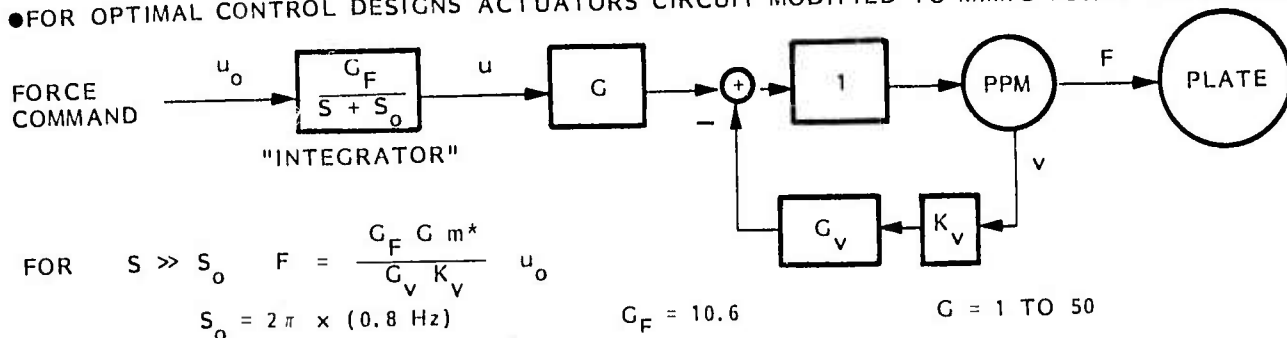
Fig. 3-43 Circular Plate PPM Actuator Compensation
