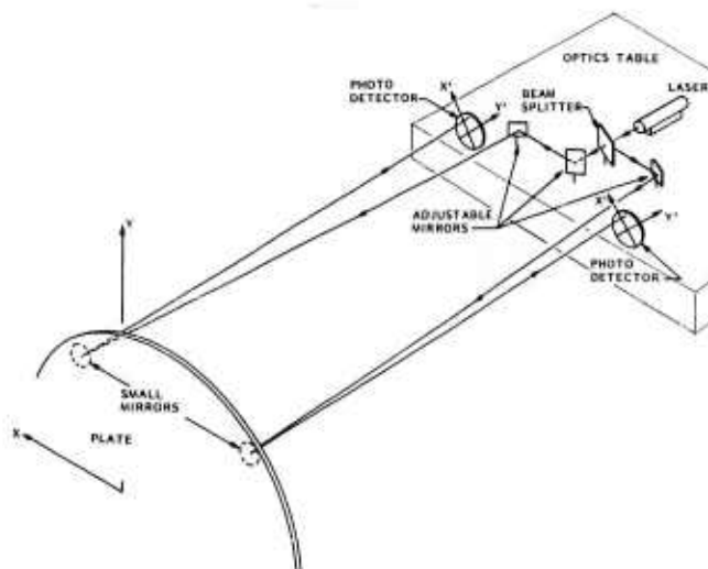
Fig. 3-41 Circular Plate Optical Sensing System
