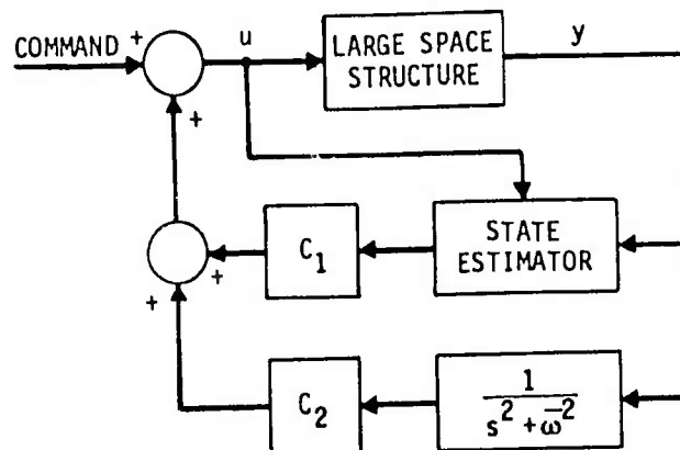
Fig. 4-6 A Frequency-Shaped Controller to Eliminate the Effect of Disturbance at \bar{\omega} on Output y
