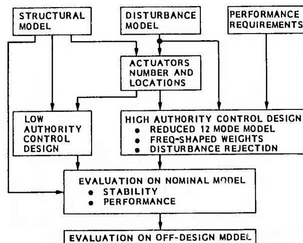
Fig. 4-13 Control Design Approach for Disturbance Rejection
