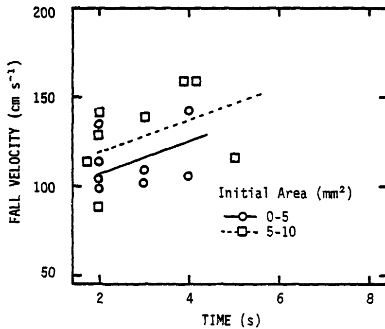
Fig. 6.3. Fall Velocity vs Time (at 4 °C, 90% RH)
