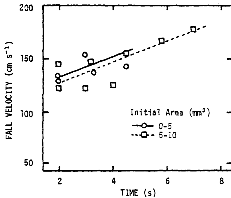
Fig. 6.4. Fall Velocity vs Time (at 4 °C, 100% RH)
