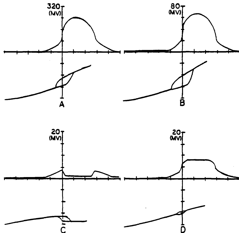
Figure 20. Output of the bistable device at various transverse locations.
