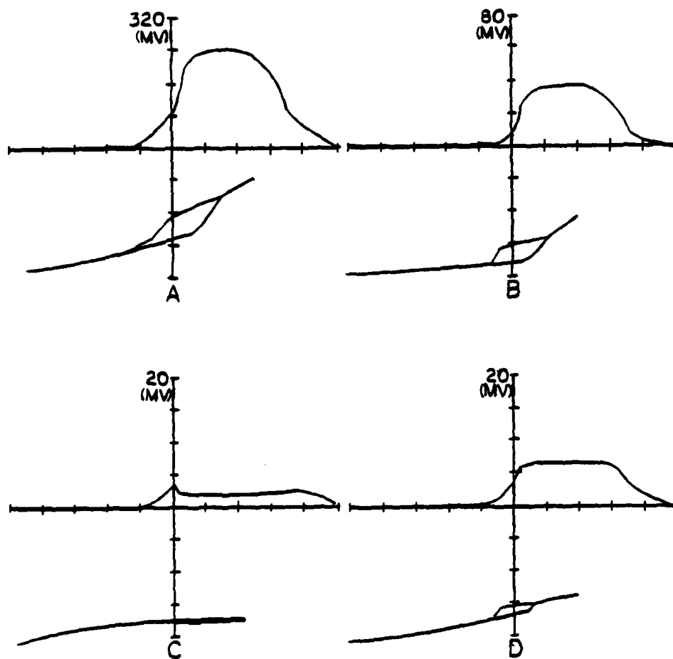
Figure 22. Output of device at various transverse points.
