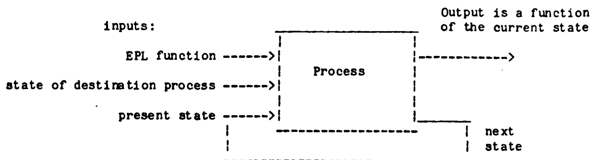
Figure 3.5 - Process as a finite state machine
