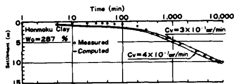
Fig.12 A typical example of curve fitting on self-weight consolidation process ( Honmoku clay )
