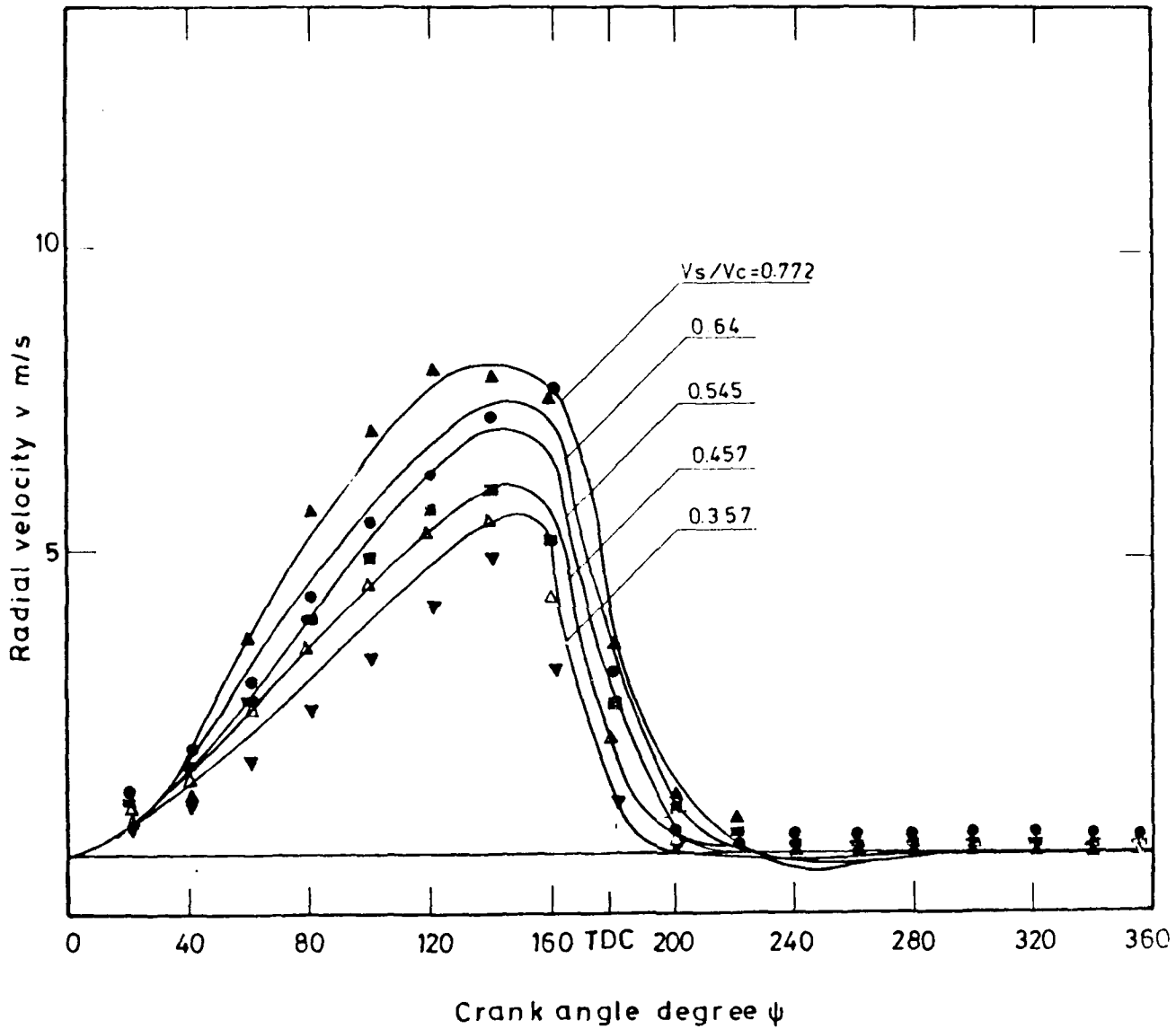
Fig( 46 ) Predicted and measured radial velocity in plane 4 at r/R_s=0.503 and various crank angles for different swirl volume ratios keeping A_j/A = 0.0092 and N = 1000 r.p.m constant.
