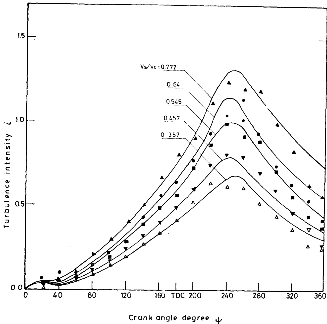
Fig ( 49) Predicted and measured turbulence intensity in plane 4 at r/R_s=0.503 during compression and expansion strokes for different swirl volume ratios keeping A_j/A=0.0092 and N=1000 r.p.m. constant.
