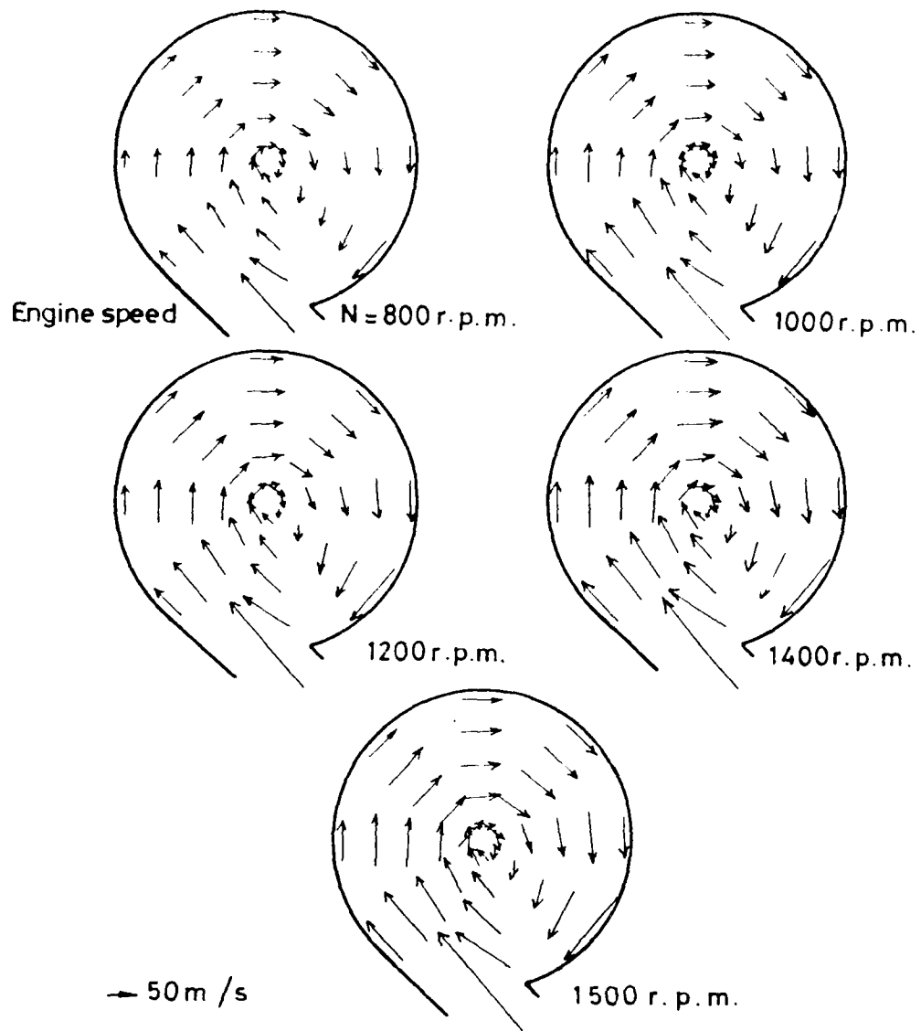
Fig( 50)Velocity vector plot for different engine speed at 20^\circ BTDC keeping V_s/V_c=0.772 And A_j/A=0.0092 constant.
