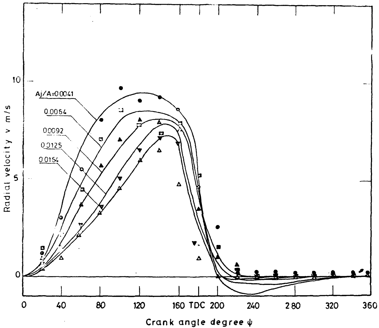
Fig ( 39 ) Predicted and measured radial velocity in plane 4 at r/R_s=0.503 and various crank angle for different port area ratios, keeping v_s/v_c=0.772 and N = 1000 r.p.m. constant.
