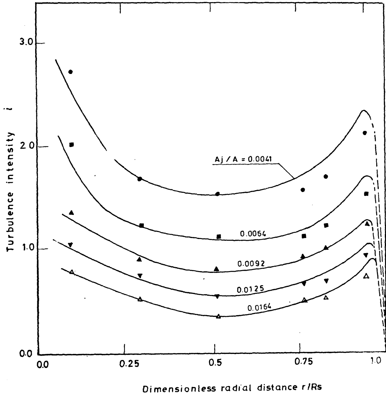
Fig(42 ) Predicted and measured turbulence intensity in plane 4 at TDC and various radii for different port area ratios keeping V_s/V_c = 0.772 and N = 1000 r.p.m constant.
