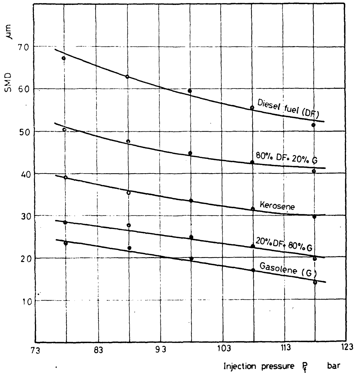
Fig( 29 ) Effect of injection pressure on Sauter mean diameter for clear and multifuel .
