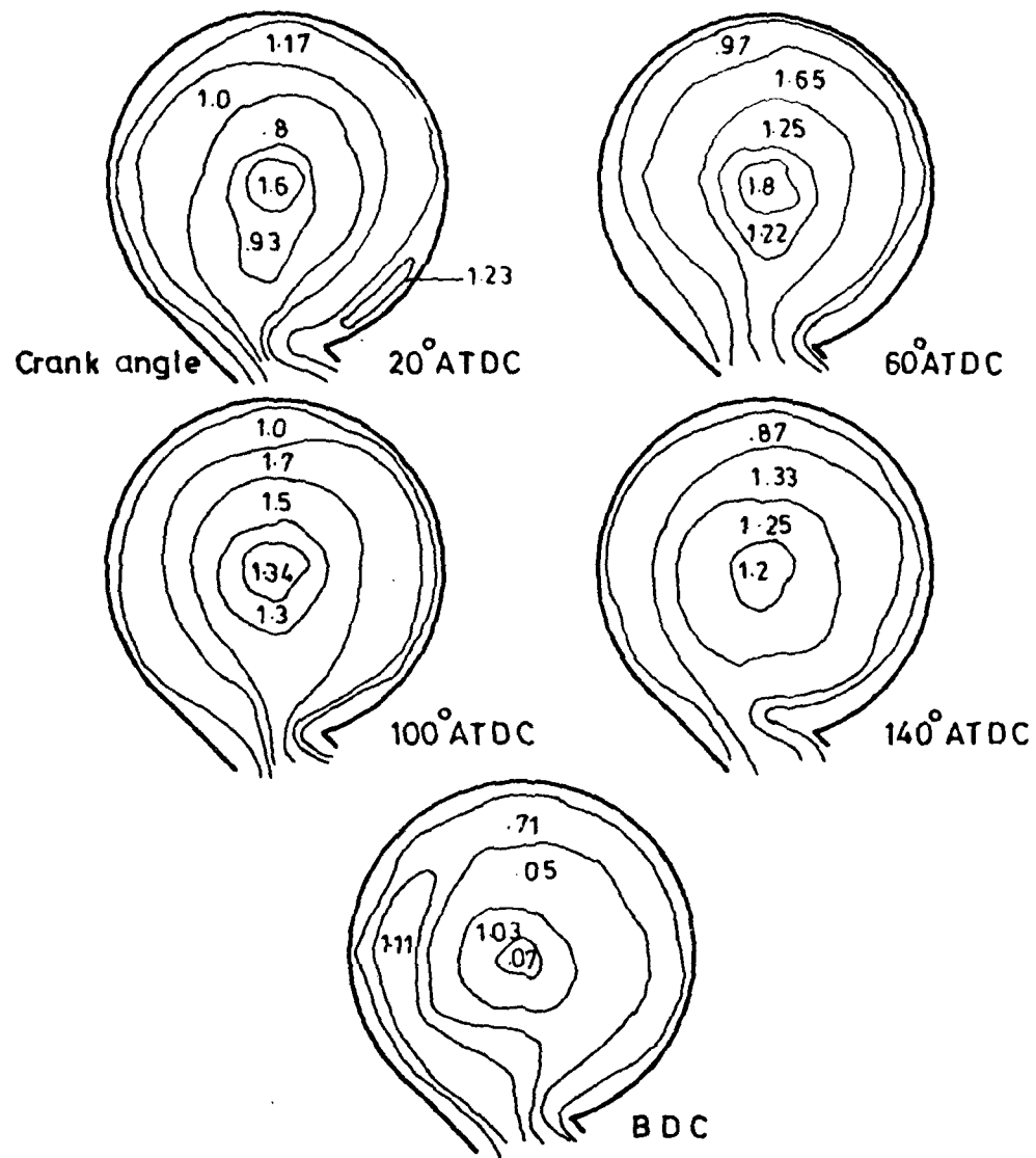
Fig( 33 )Turbulence intensity contours during expansion stroke keeping V_s/V_c=0.772 , A_j/A=0.0092 and N=1000 r.p.m constant.
