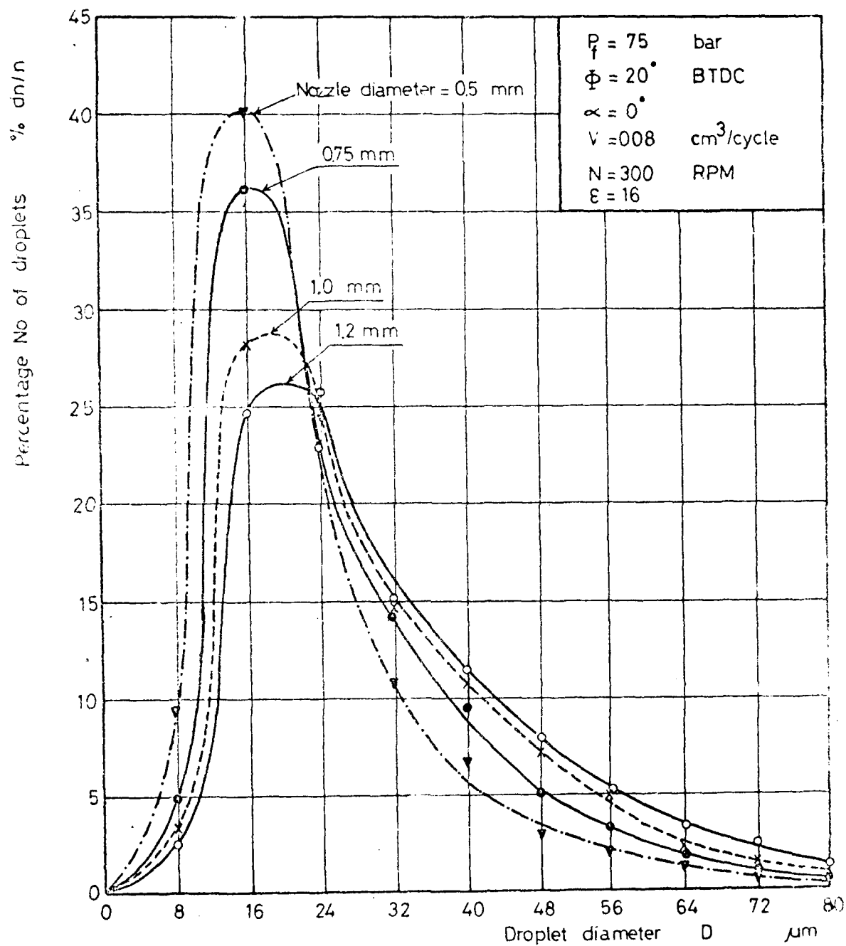
Fig( 27 ) Droplet size distribution for diesel fuel sprays inside a cold engine model for various nozzle diameters.
