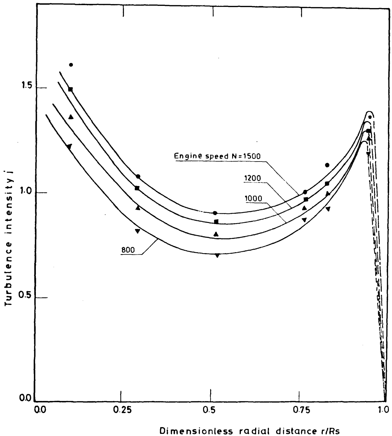
Fig( 56 ) Predicted and measured turbulence intensity at TDC in plane 4 for different radii and different engine speeds keeping V_s/V_c = 0.772 and A_j/A = 0.0092 constant.
