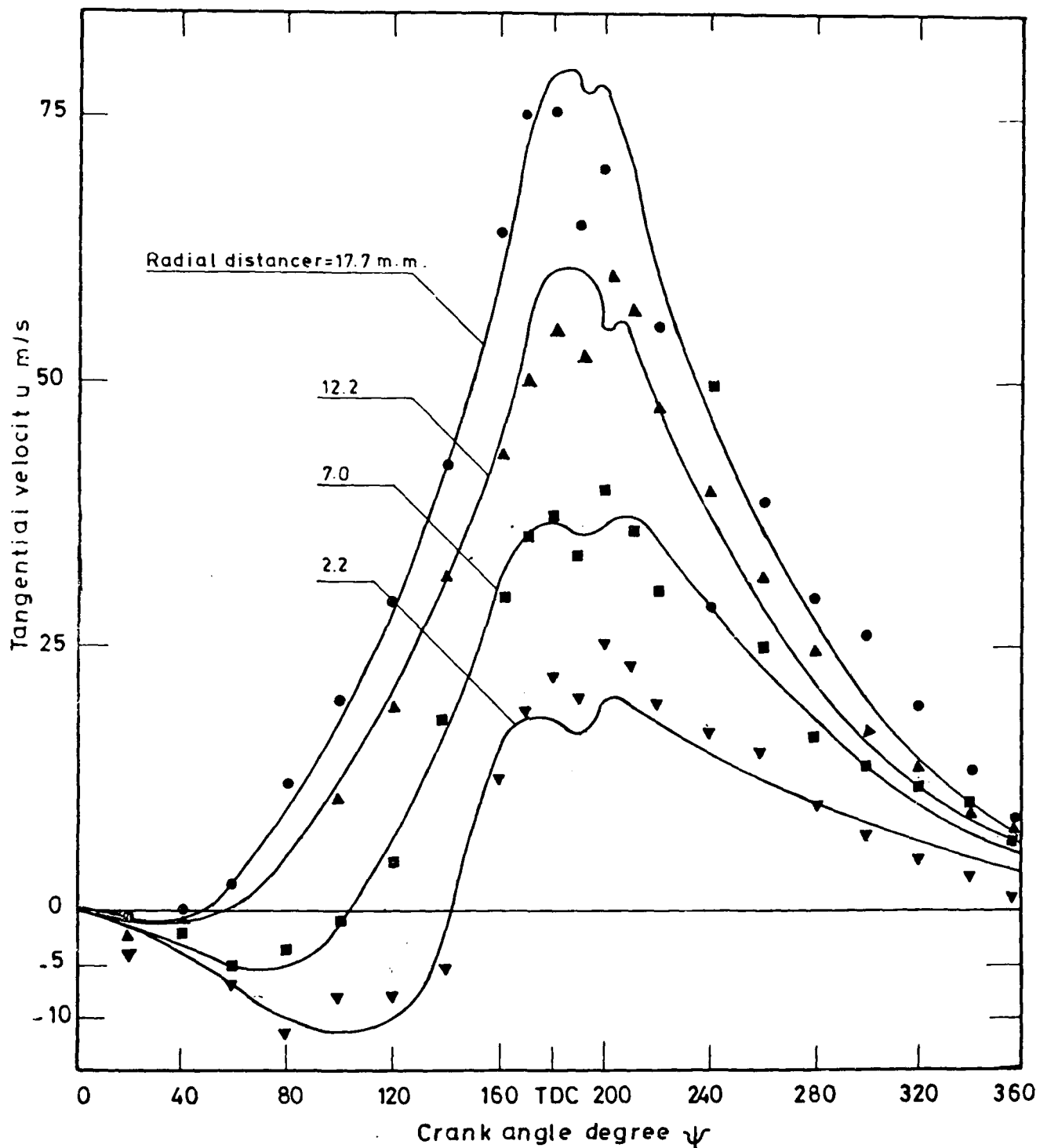
Fig( 28 ) Predicted and measured tangential velocity during compression and expansion strokes in plane 4 at various radii keeping V_s/V_c=0.772 , A_j/A=0.0092 and N=1000 r.p.m constant.
