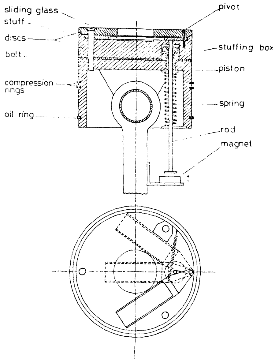
Fig(16) Slide sampling apparatus inside an operating piston .
