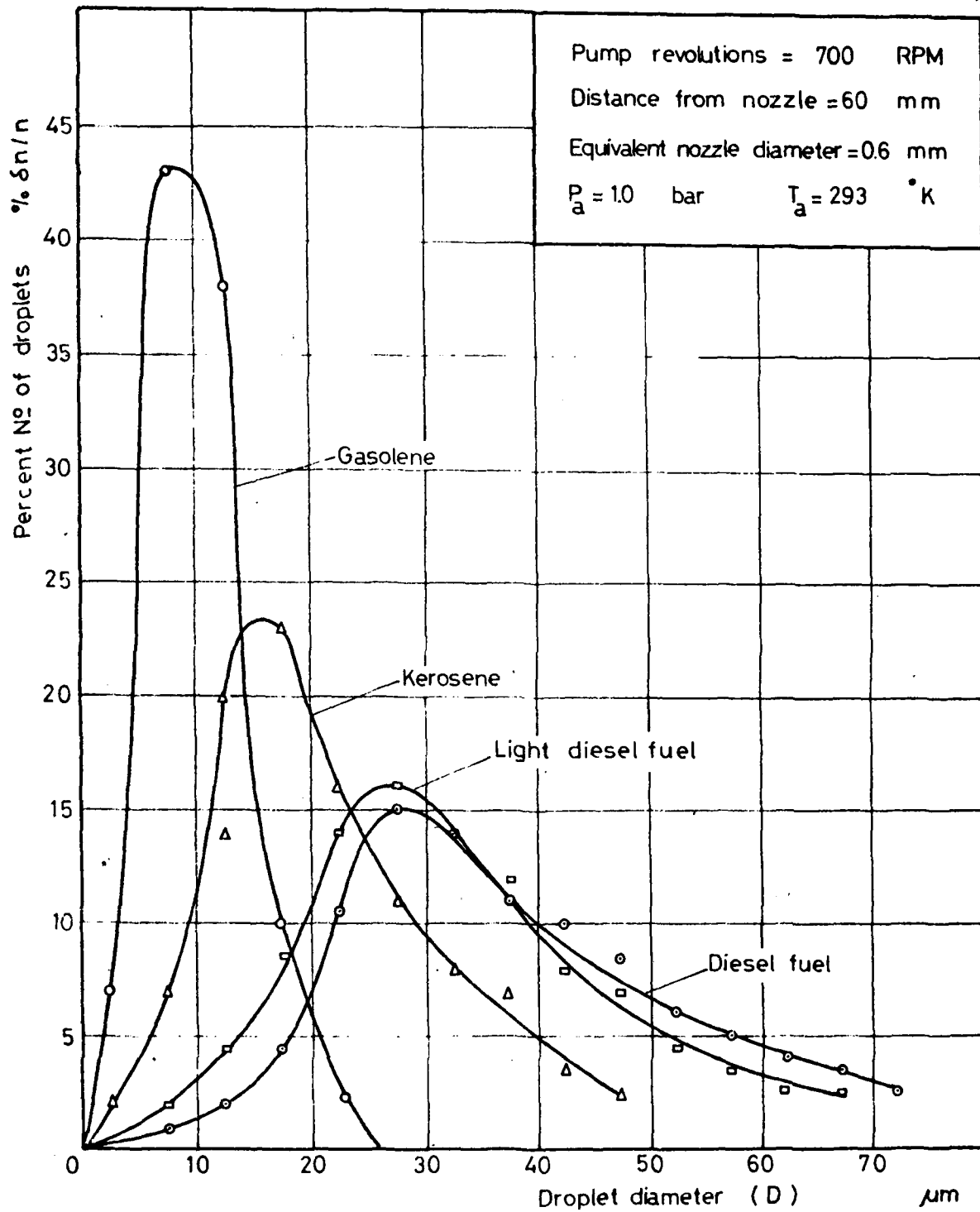
Fig(22) Droplet size distribution of clear fuel sprays injected by a pintle type injector with injection pressure 118 bar .
