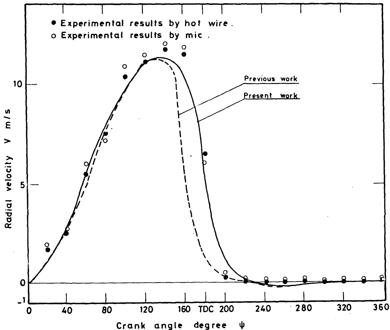
Fig.( 24 ) Comparison of predicted radial velocity by the suggested, and previous method [ ] during compression and expansion strokes with the experimental results at radial distance ratio 0.503 keeping V_s/V_c = 0.772 , A_j/A = 0.0092 and N = 1500 r. p. m. constant .
