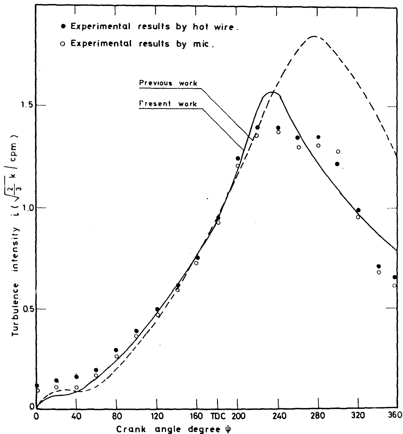
Fig. ( 22 ) Predicted and experimental variation of the turbulence intensity during compression and expansion strokes at radial distance ratio 0.503 keeping V_s/V_c = 0.772 , A_j/A = 0.0092 and N = 1500 r.p.m. constant.
