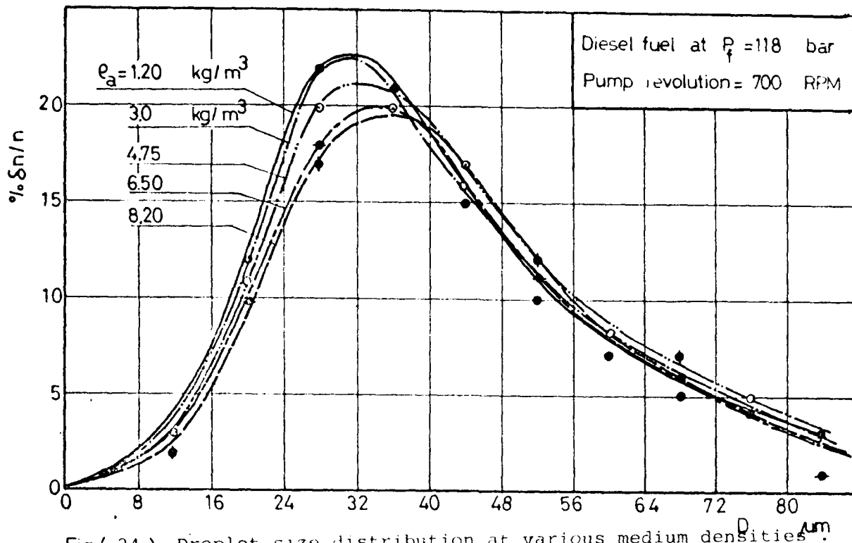
Fig ( 24 ) Droplet size distribution at various medium densities.
