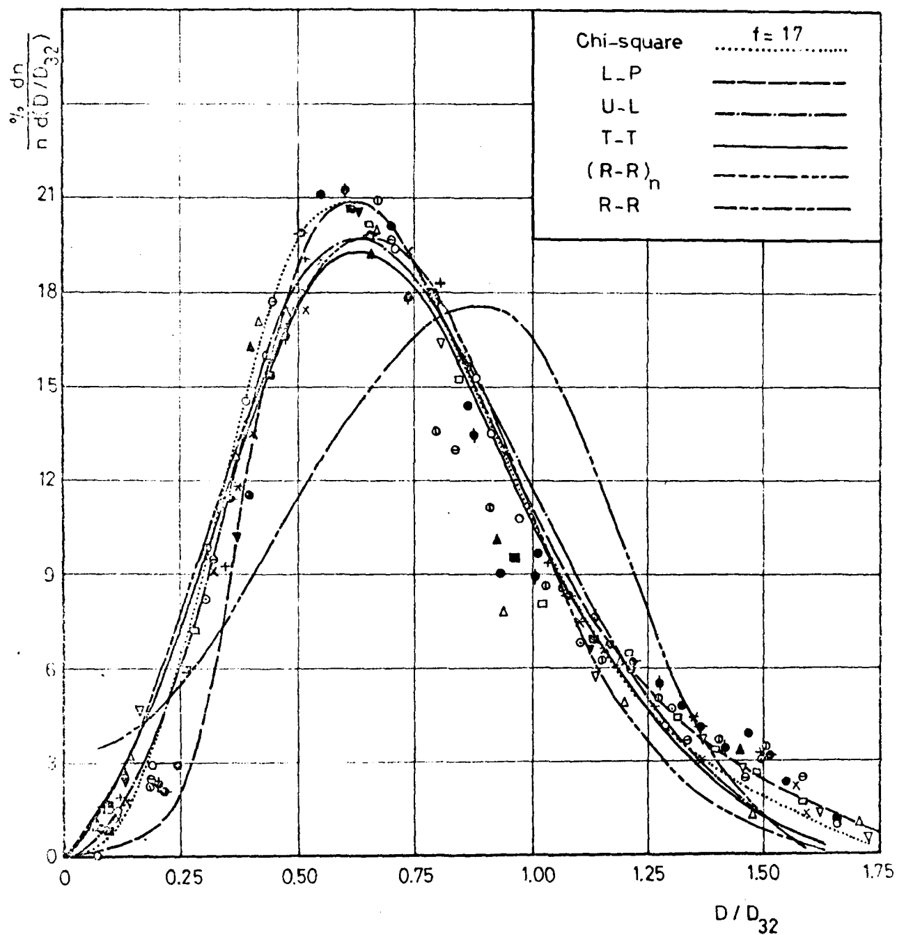
Fig ( 34 ) Comparison of various distribution equations with experimental values .
