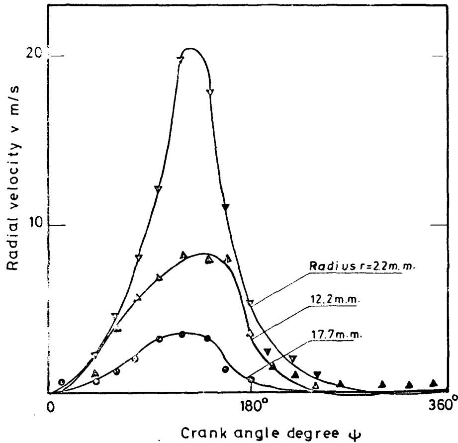
Fig( 30) Predicted and measured radial velocity during compression and expansion strokes in plane 4 at various radii, keeping V_s/V_c = 0.772 , A_j/A = 0.0092 and N = 1000 r.p.m. constant.
