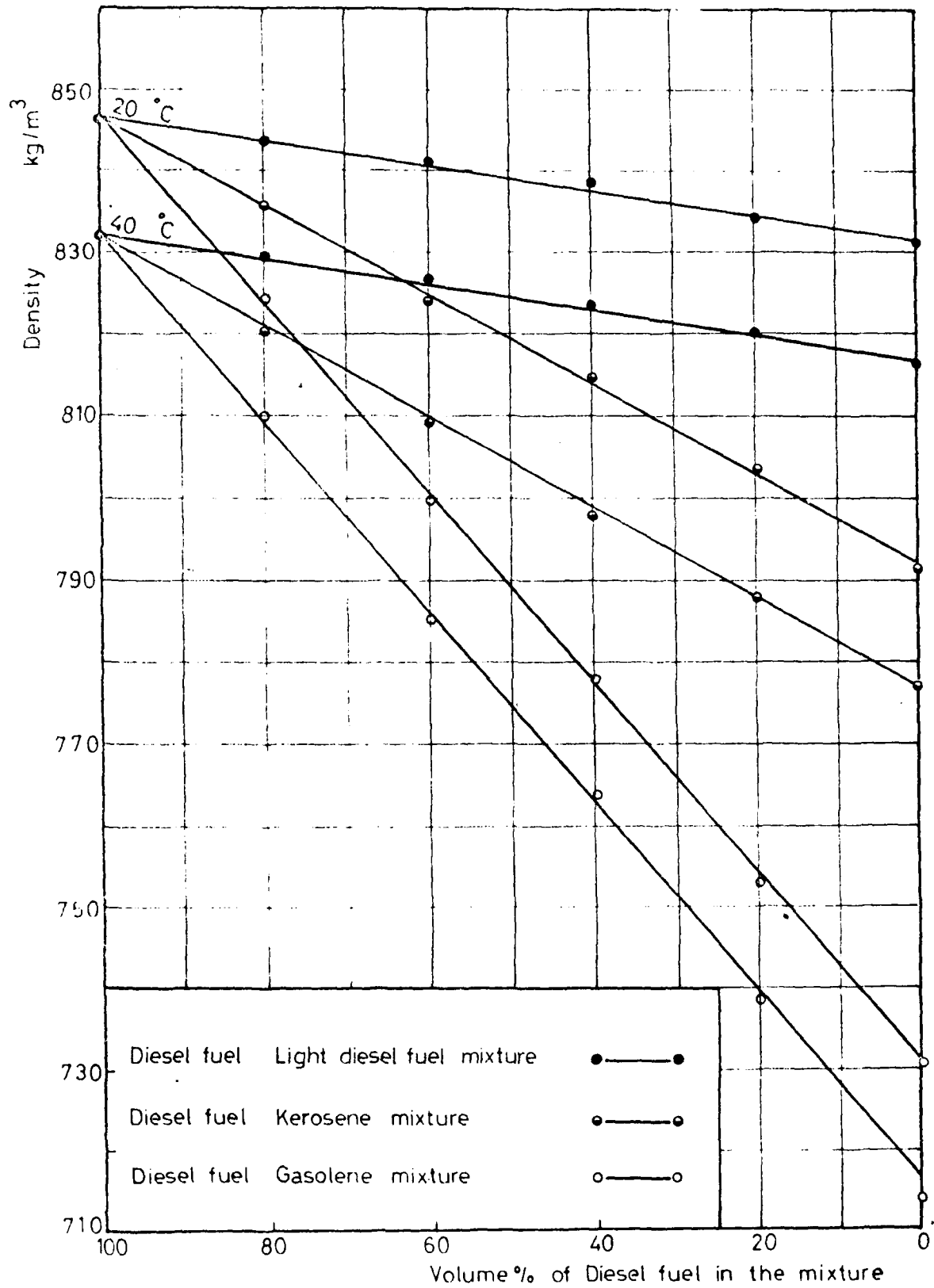
Fig(19) Nature of density variation for various blend mixtures .
