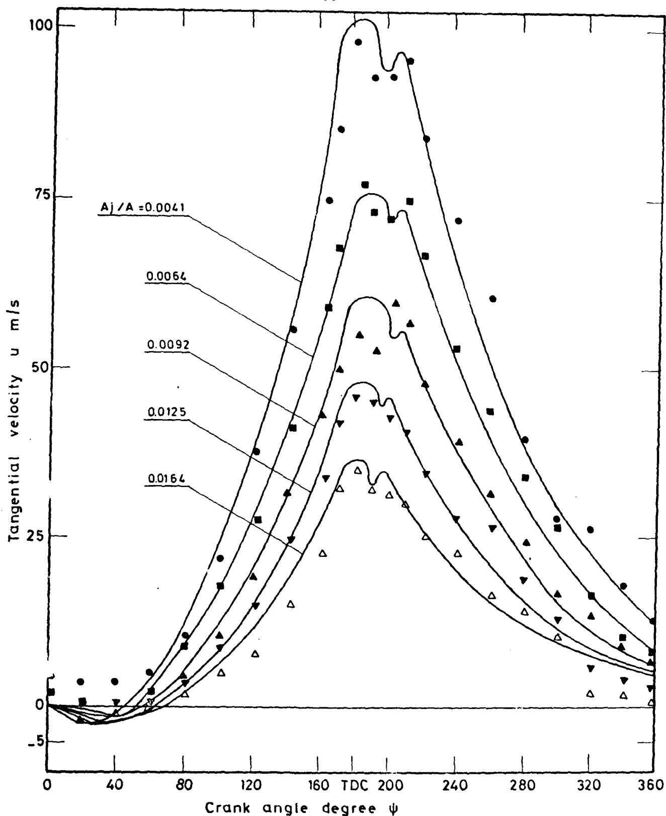
Fig.(37 )Predicted and measured tangential velocity during compressor and expansion strokes in plane 4 for different port area ratios keeping V_s/V_c=0.772 and N=1000 r.p.m. constant.
