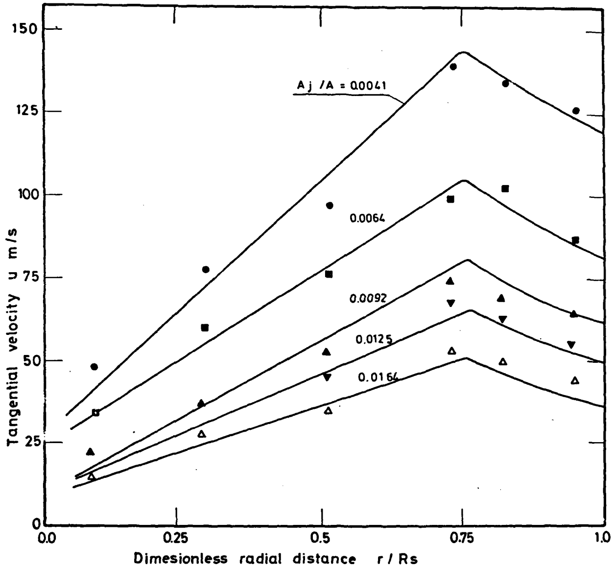
Fig.( 38 ) Predicted and measured tangential velocity in plane 4 at TDC and various radii for different port area ratios keeping V_s/V_c = 0.772 and N = 1000 r.p.m. constant.
