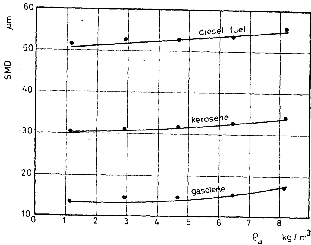
Fig( 30 ) Effect of medium density on Sauter mean diameter for clear fuel at injection pressure bar
