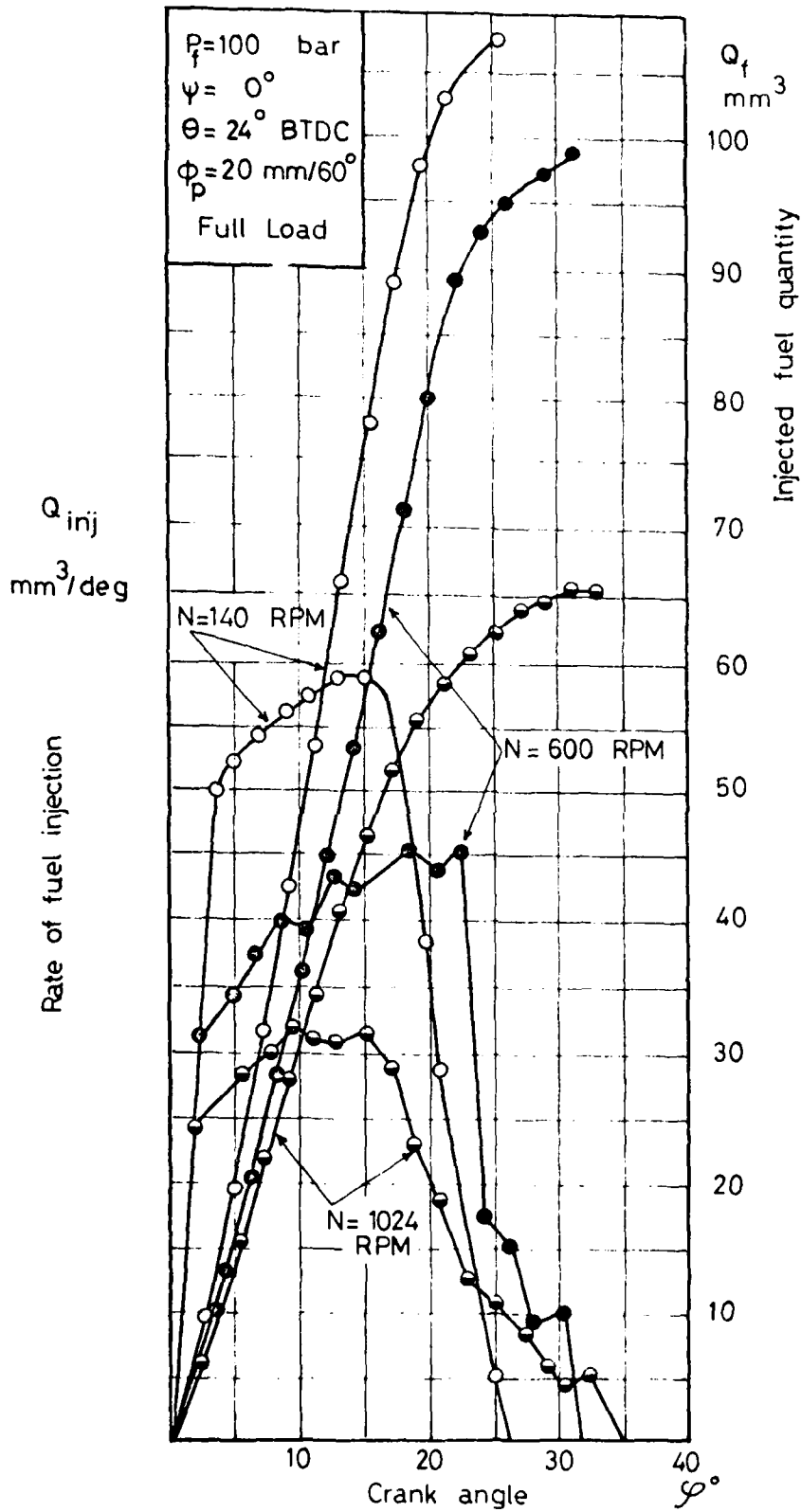
Fig( 2 ) The fuel delivery law and injection law at various engine speeds
