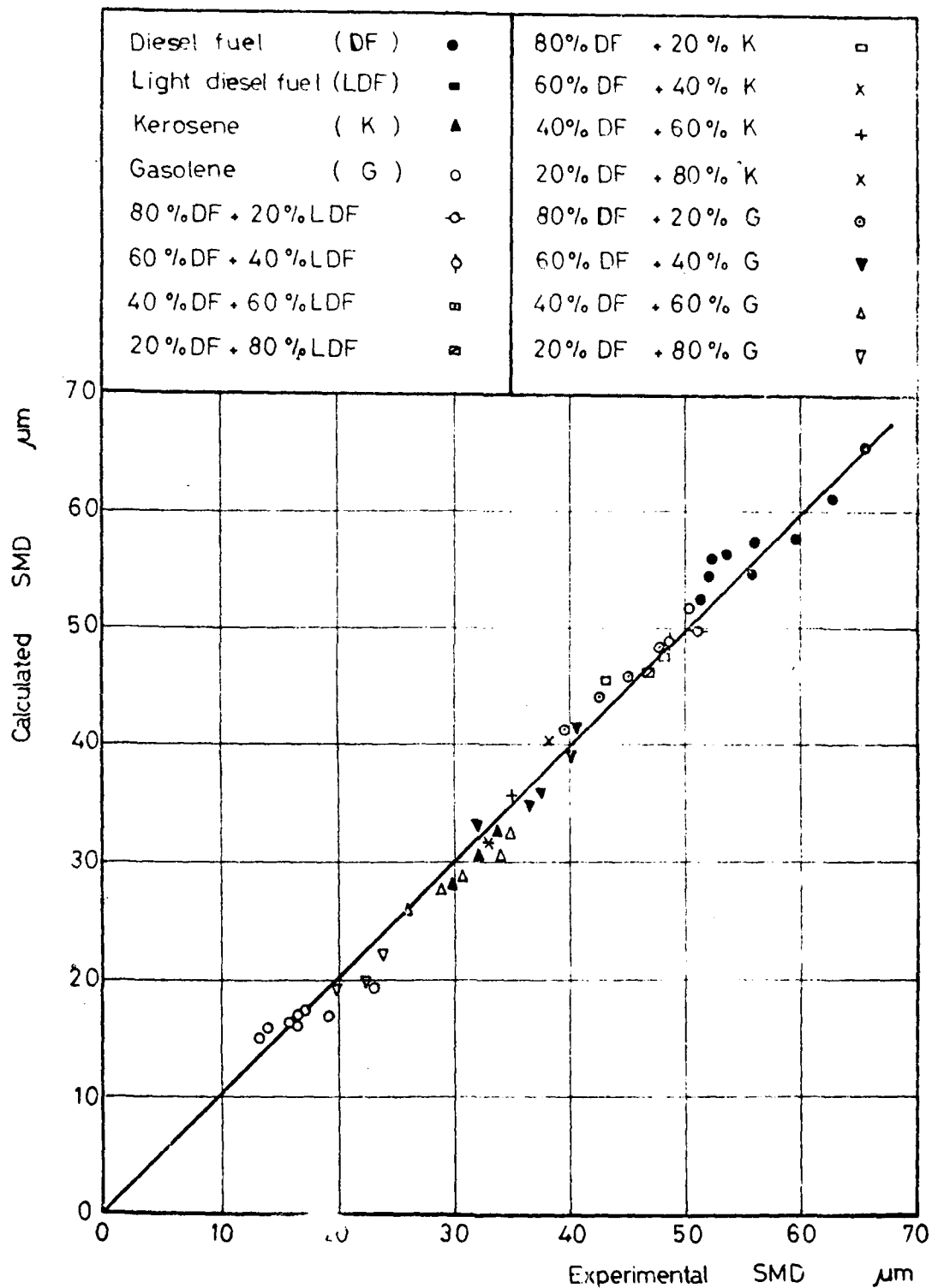
Fig(36 ) Comparison of calculated and experimental values of Sauter mean diameter .
