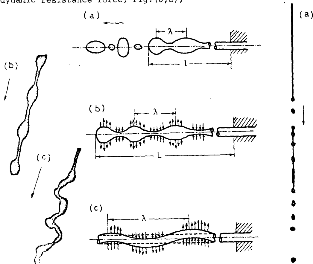
Fig. ( 8 ) Characteristics of the first three regimes of atomization .
