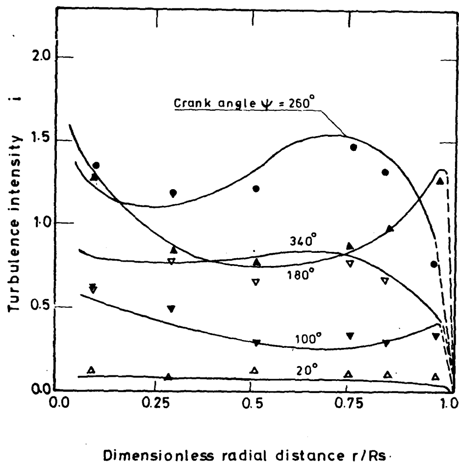
Fig ( 35 ) predicted and measured turbulence intensity in plane 4 at various radii and different crank angles keeping V_s/V_c = 0.772 , A_j / A = 0.0092 and N = 1000 r.p.m. constant.
