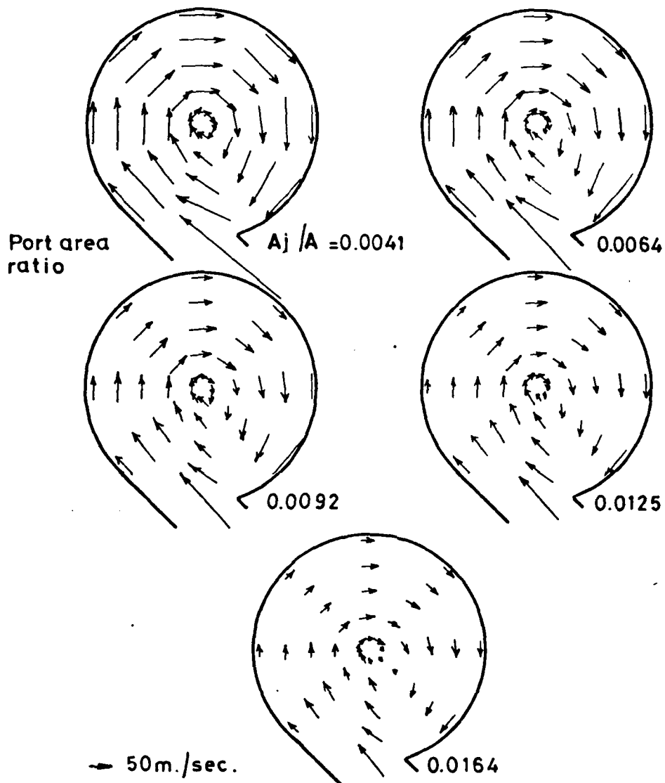
Fig. (36) Velocity vector plot for different port area ratios at 20^\circ BTDC keeping V_s/V_c = 0.772 and N = 1000 r.p.m constant.
