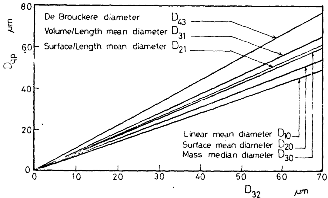
Fig( 31 ) Comparison between Sauter mean diameter D_{32} and other mean diameters.
