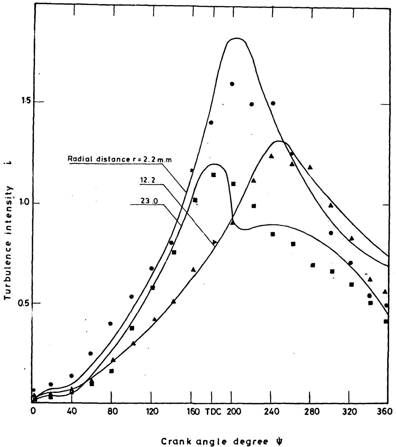
Fig(34) Predicted and measured turbulence intensity during compression and expansion strokes in plane 4 at various radii keeping V_s/V_c = 0.772 A_j/A = 0.0092 and N = 1000 \text{ r.p.m.} constant.
