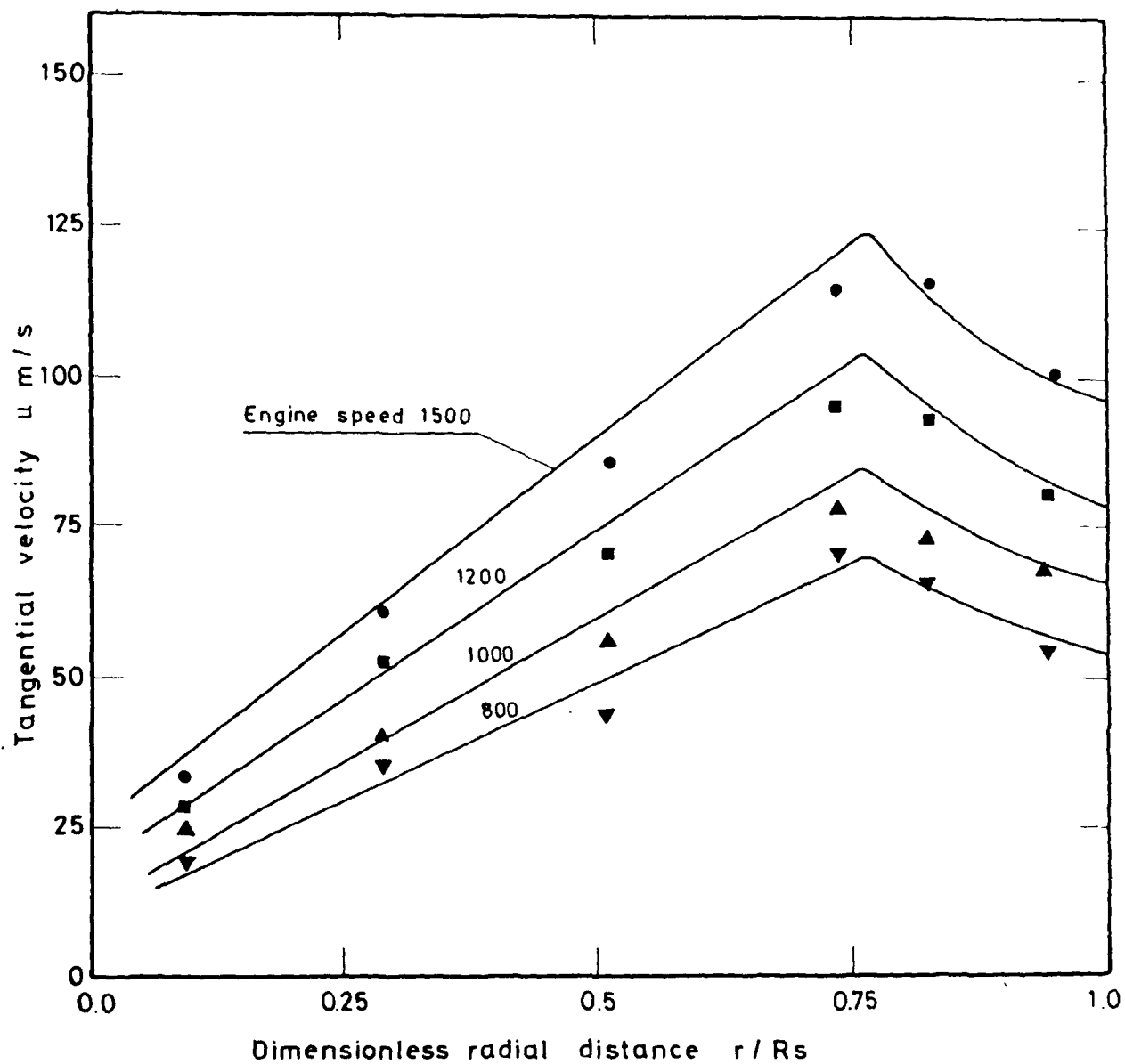
Fig.(52 ) Predicted and measured tangential velocity in plane 4 at TDC for different engine speeds keeping V_s/V_c = 0.772 and A_j/A = 0.0092 constant.
