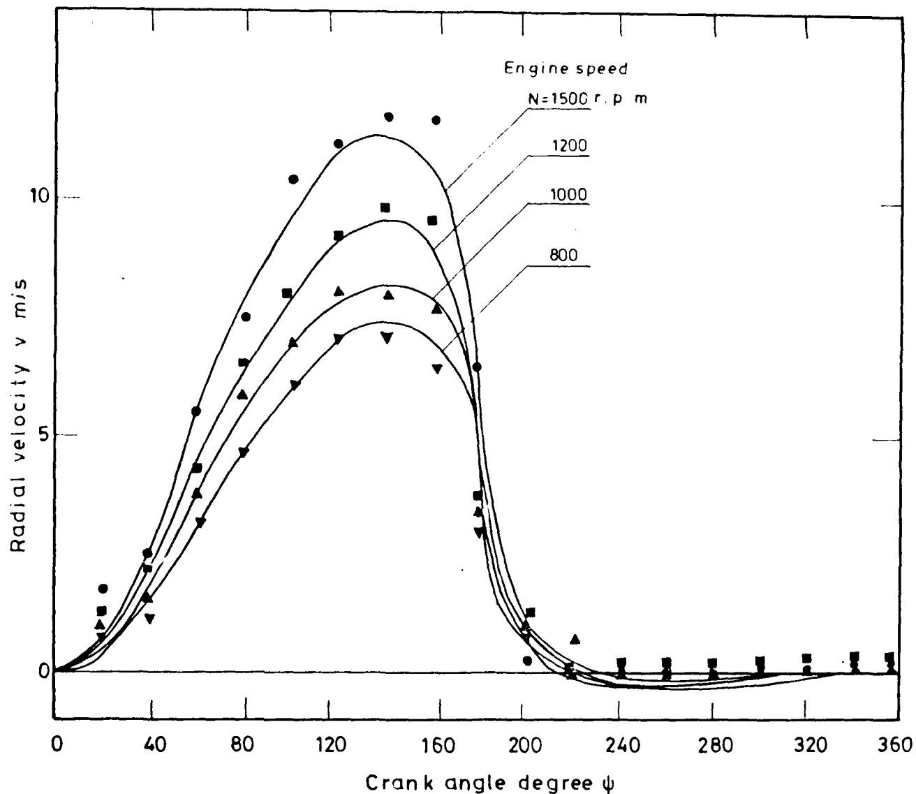
Fig ( 53) Predicted and measured radial velocity at plane 4 and r/R_s = 0.503 during compression and expansion strokes at various engine speeds keeping V_s/V_c = 0.772 and A_j/A = 0.0092 constant.
