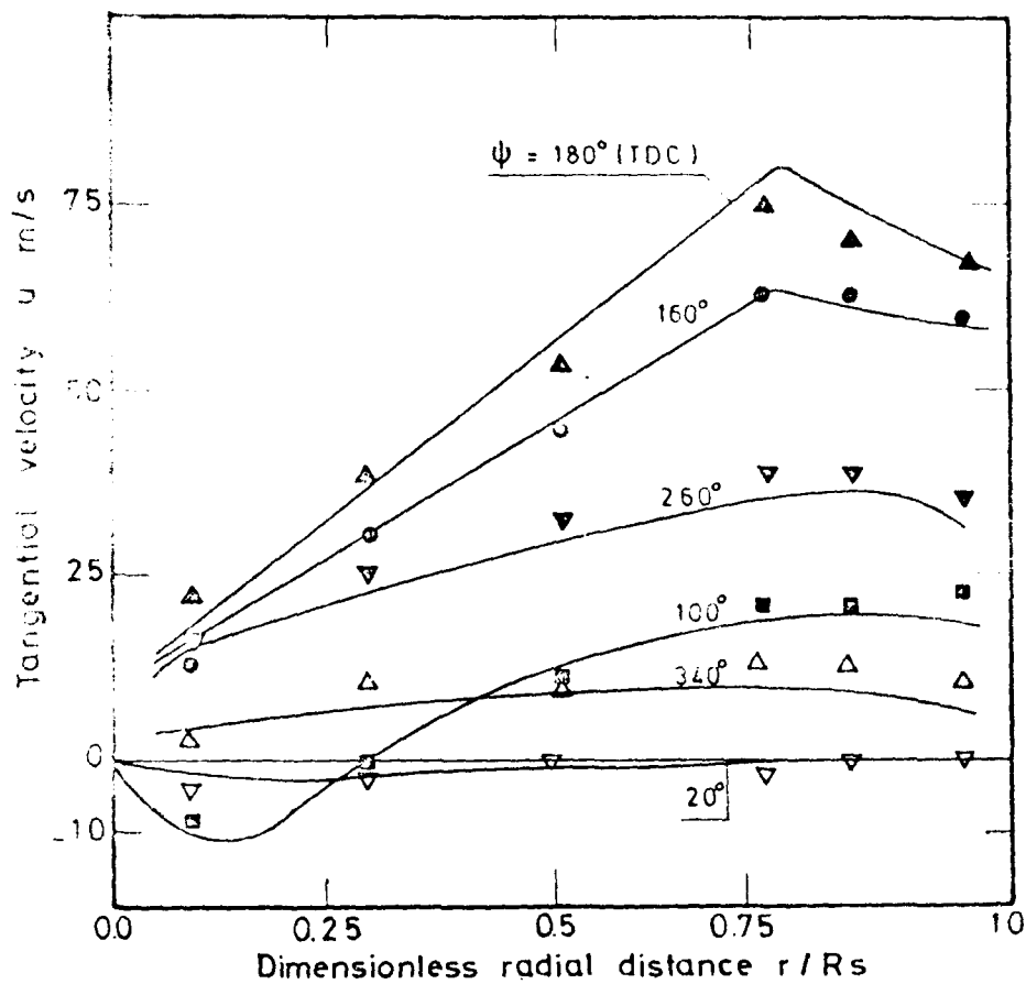
Fig.(29) Predicted and measured tangential velocity in plane 4 at various radii at different crank angles, keeping V_s/V_c=0.772 , A_j/A=0.0092 and N=1000 r.p.m. constant.
