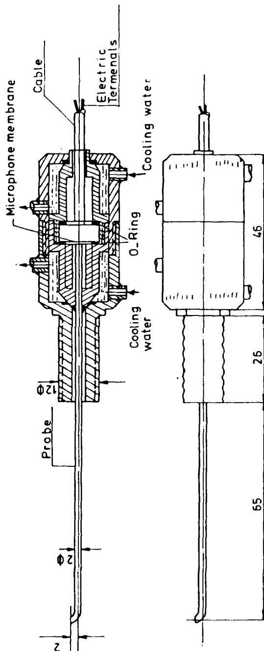
Fig ( 5 ) Condenser microphone measuring probe
