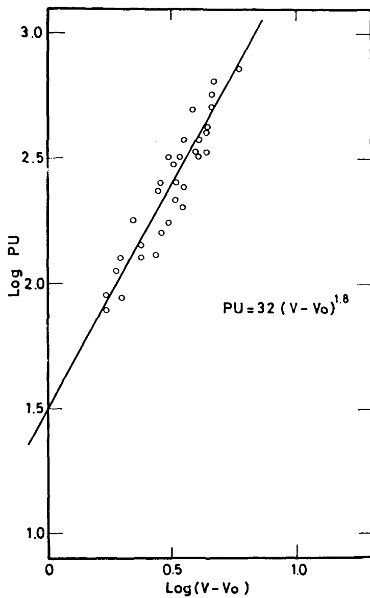
Fig.( 8 ) Determination of hot-wire calibration constants
