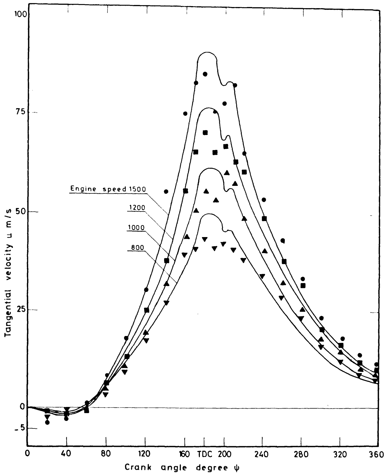
Fig.( 51 ) Predicted and measured tangential velocity during compression and expansion strokes in plane 4 for r/R_s = 0.503 at various engine speeds keeping V_s/V_c = 0.772 and A_j/A = 0.0092 constant .
