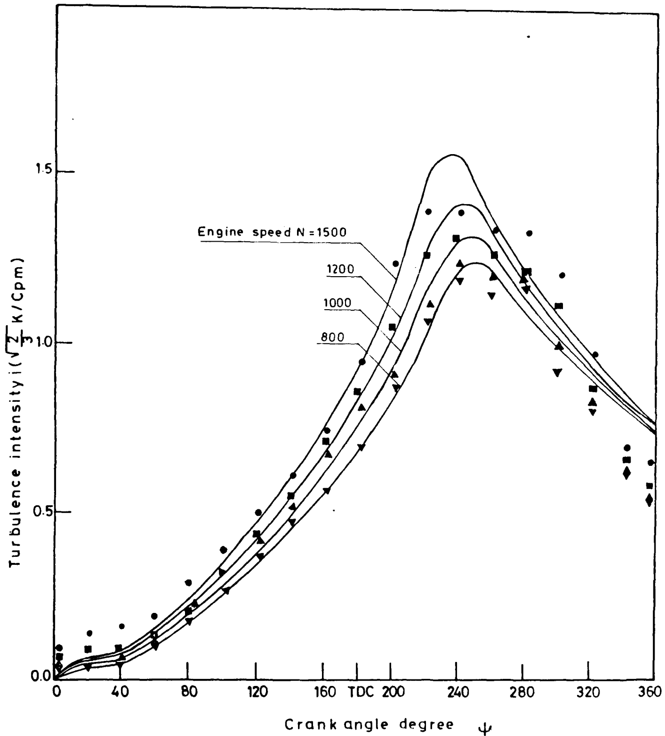
Fig( 55) Predicted and measured turbulence intensity at r/R_s = 0.503 in plane 4 for various crank angles and different engine speeds keeping V_s/V_c = 0.772 and A_j/A = 0.0092 constant
