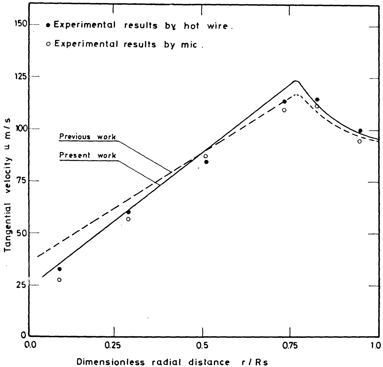
Fig.(19 )Comparison of predicted tangential velocity by the suggested and previous method [ ] along the radius with the experimental results at TDC keeping V_s/V_c=0.772 , A_j/A=0.0092 and N=1500 r.p.m. constant.
