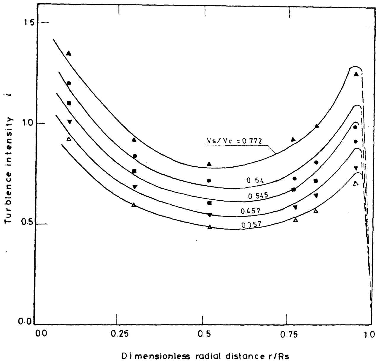
Fig.( 48 ) Predicted and measured turbulence intensity in plan 4 at TDC and various radii for different swirl volume ratios keeping A_j/A = 0.0092 and N = 1000 r.p.m. constant.
