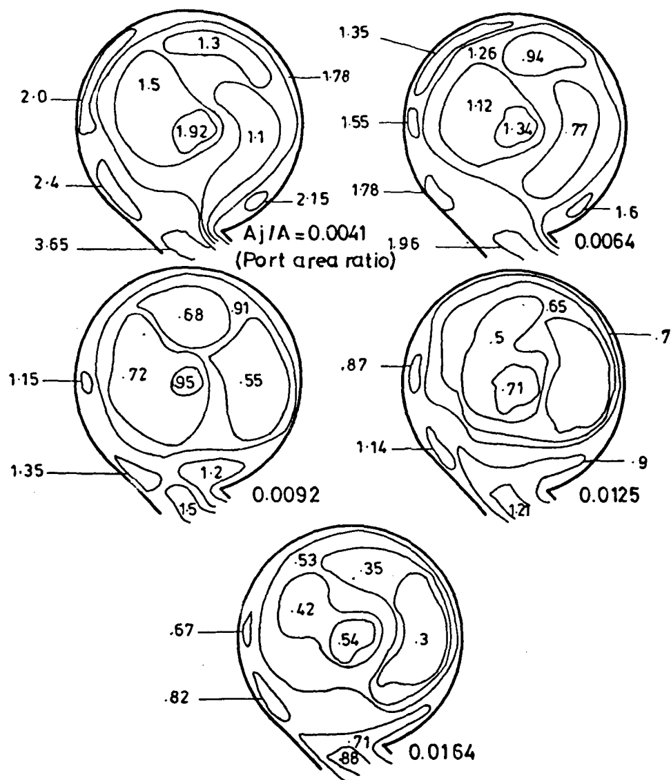
Fig ( 40 ) Turbulence intensity contours for different part area ratios at 20^\circ BTDC keeping V_s/V_c = 0.772 and N = 1000 r.p.m constant
