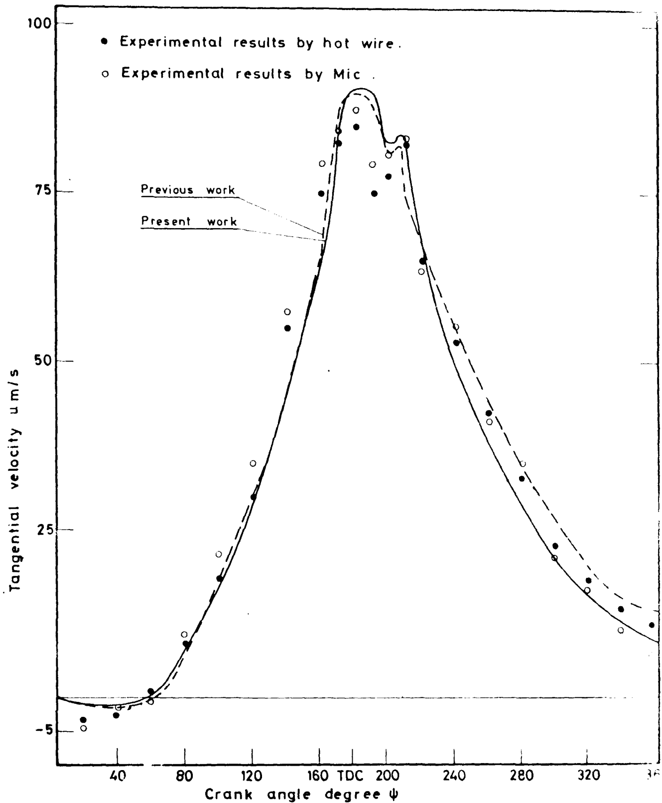
Fig.( 20 ) Comparison of predicted tangential velocity by the suggested and previous method [ 1 ] during compression and expansion strokes with the experimental results at radial distance ratio 0.503 keeping V_s/V_c = 0.772 , A_j/A = 0.0092 and N = 1500 r.p.m. constant.
