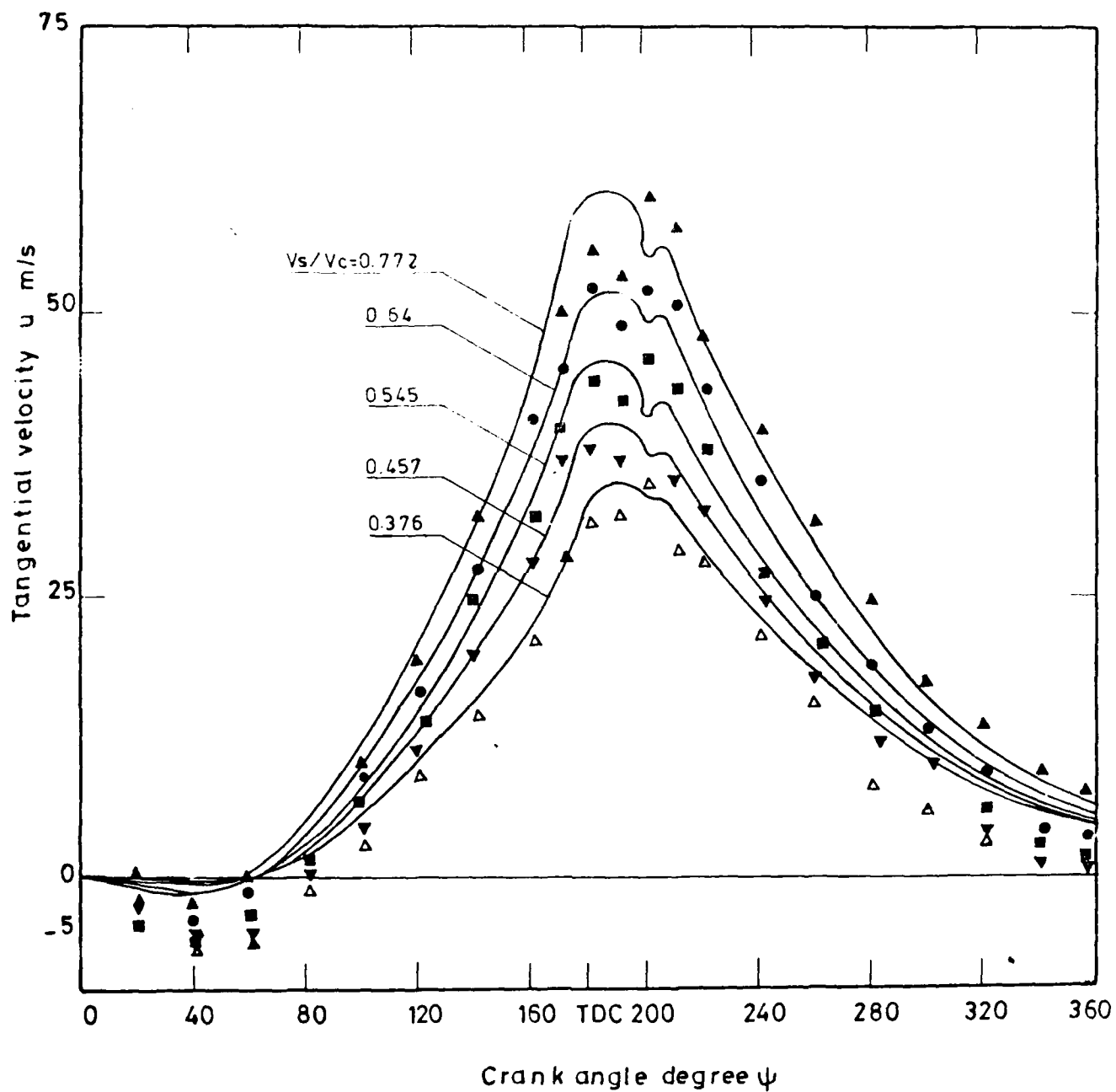
Fig.(44) Predicted and measured tangential velocity during compression and expansion strokes in plane 4 at r/R_s = 0.503 for different swirl volume ratios keeping A_j/A = 0.0092 and N = 1000 r.p.m. constant.
