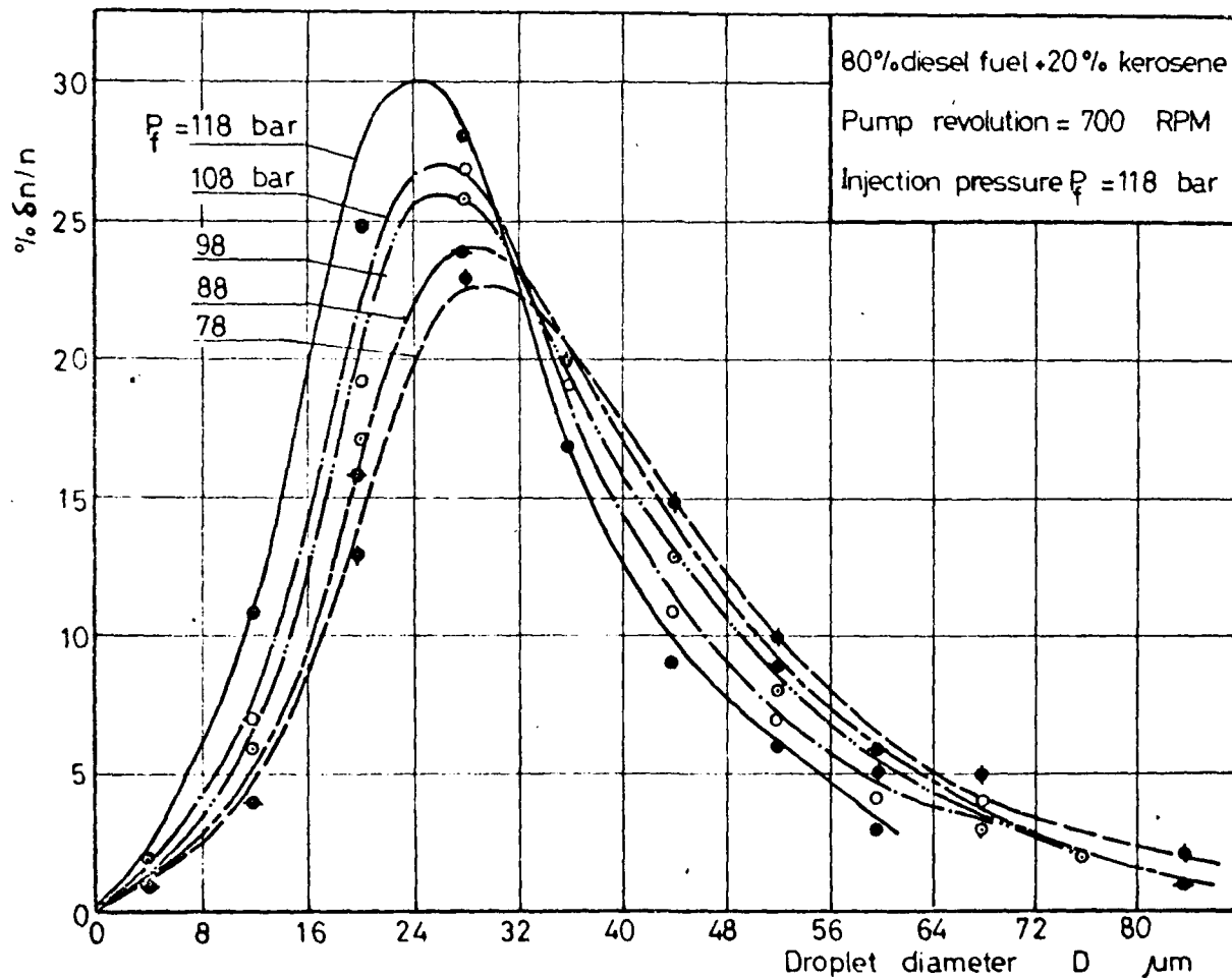
Fig( 25 ) Droplet size distribution at various injection pressures .
