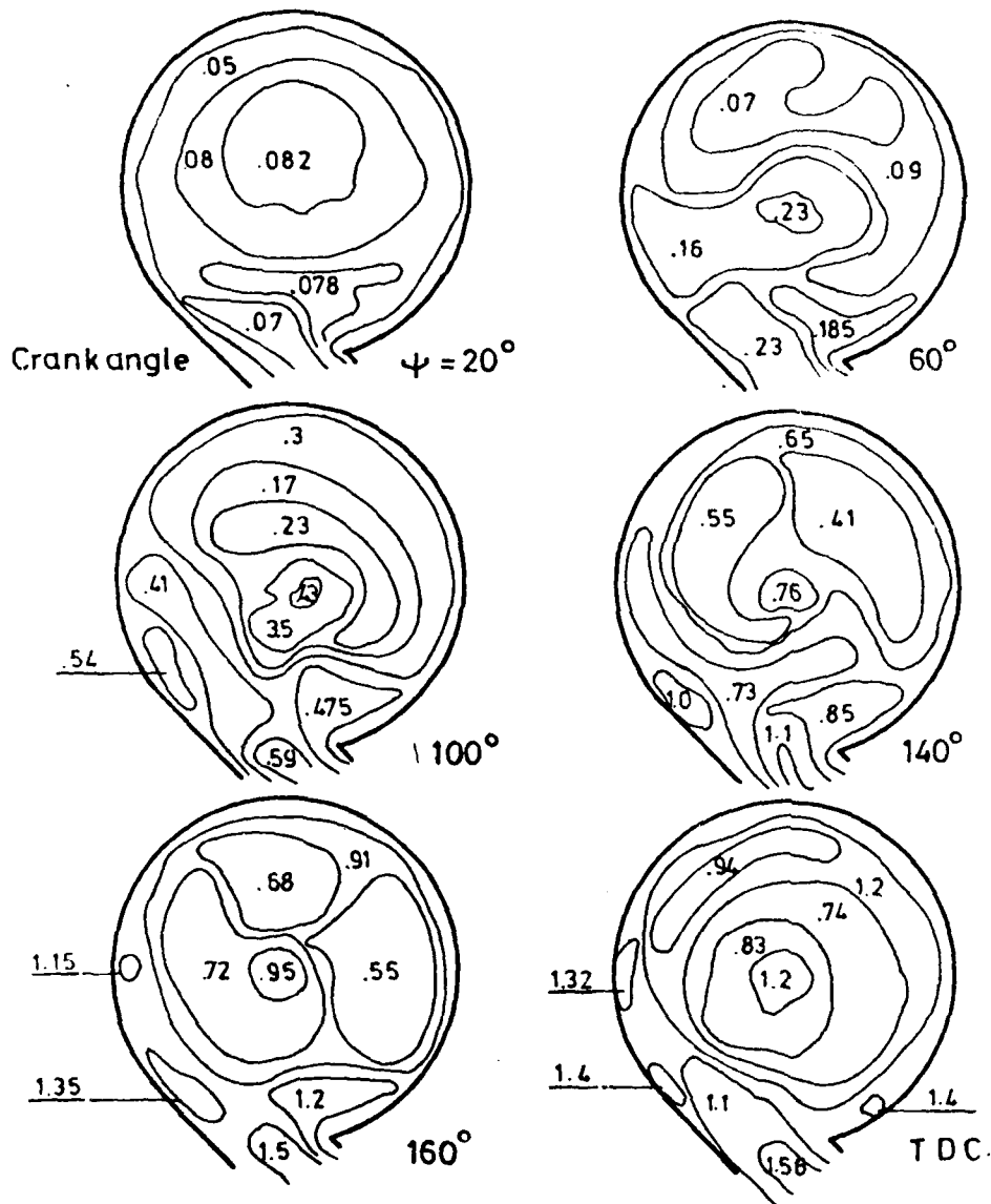
Fig.(32 )Turbulence intensity contours during compression stroke keeping V_s/V_c=0.772 , A_j/A=0.0092 and N=1000 , \mu m constant.
