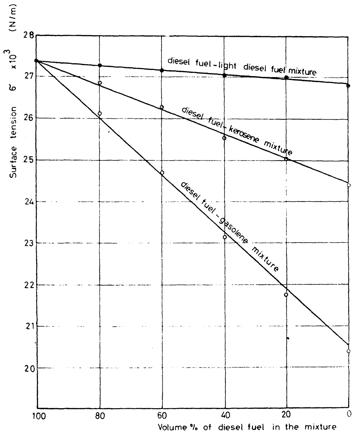
Fig(18 ) Nature of surface tension variation for various blend mixtures .
