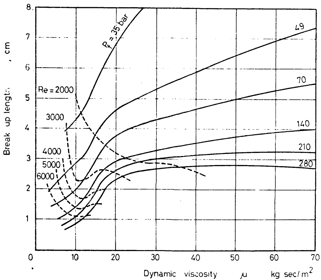
Fig( 10 ) Effect of kinematic viscosity of fuel on the break up length for various injection pressures .
