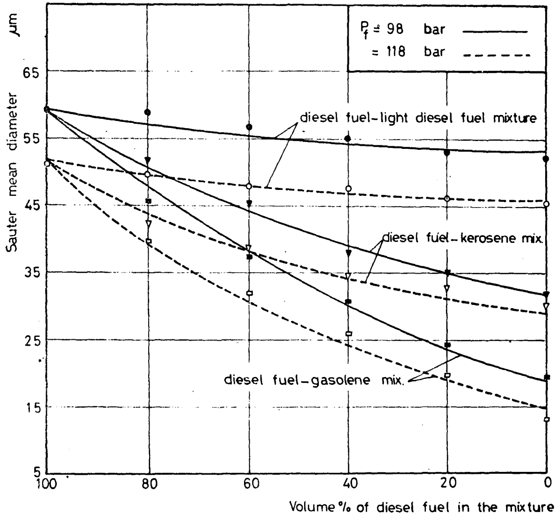
Fig(.28) Variation of Sauter mean diameter with the quantity of diesel fuel in multifuel at various injection pressures .
