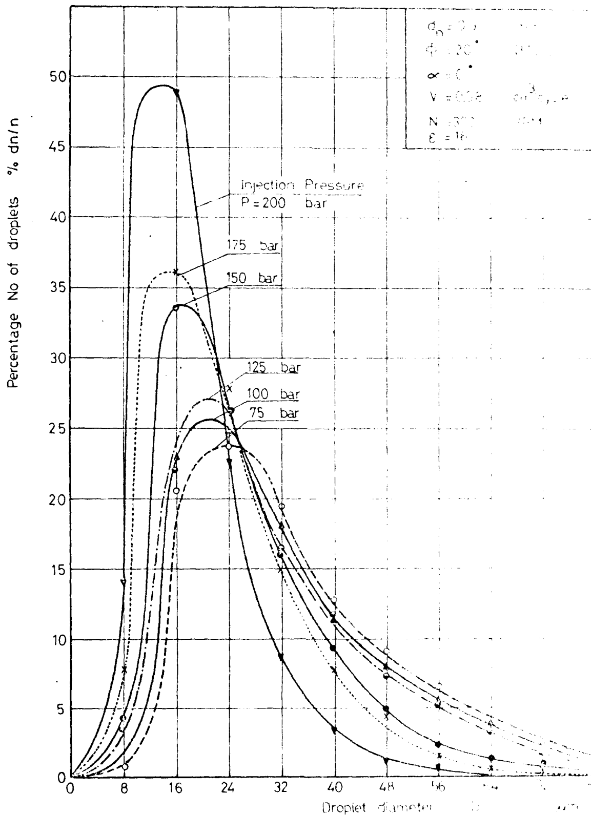
Fig(26) ) Droplet size distribution for engine fuel spray inside a cold engine model at various injection pressures
