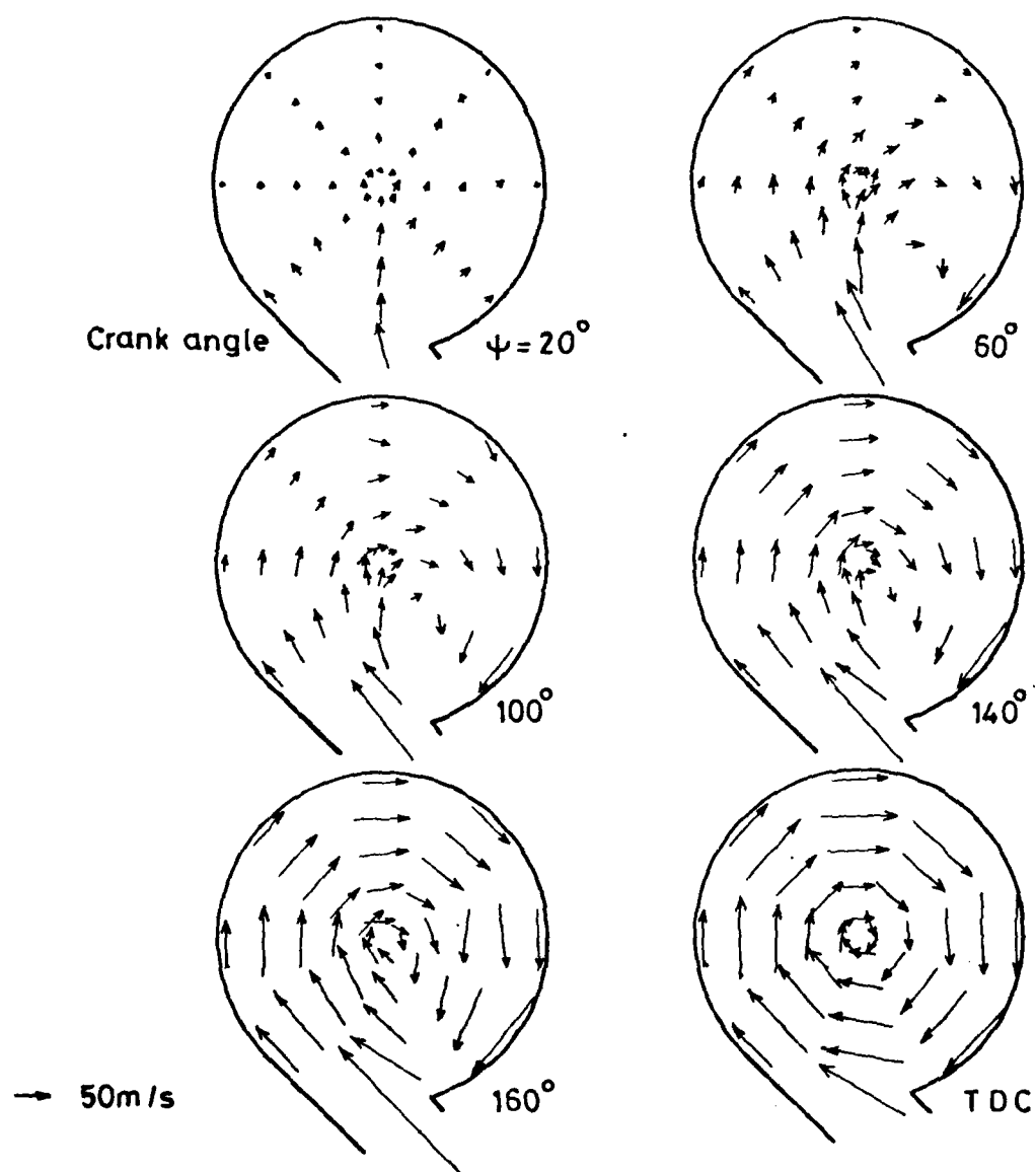
Fig (26) Velocity vector plot during compression stroke for V_s/V_c=0.772 , N=1000 \text{ r.p.m} and A_j/A = 0.0092
