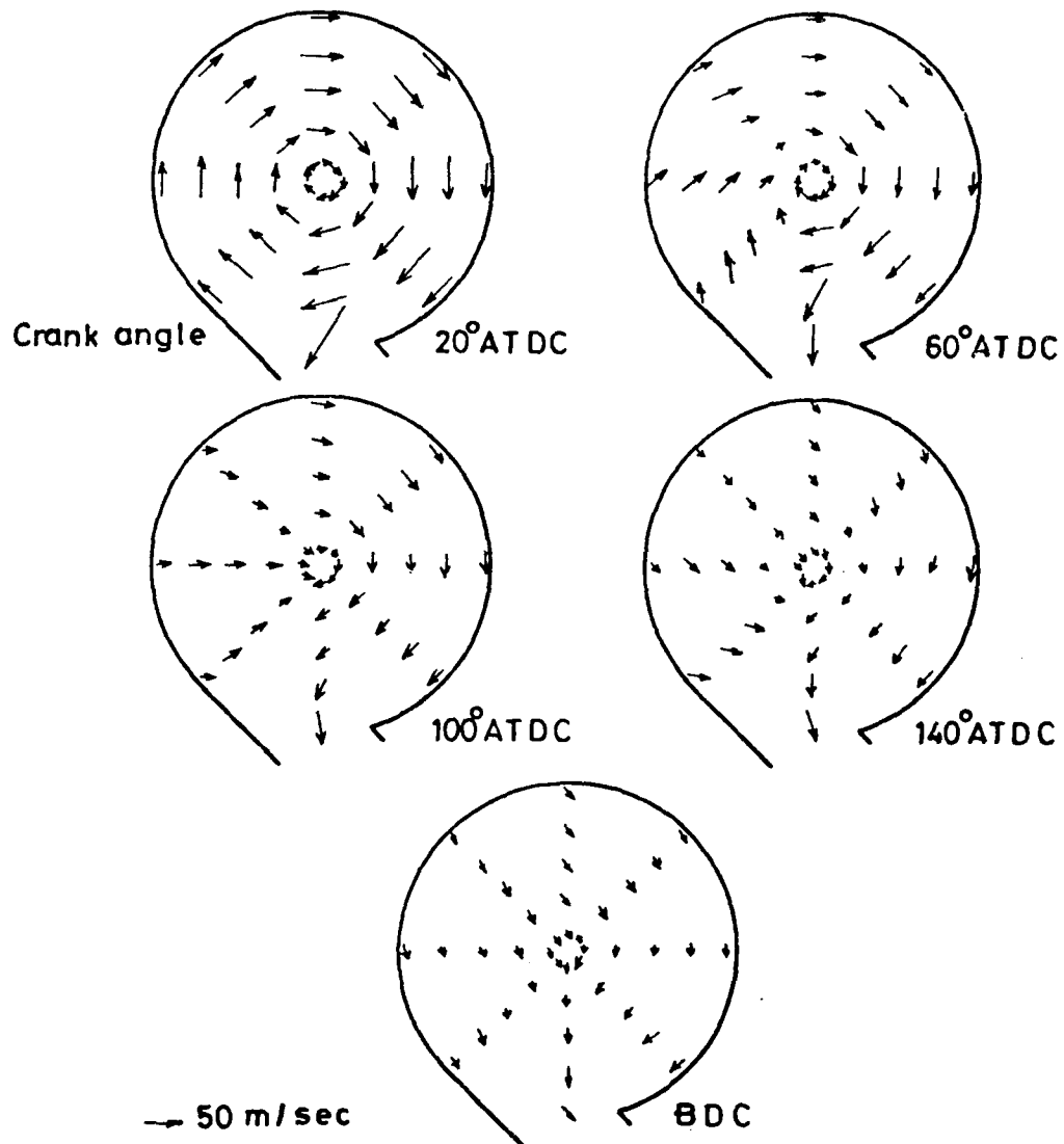
Fig( 27 ) Velocity vector plot during expansion stroke for V_s/V_c=0.772 , N=1000 r.p.m and A_j/A = 0.0092
