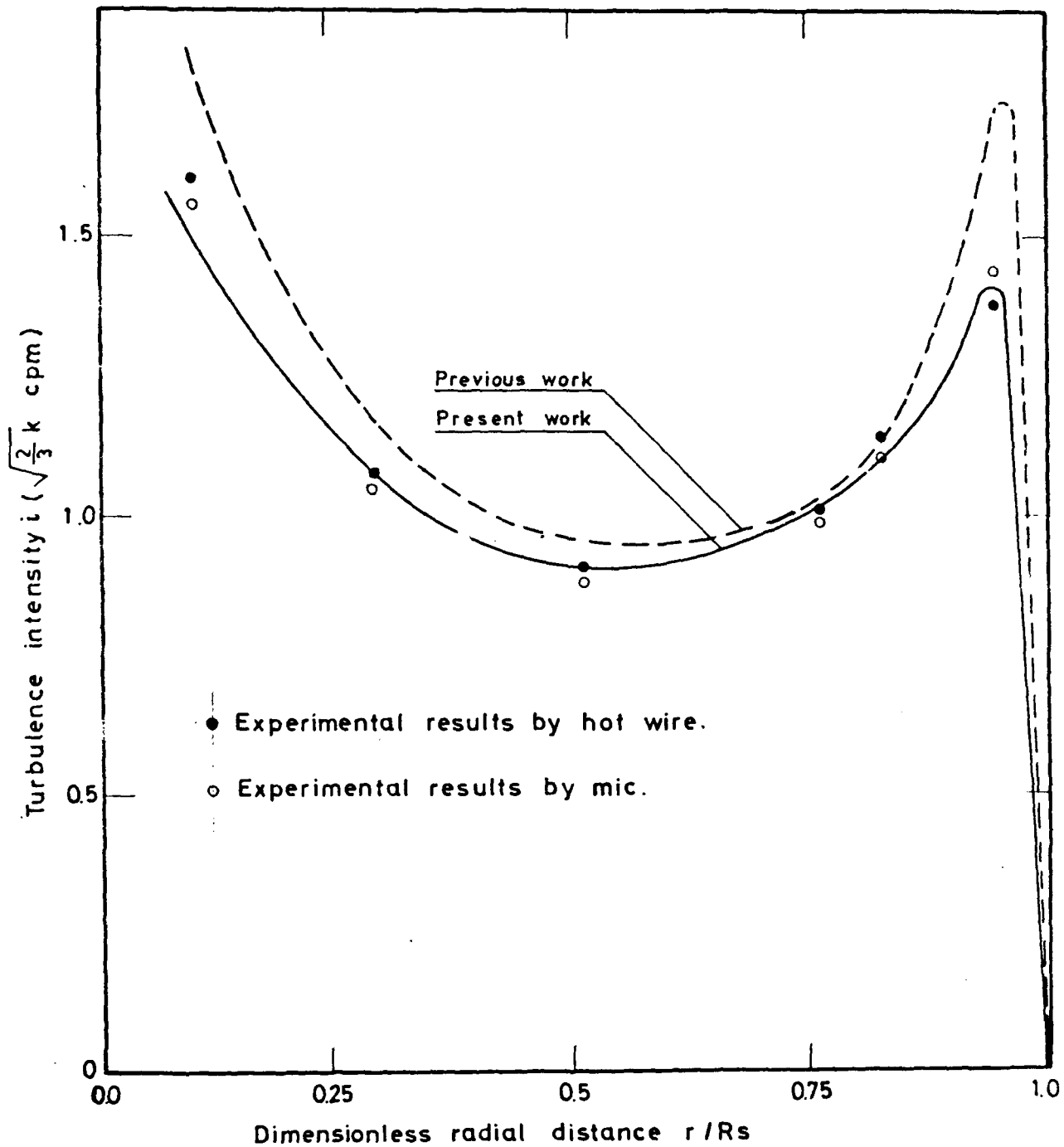
Fig. ( 21 ) Comparison of predicted turbulence intensity i / the suggested and previous method [ ] along the radius with the experimental results at TDC keeping V_s/V_c = 0.772 , A_j/A = 0.0092 and N = 1500 r. p. m. constant.
