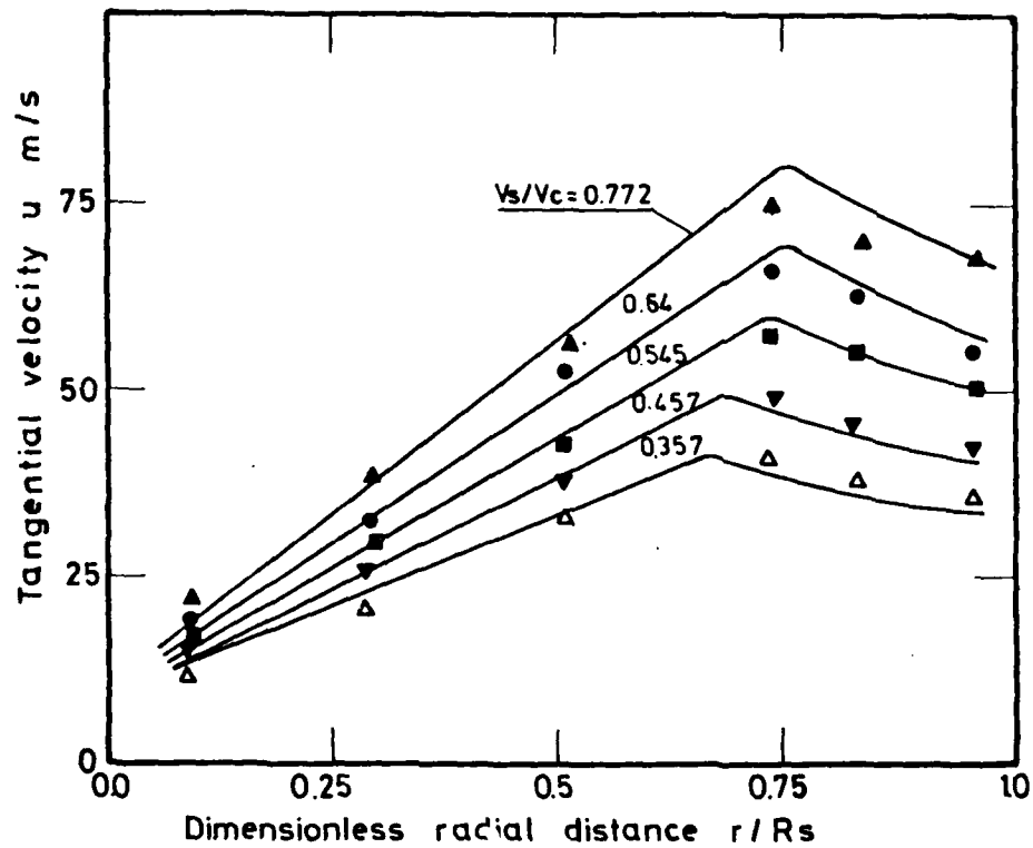
Fig.(45 )Predicted and measured tangential velocity in plane 4 and TDC for various radii and different swirl volume ratios keeping A_j/A_s = 0.0092 and N=1000 r.p.m. constant.
