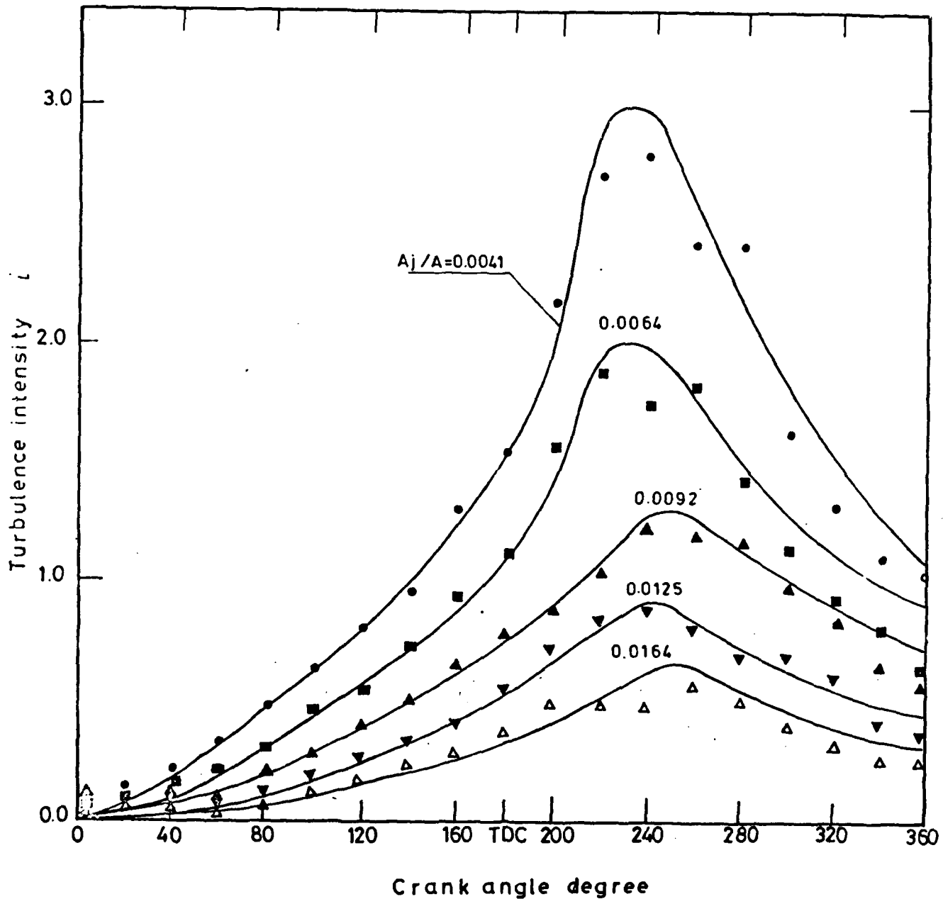
Fig ( 41 ) Predicted and measured turbulence intensity in plane 4 at r/R_s=0.503 during compression and expansion strokes for different port area ratio keeping V_s/V_c=0.772 and N=1000 r.p.m. constant.
