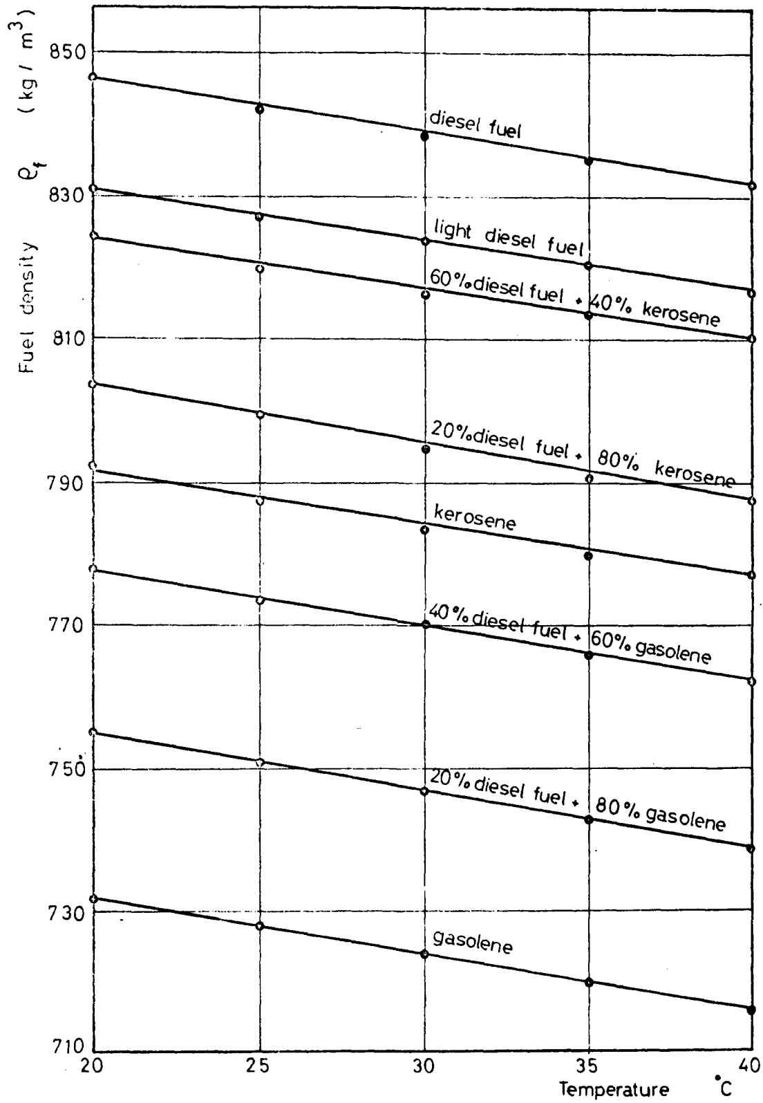
Fig( 21 ) Variation of fuel density with temperature rise for clear and multifuel .
