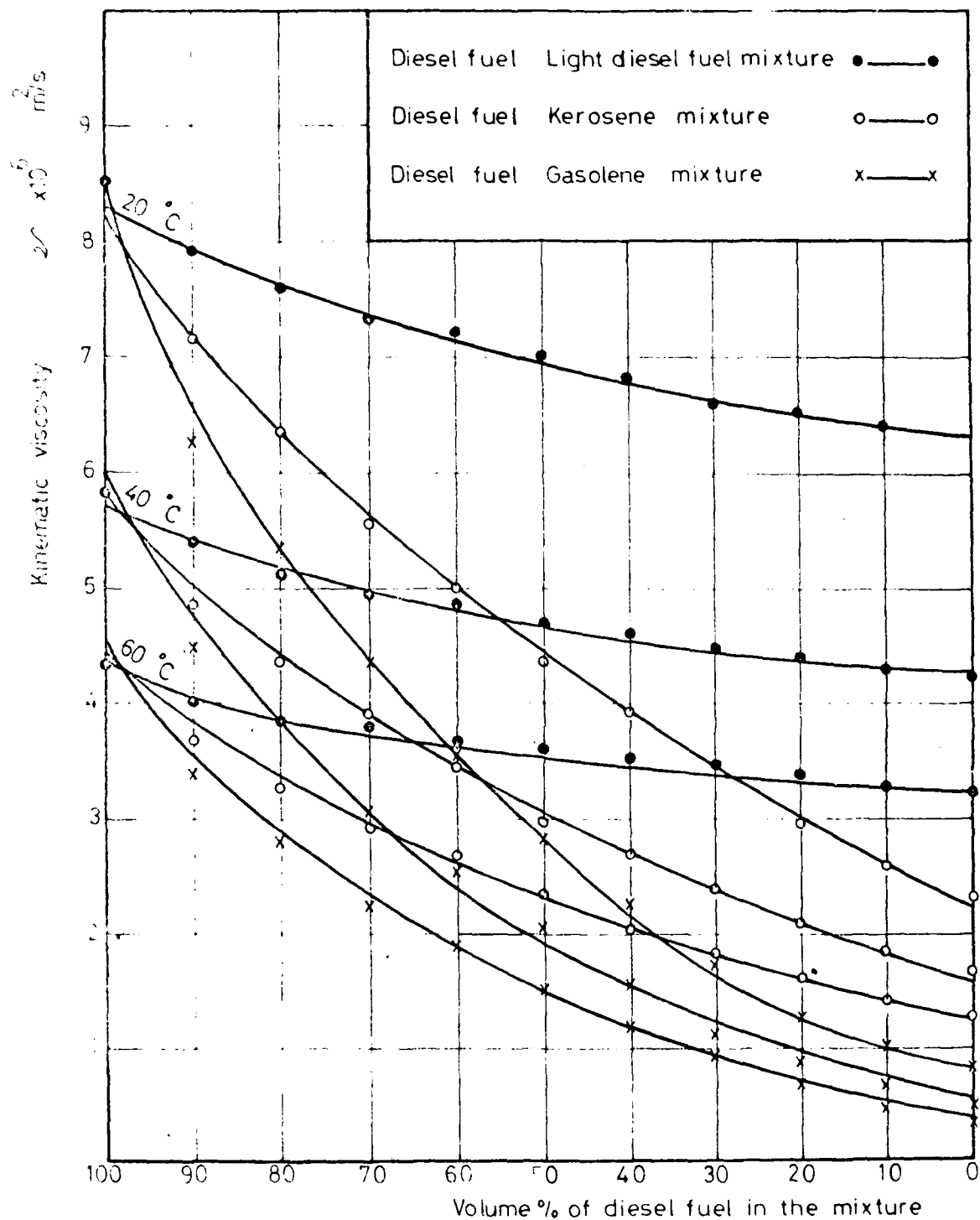
Fig(17) Nature of kinematic viscosity variation for various blend mixtures .
