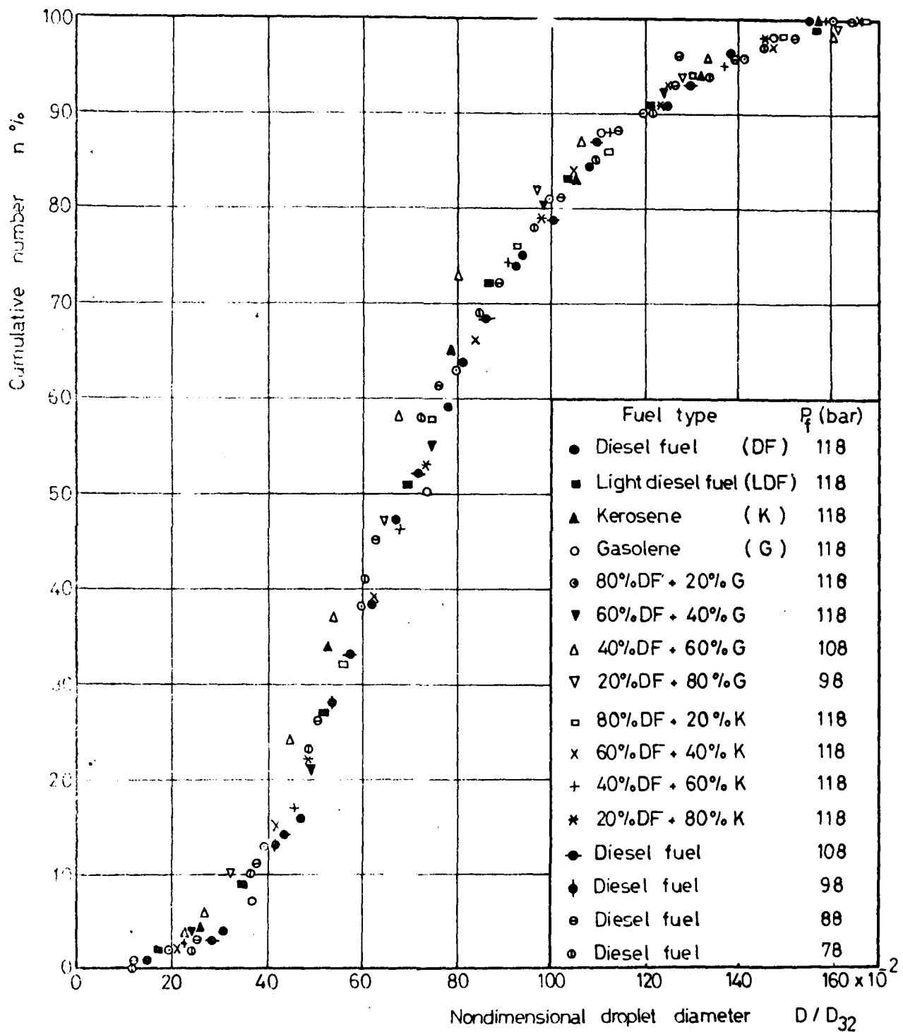
Fig( 32 ) Cumulative frequency distribution of droplet size for multifuel sprays with dimensionless droplet diameter .
