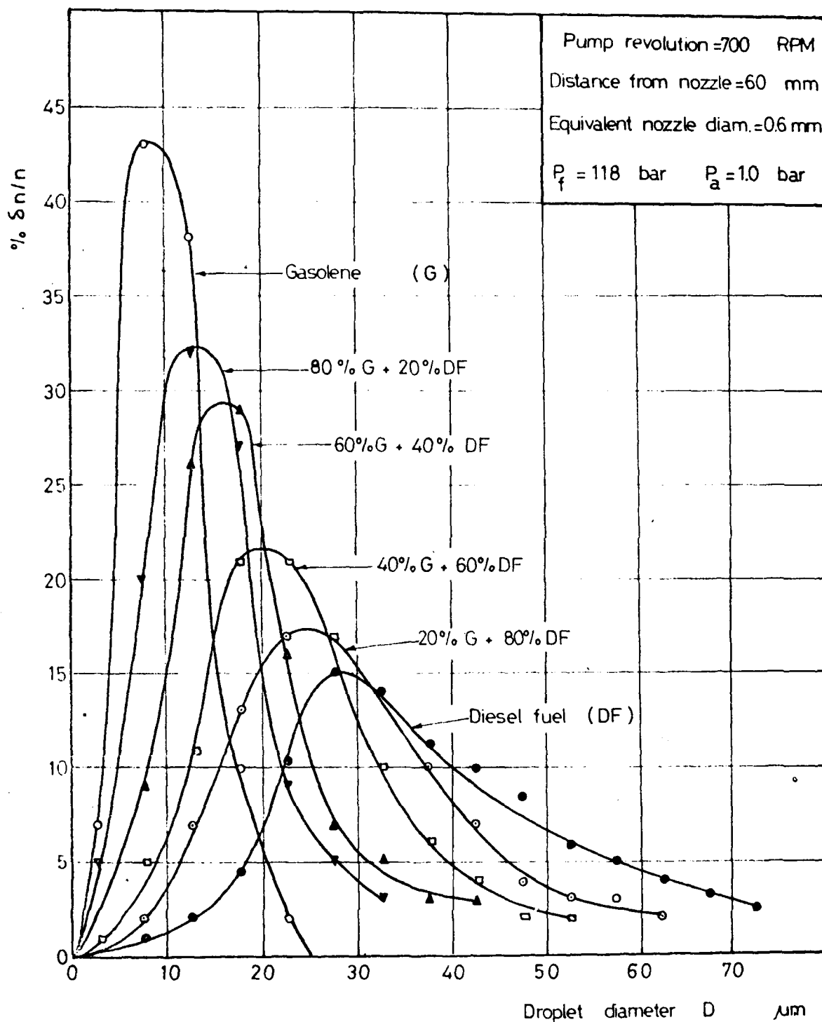
Fig(23) Droplet size distribution of diesel-gasolene mixtures .
