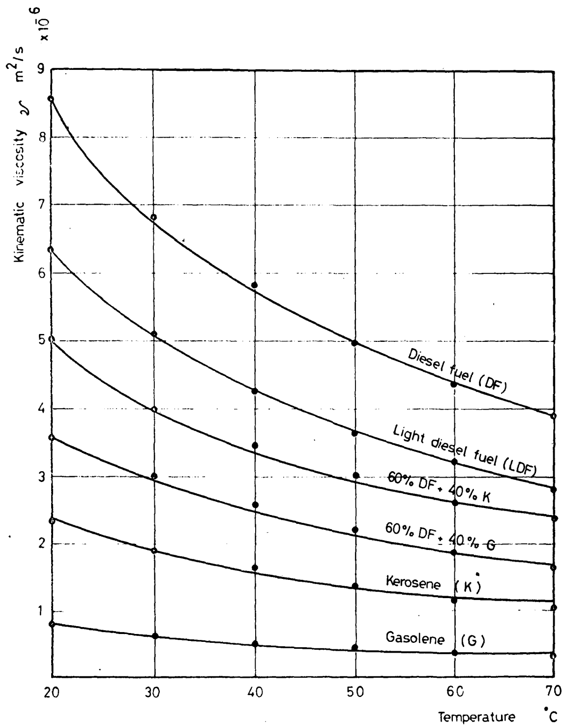
Fig ( 20 ) Variation of fuel viscosity with temperature rise for clear and multifuel .
