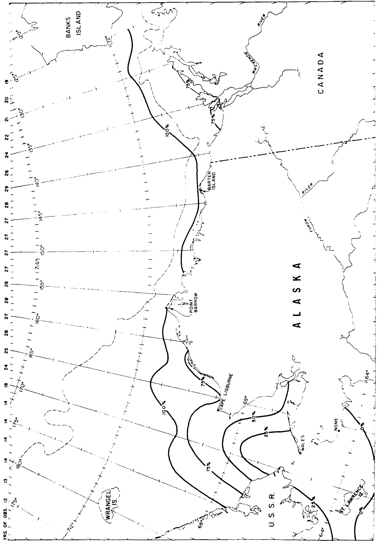
FIGURE 8. PROBABILITIES OF THE ICE LIMIT FOR JULY 1
