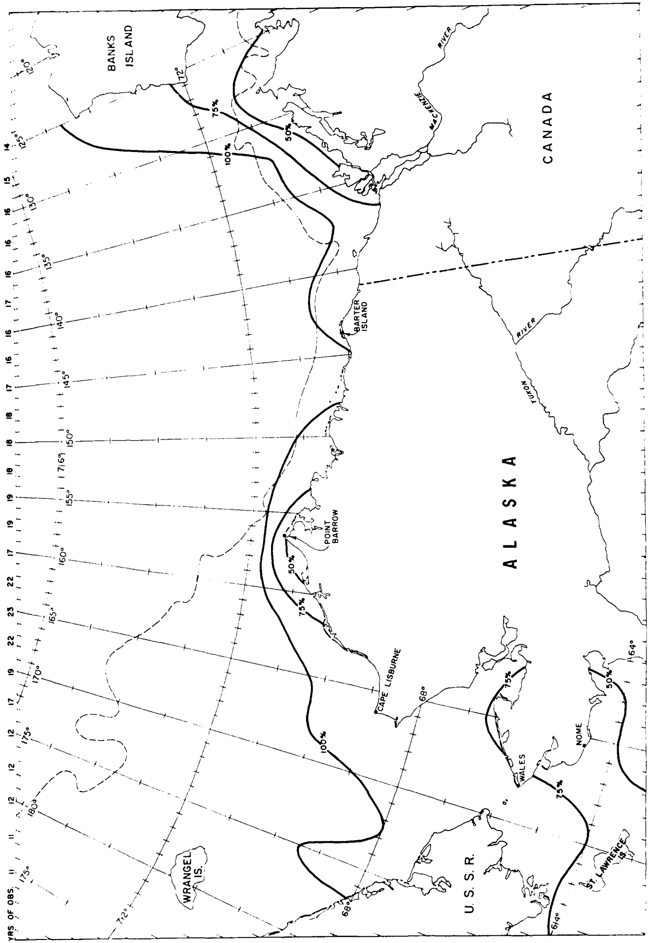
FIGURE 5. PROBABILITIES OF THE 50% ICE CONCENTRATION BOUNDARY FOR JUNE 1
