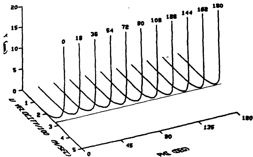
Figure 8a. 3-D velocity profiles, M = 0.96 , \alpha = 2.0^\circ , X/D = 4.76
