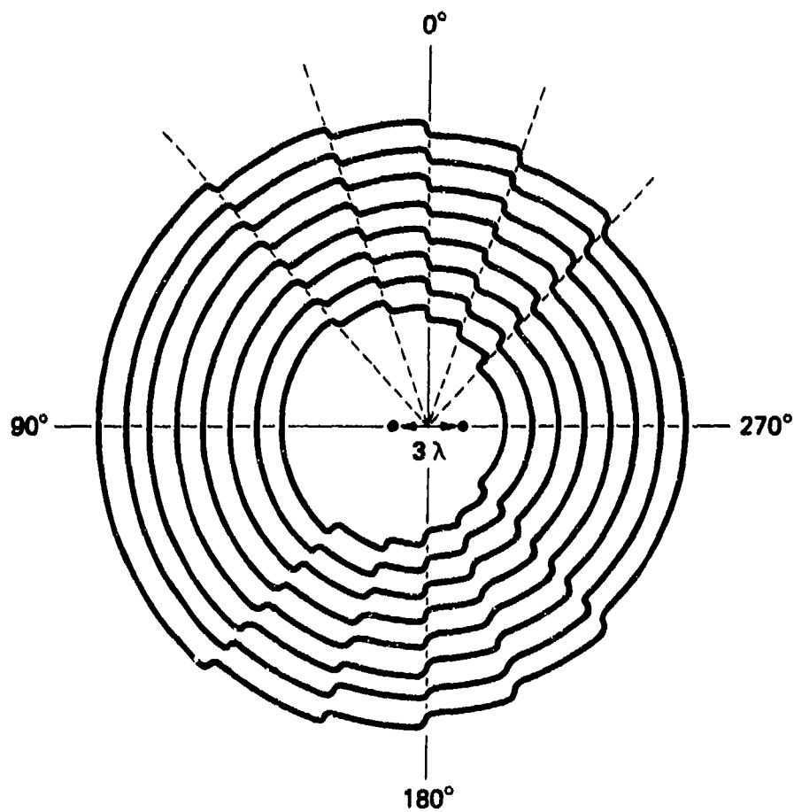
FIGURE A.1 DISTORTED PHASE FRONTS FROM TWO WAVE CENTERS SEPARATED BY THREE WAVELENGTHS AND DRIVEN 180° OUT OF PHASE
