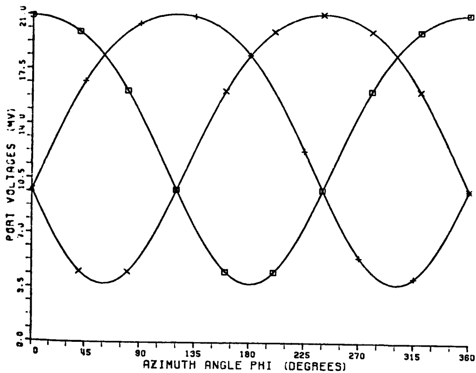
Fig. 4-2(a). Theta component of the received voltage pattern for three input ports spaced 120^\circ apart around the cylinder.
