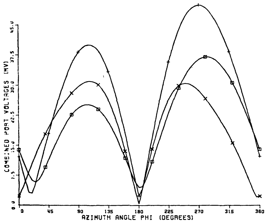
Fig. 4-11(b). Phi component of received voltage pattern obtained by adding voltage at Port 1 and Port 2. Three frequencies are shown. The incident wave is 20^\circ above horizontal plane. The half-loop elements are on the infinite cylinder.
