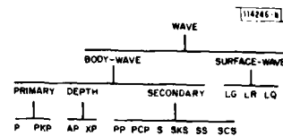
Fig. II-16. Inheritance hierarchy of frames representing seismic waves.
