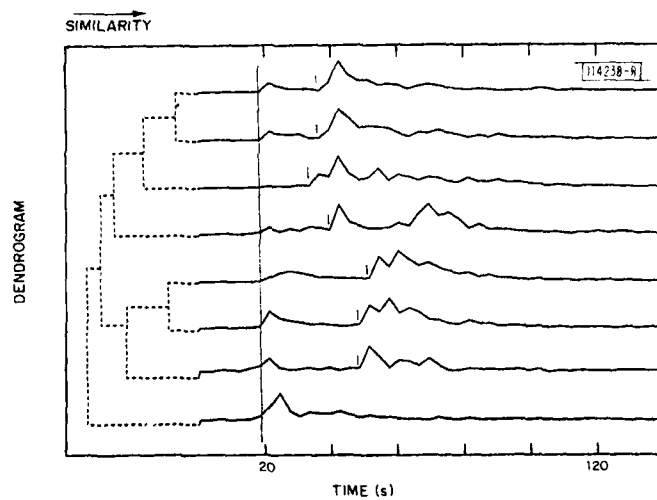
Fig. II-8. Cluster analysis of envelopes of eight local seismograms recorded at BDW. A dendrogram indicating hierarchical clustering of waveforms is shown by dotted lines to left of envelopes.
