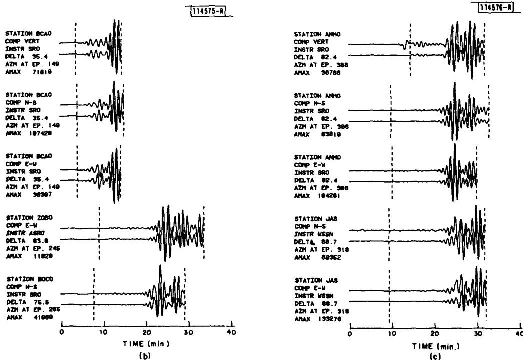
Fig. III-6(a-c). Comparison of observed (top) and synthetic GDSN seismograms for El Asnam, Algeria earthquake of 10 October 1980.
