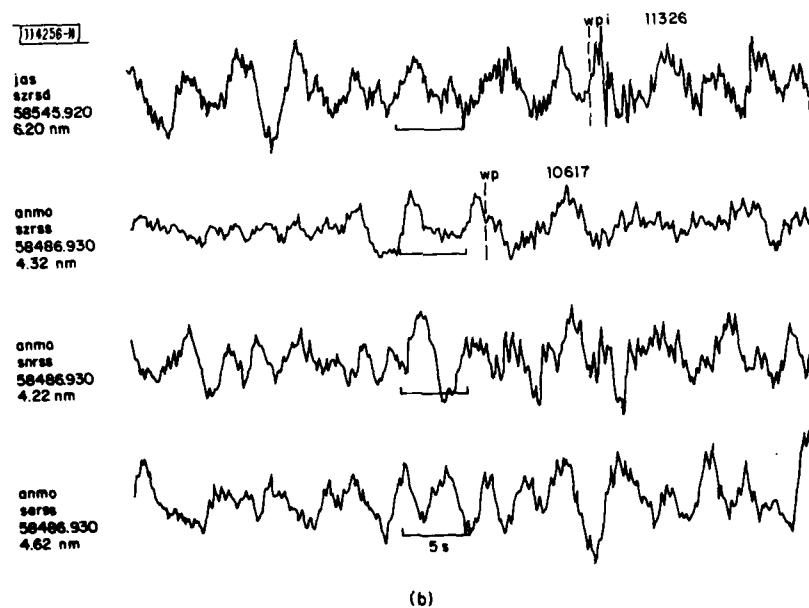
Fig. II-22(a-b). Hypothetical Colorado event.
