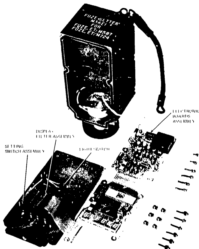
Figure 9. Electronics removed.
