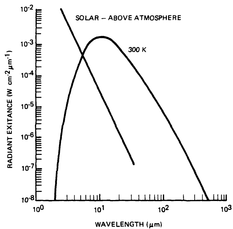
Figure III-1. Radiance for 300 0 K Blackbody and Reflected Sunlight
