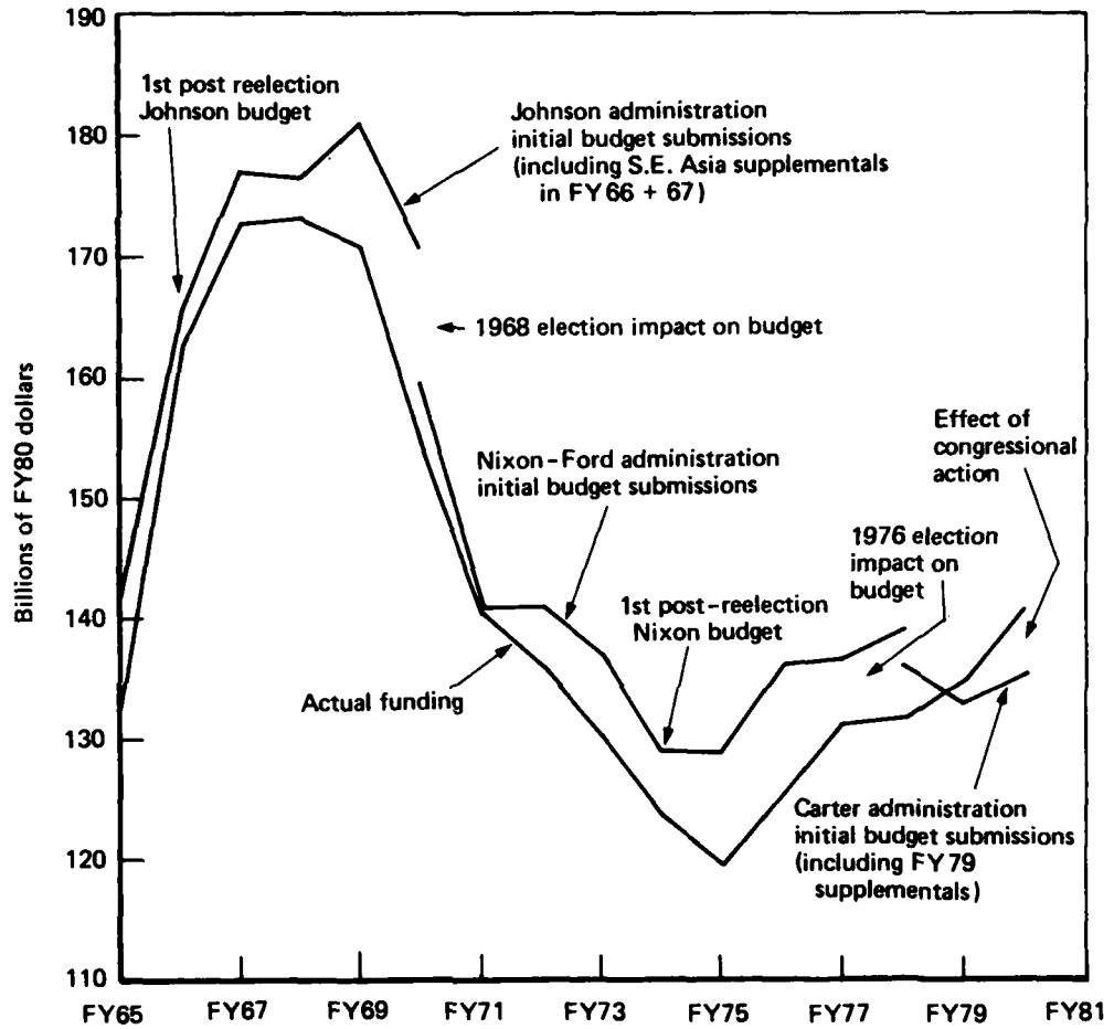
Fig. 3 - Defense TOA
