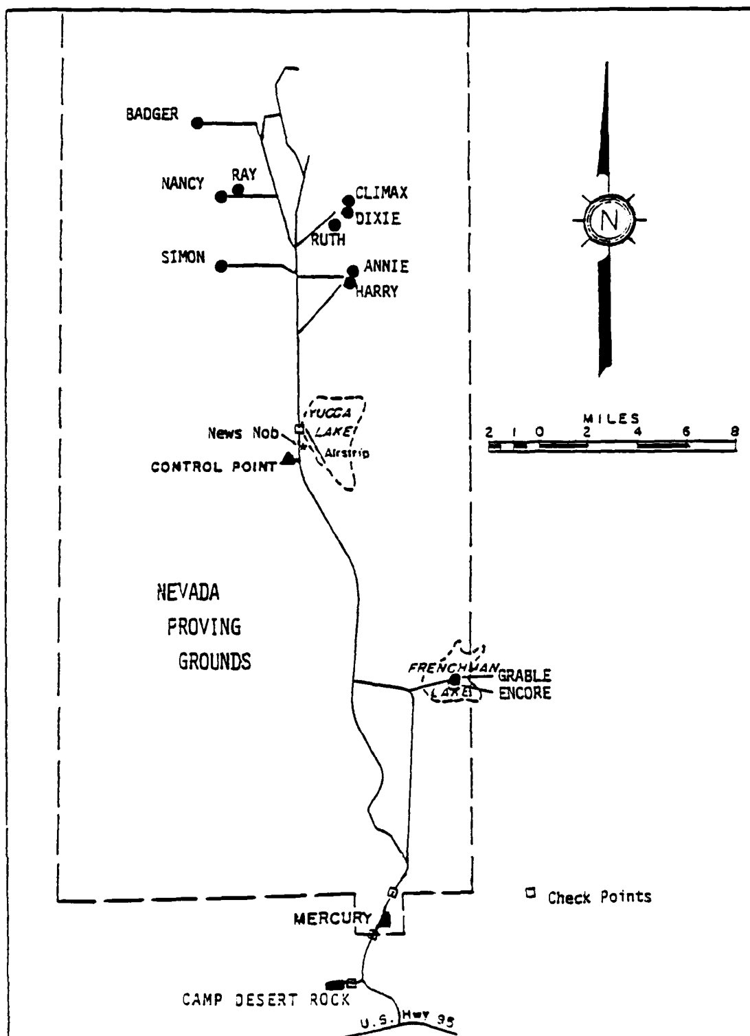
Figure 1-1 Shot Locations, Operation Upshot-Knothole
