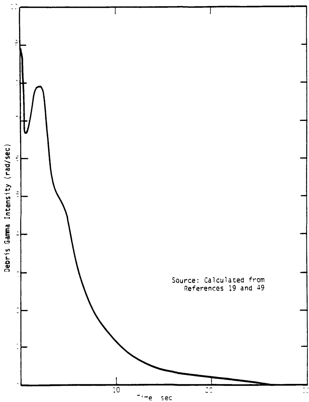
Figure 3-1 Debris Gamma Intensity at 2000 Yards as a Function of Time, Shot Badger
