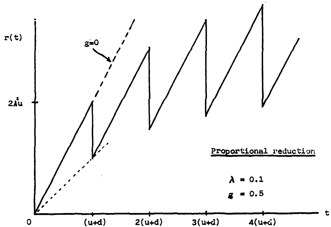
Fig. 4.4.1 Linear failure rate for fixed and proportional reduction.
