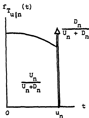
Fig. 2.6.3 P.d.f. of T_{u|n} .
