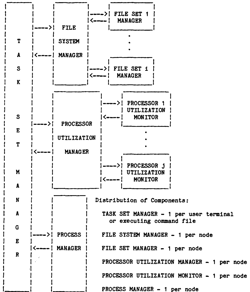
Figure 1. The XFDPS.1 Model of Control
