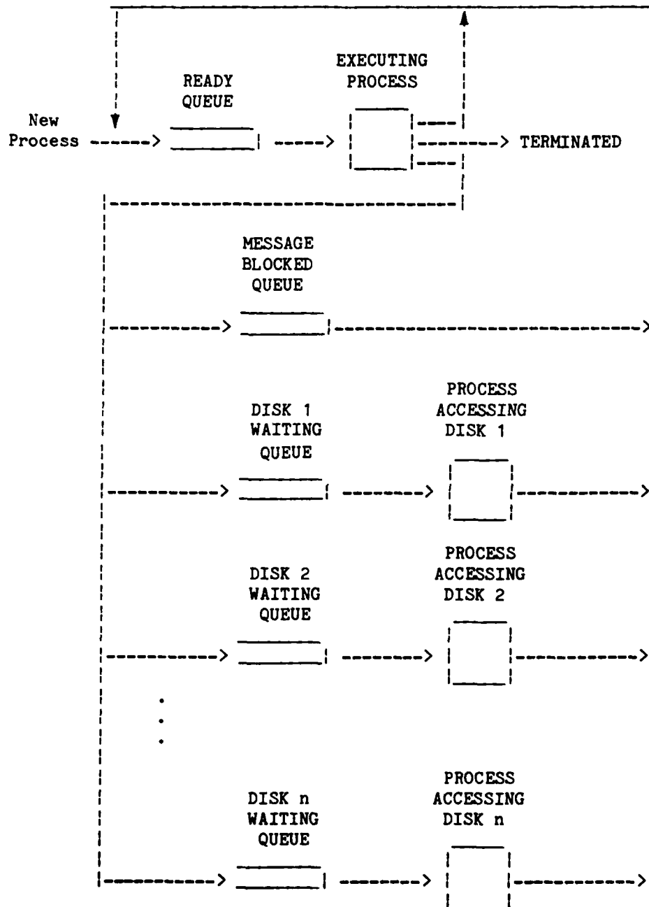
Figure 3. Process Queues on Each Node
