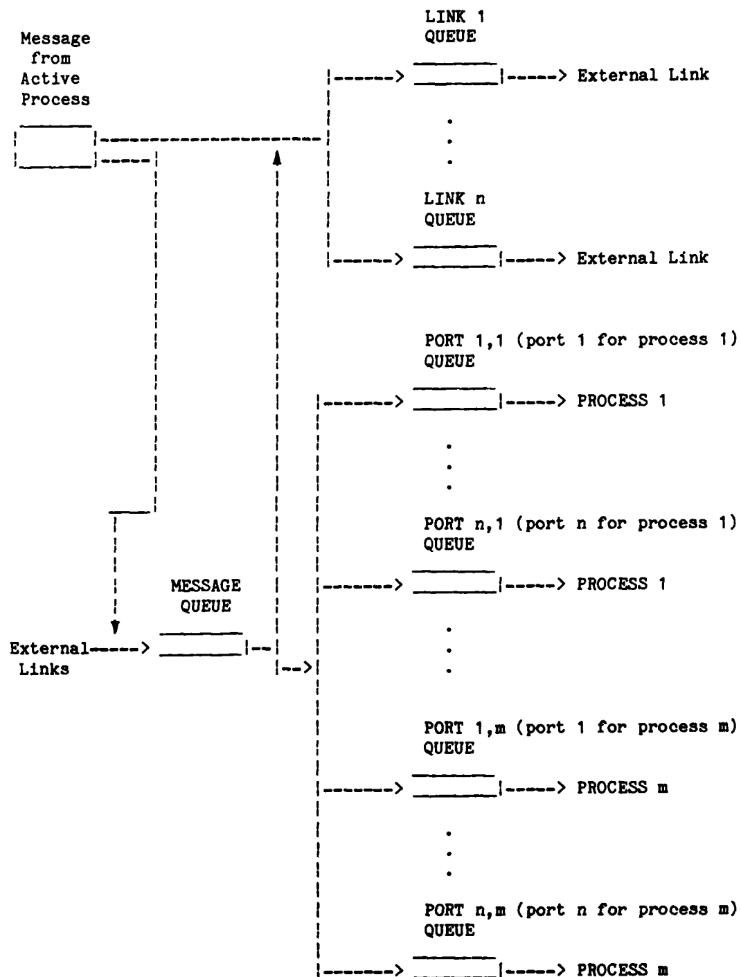
Figure 4. Message QUEUES on Each Node
