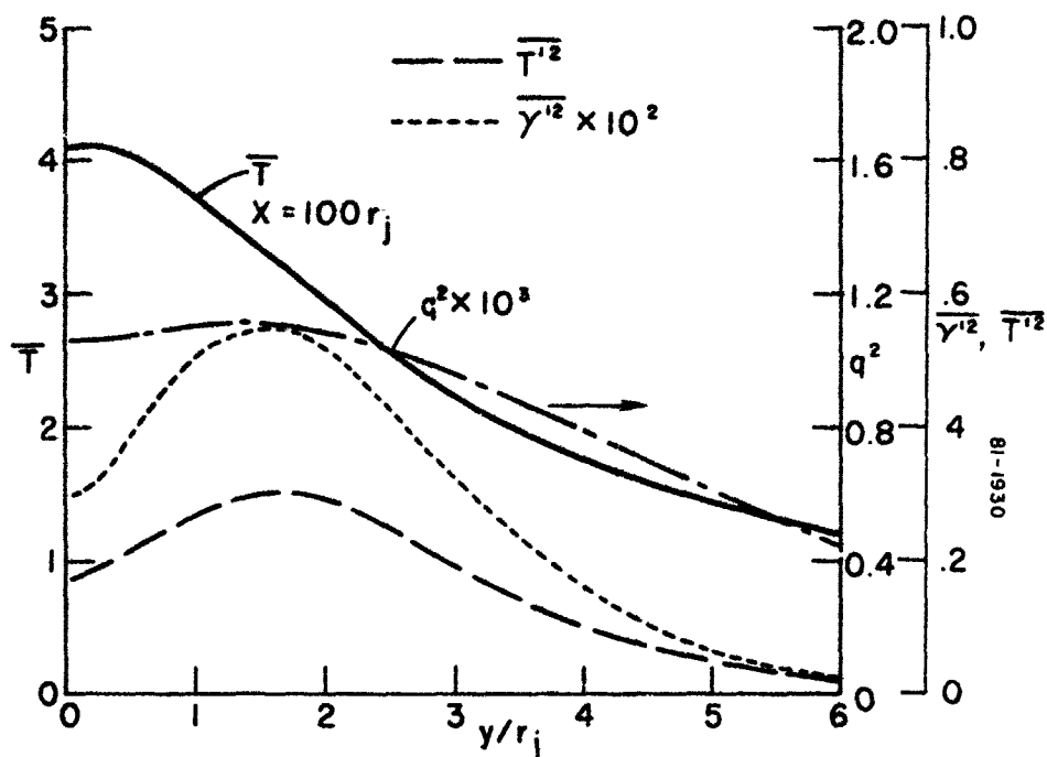
FIGURE 11. Radial Distribution of Mean and Fluctuating Properties Predicted by RSL Code for the Model Afterburning Exhaust Plume at x/r_j = 100 . Temperature and Velocity Normalized by Reference Values of 300 K and 2500 m/sec, Respectively.
