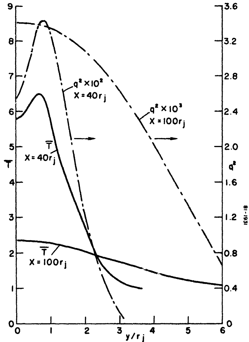
FIGURE 13. Radial Profile of Mean and Fluctuating Properties Predicted by the BOAT Code with a Compressibility Correction for the Model Afterburning Exhaust Plume at x/r_j = 40 and 100 . Temperature and Velocity Normalized by Reference Values of 300\text{ K} and 2500\text{ m/sec} , Respectively.
