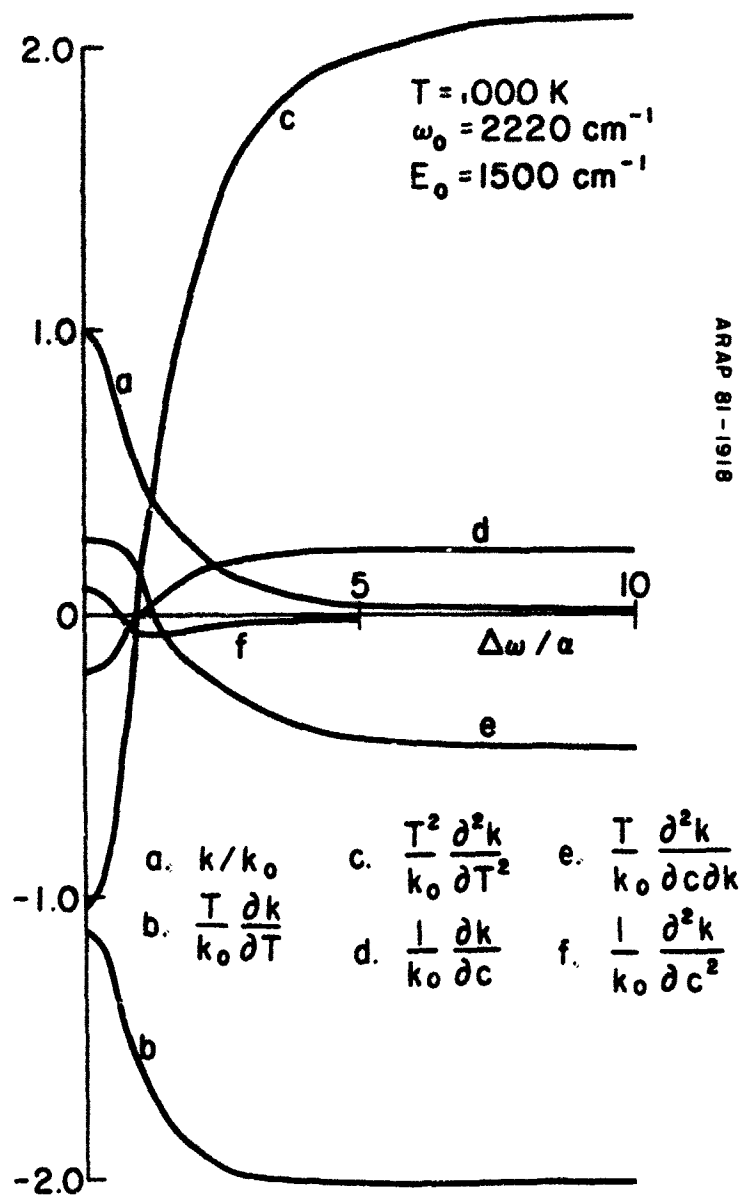
FIGURE B-2. Normalized Derivatives of the Spectral Absorption Coefficient: Single Line, Lorentz Line Shape, E_0 = 1500 \text{ cm}^{-1} , T = 1000 \text{ K} .
