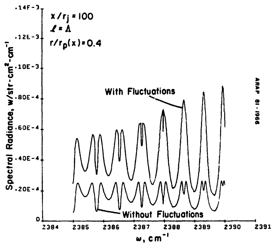
FIGURE 32. Source Spectral Radiance for a Line of Sight at the Axial Location x/r_j = 100 and Off the Plume Axis at r = 0.4r_p . CO 2 Blue Spike Region.
