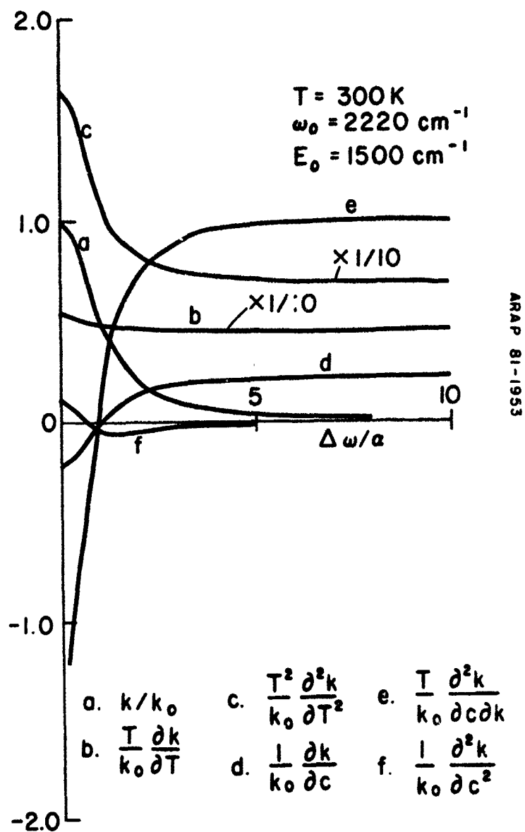
FIGURE B-1. Normalized Derivatives of the Spectral Absorption Coefficient: Single Line, Lorentz Line Shape, E_0 = 1500 \text{ cm}^{-1} , T = 300 \text{ K} .
