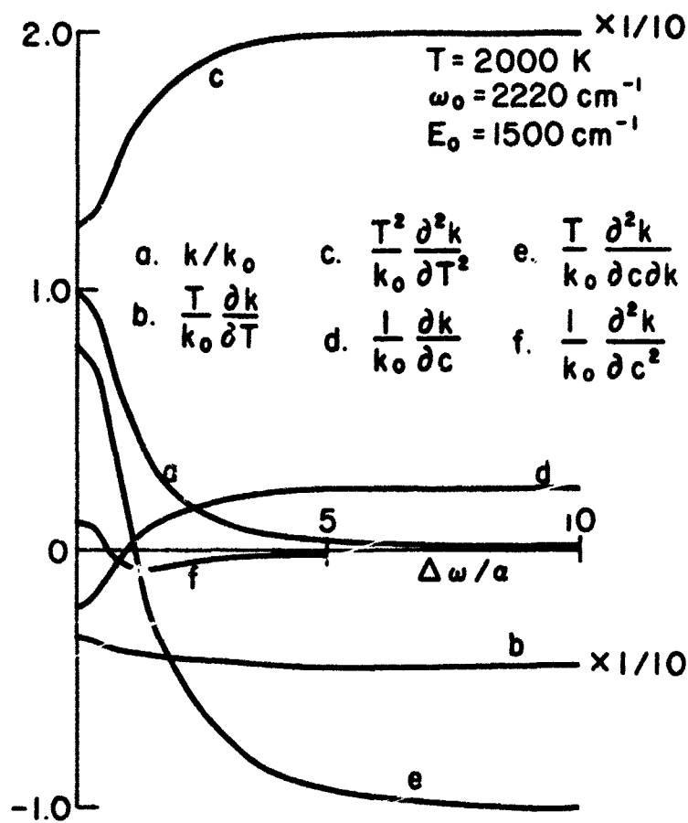
FIGURE B-3. Normalized Derivatives of the Spectral Absorption Coefficient: Single Line, Lorentz Line Shape, E_0 = 1500 \text{ cm}^{-1} , T = 2000 \text{ K} .
