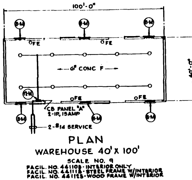
Figure B6. Existing warehouse (facility number: 44-11).
