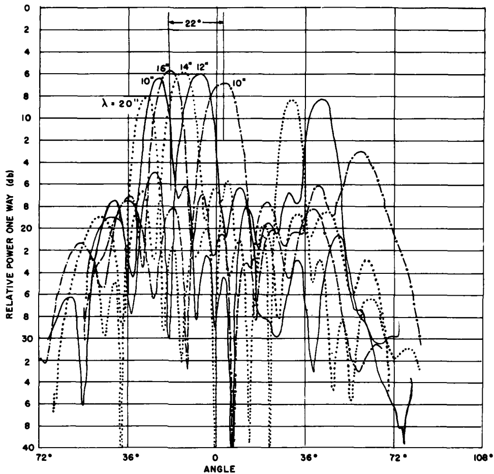
Figure 12. E-plane Radiation Patterns of Eight-Element Array Showing the Amount of Scanning in Degrees When You Vary the Dipole Spacing from \lambda/2 to \lambda . This is with the 180^\circ Phase Reversal in the Dipoles.
