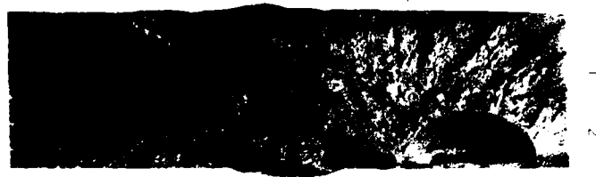
Figure 19-1 Fracture Surfaces of As-Welded SMA Tee Weldments Tested at Intermediate Strain Rate at -60 F (-51°C) - 1X Magnification
