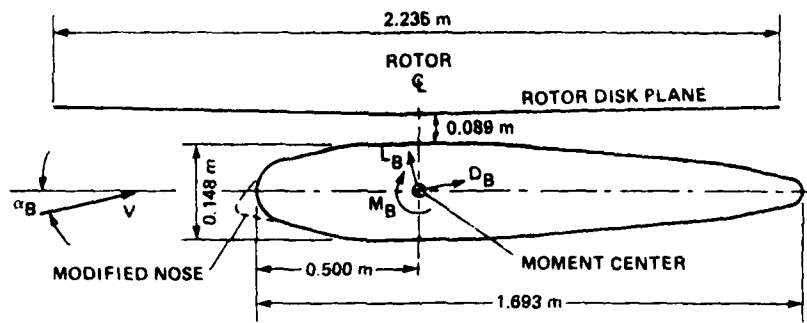
Figure 1. 1/6 Scale RTA body of revolution shown with rotor in baseline position.
