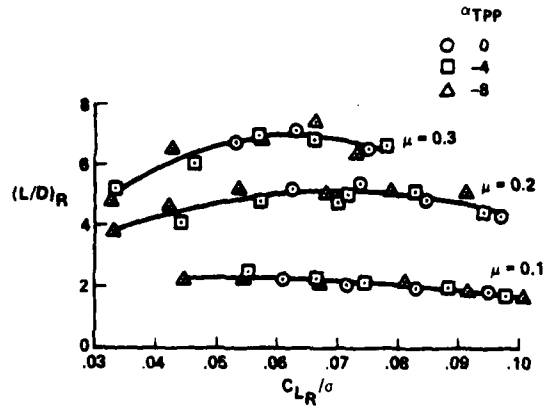
Figure 4. Isolated rotor performance.
