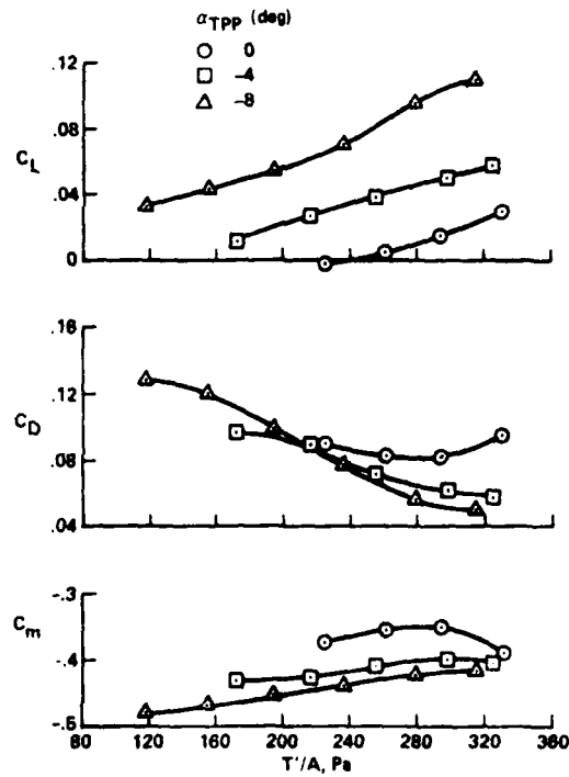
Figure 11. Effect of rotor thrust on body longitudinal characteristics (baseline configuration).
