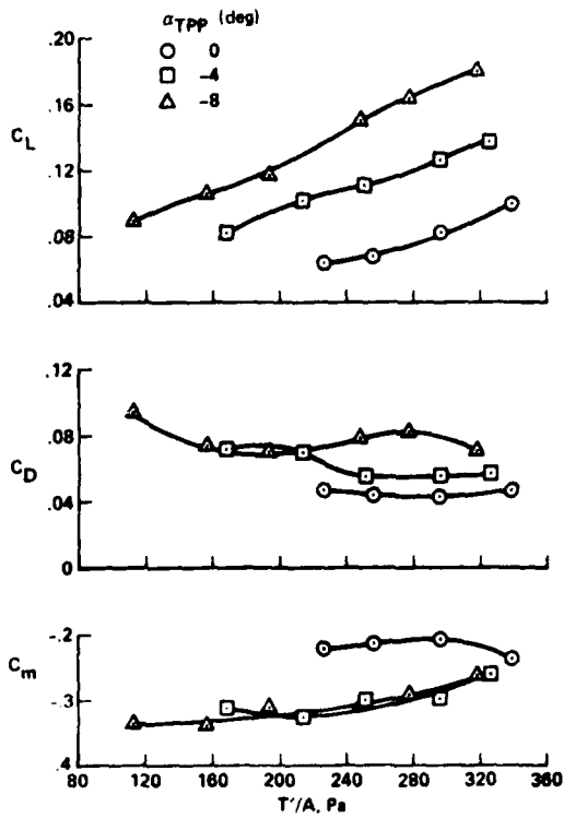
Figure 11. Effect of rotor thrust on body longitudinal characteristics (baseline configuration).
